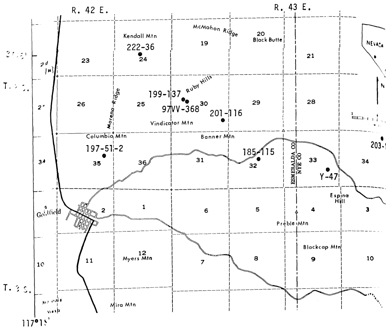
Figure 1. Map showing location of dated samples.
