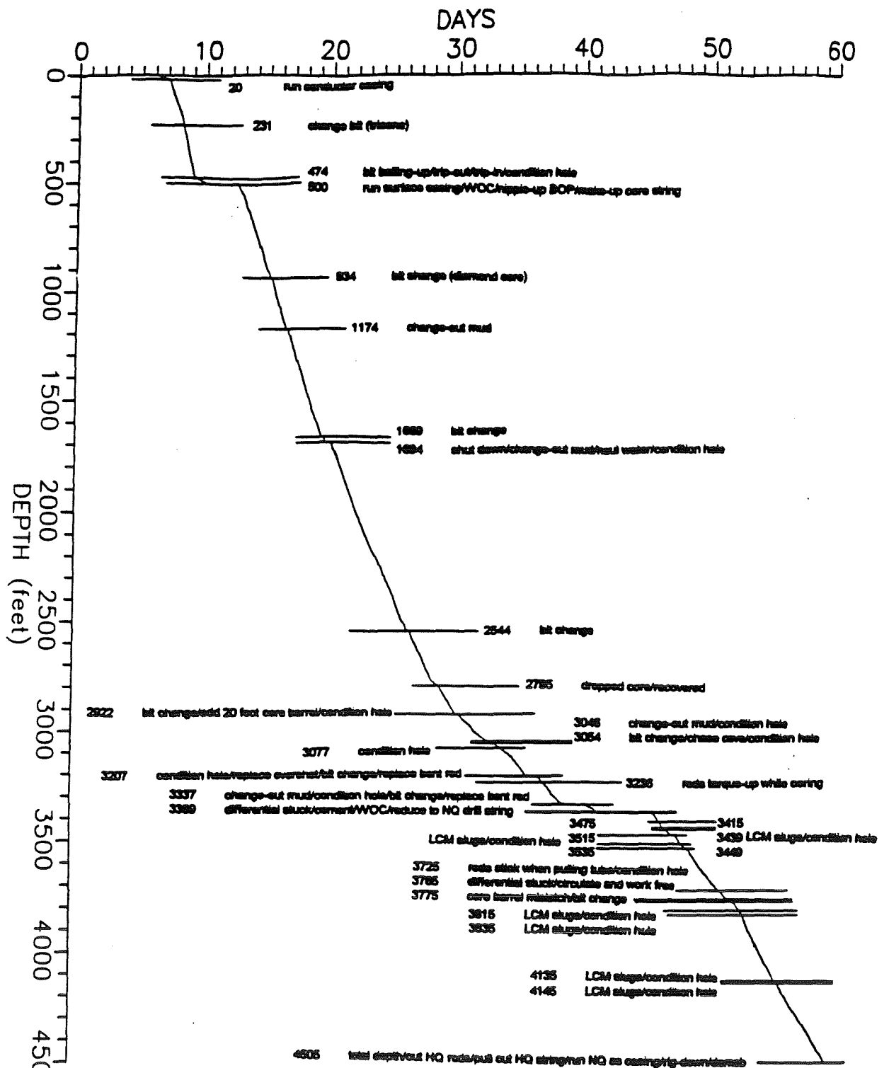
Figure 4. Drilling history of the Alpine 1/Federal borehole.
