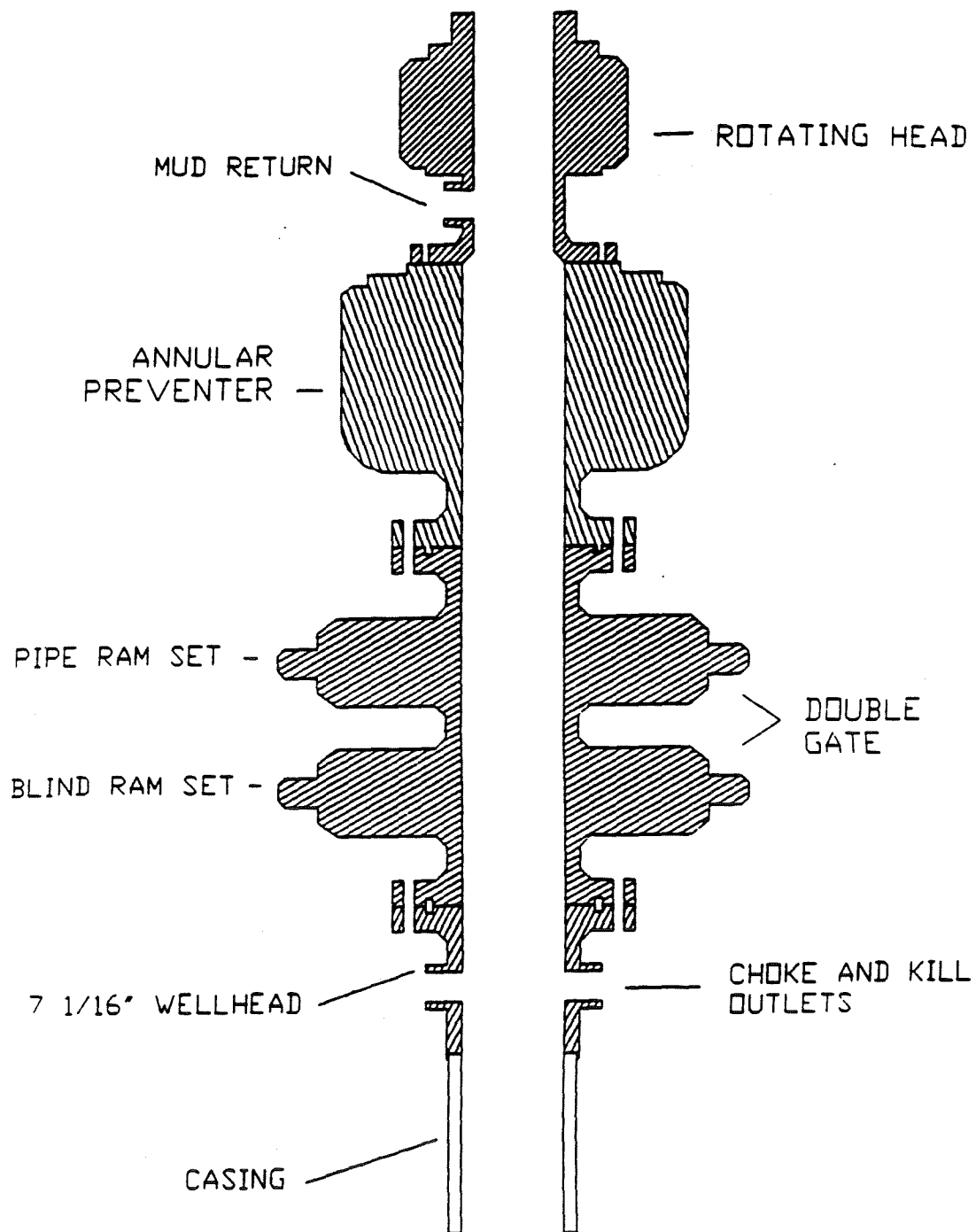
Figure 3. Diagram of blow out prevention (BOP) equipment for the Alpine 1/Federal borehole.
