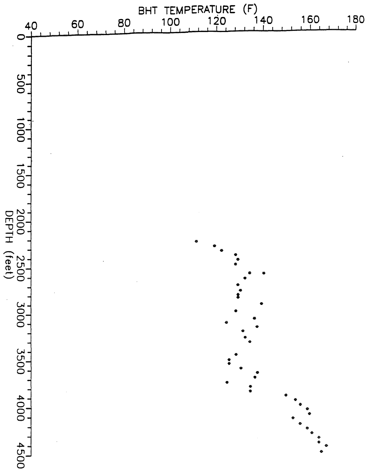
Figure 10. Subsurface bottom-hole mud temperature (BHT) versus drilling depth.
