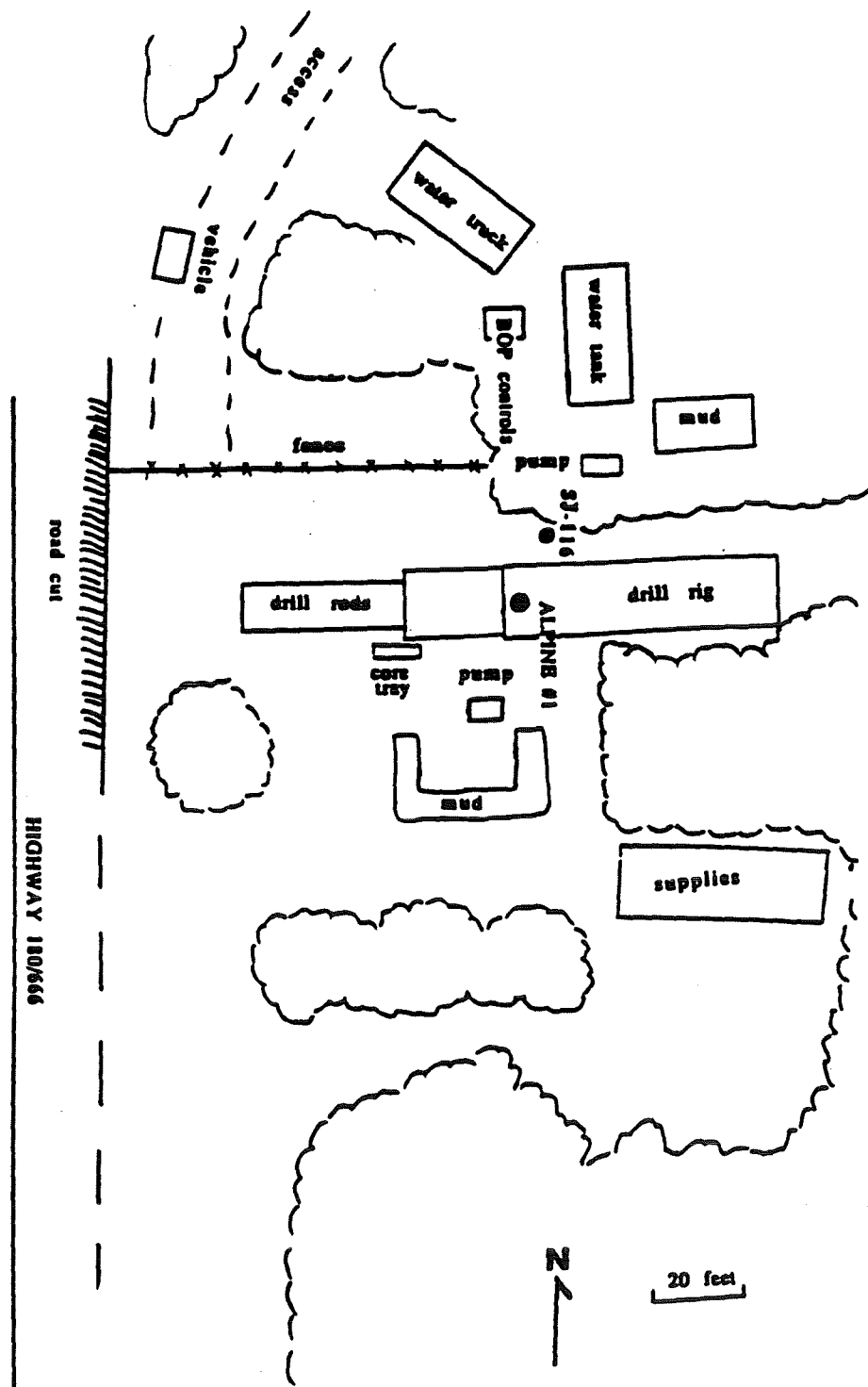
Figure 2. Layout of the Alpine 1/Federal drill site.
