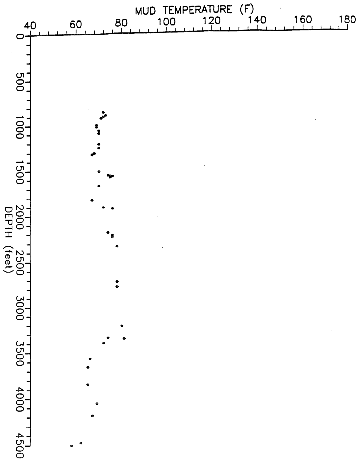
Figure 9. Surface mud temperature versus drilling depth.
