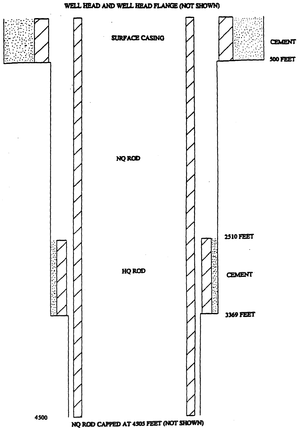
Figure 11. Temporary observation well completion diagram.
