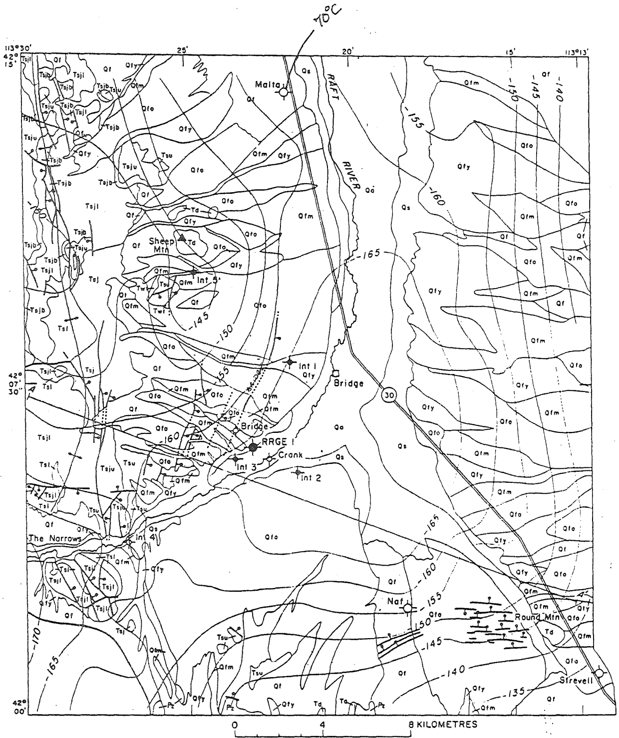
Figure 2. Geologic and gravitational features of the southern Raft River valley. Left , area map showing Bouguer gravity units in the area map and the cross section and a key to
