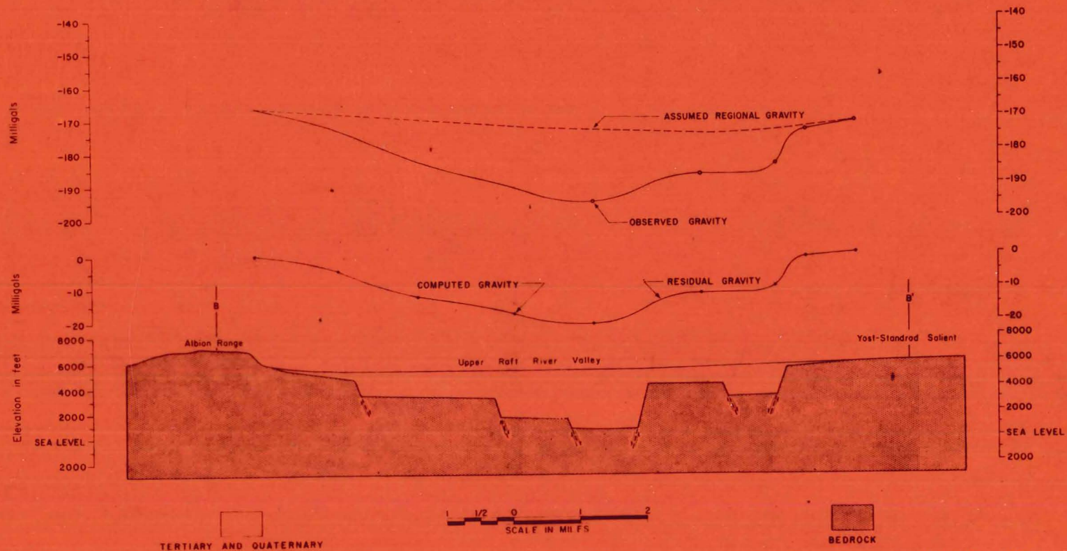
Gravity and interpretive geologic cross section along profile B-B' across Upper Raft River valley graben and northwestern part of Raft River Mountains. Assumed density contrast is 0.5 g/cc.
