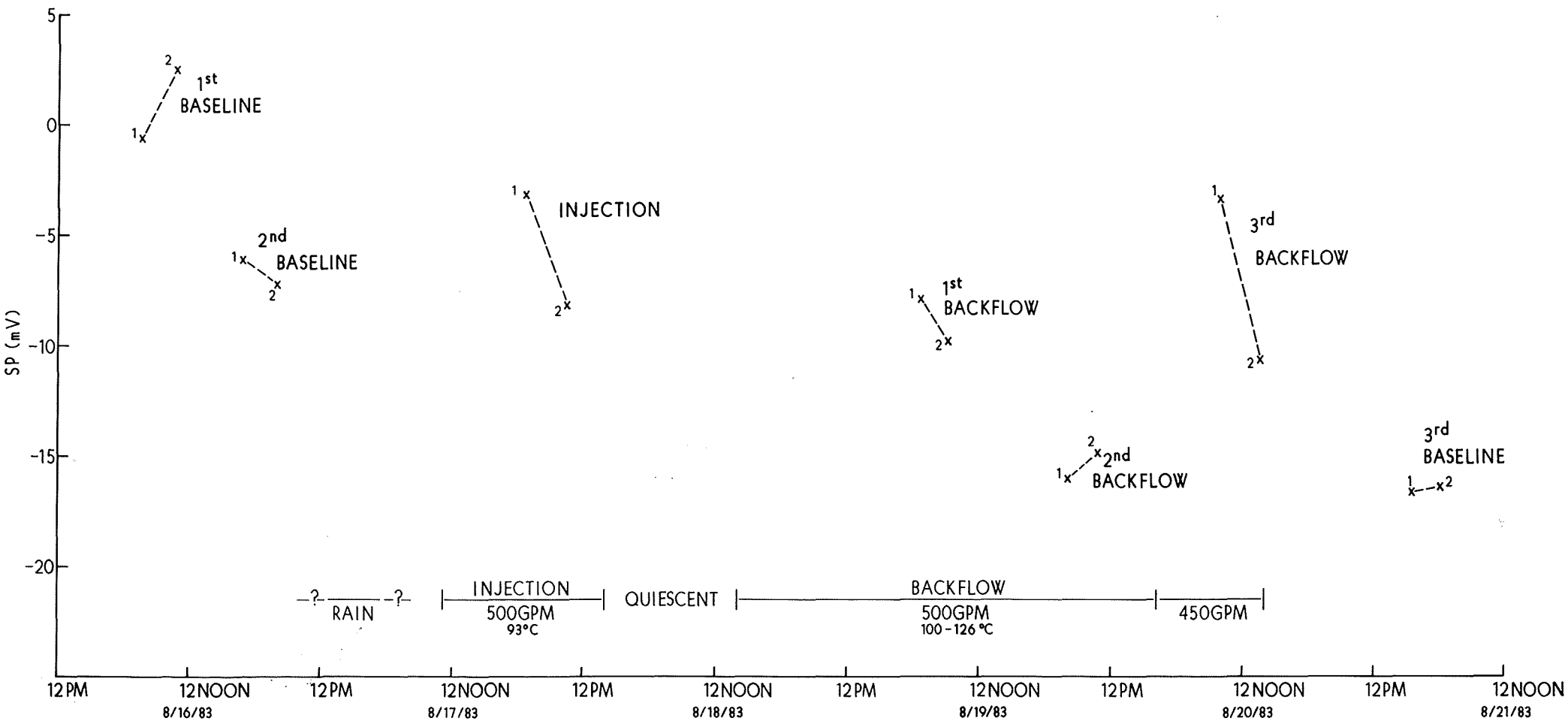
FIGURE 3 SELF - POTENTIAL SURVEY BASE READINGS EAST MESA, IMPERIAL COUNTY, CALIFORNIA
