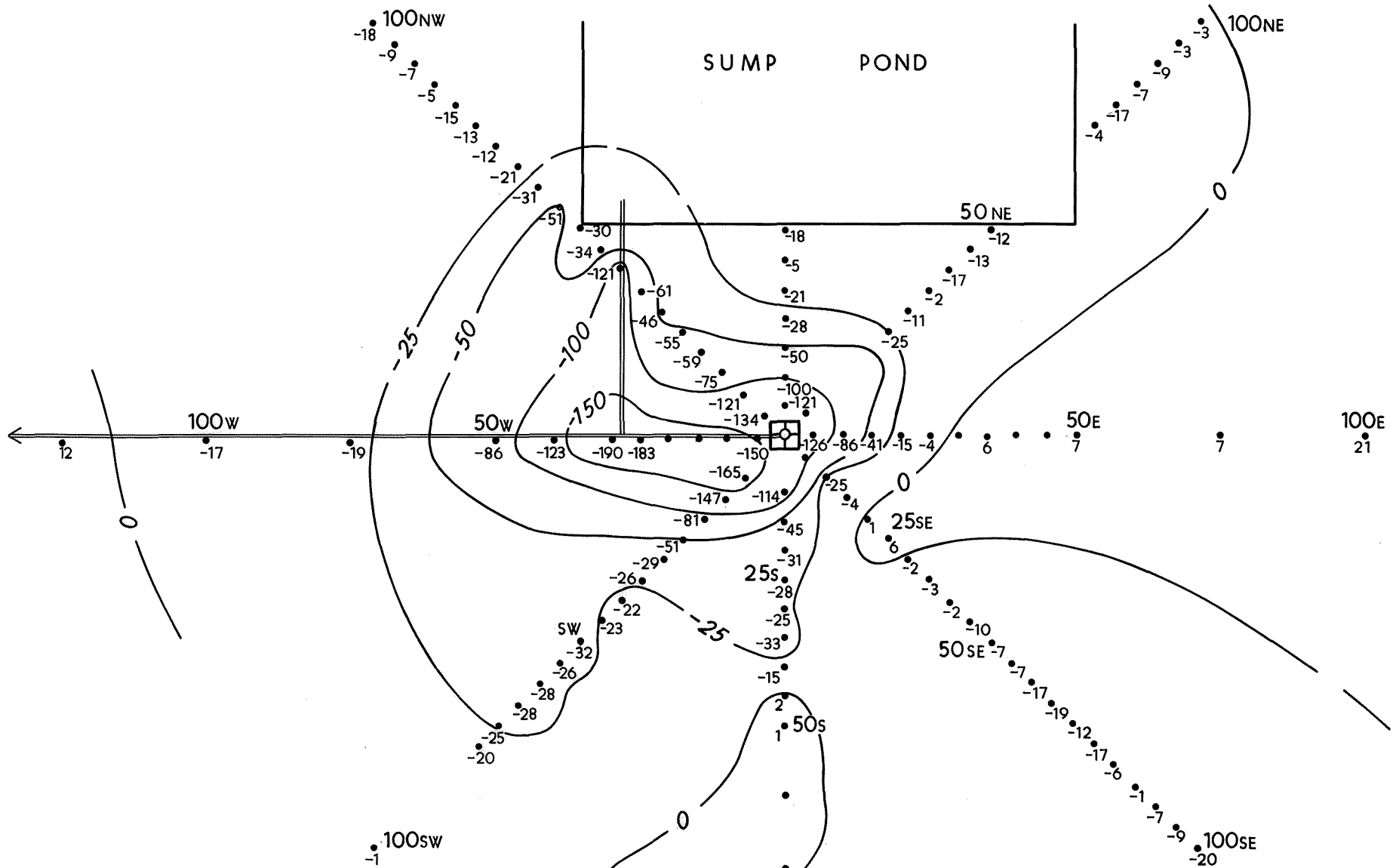
FIGURE 4 DETAILED SP RESULTS EAST MESA AREA IMPERIAL COUNTY, CALIFORNIA 0 25 FEET SCALE
