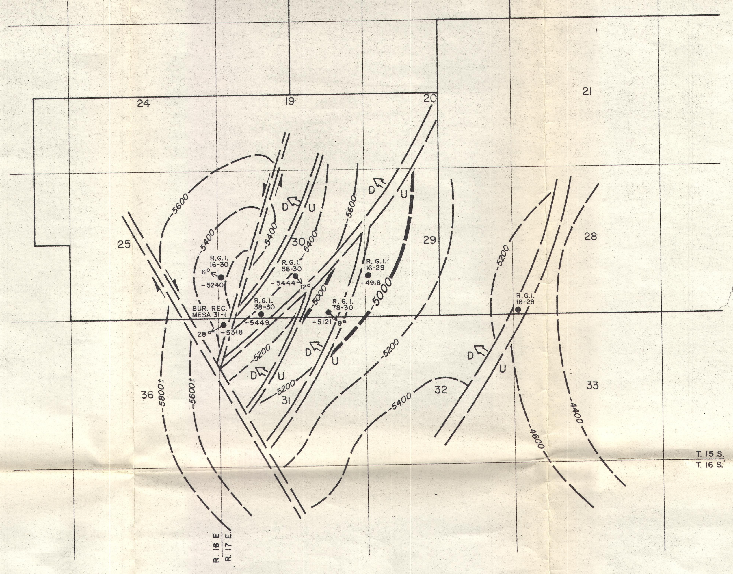
EAST MESA STRUCTURE CONTOUR MAP D 1 HORIZON
