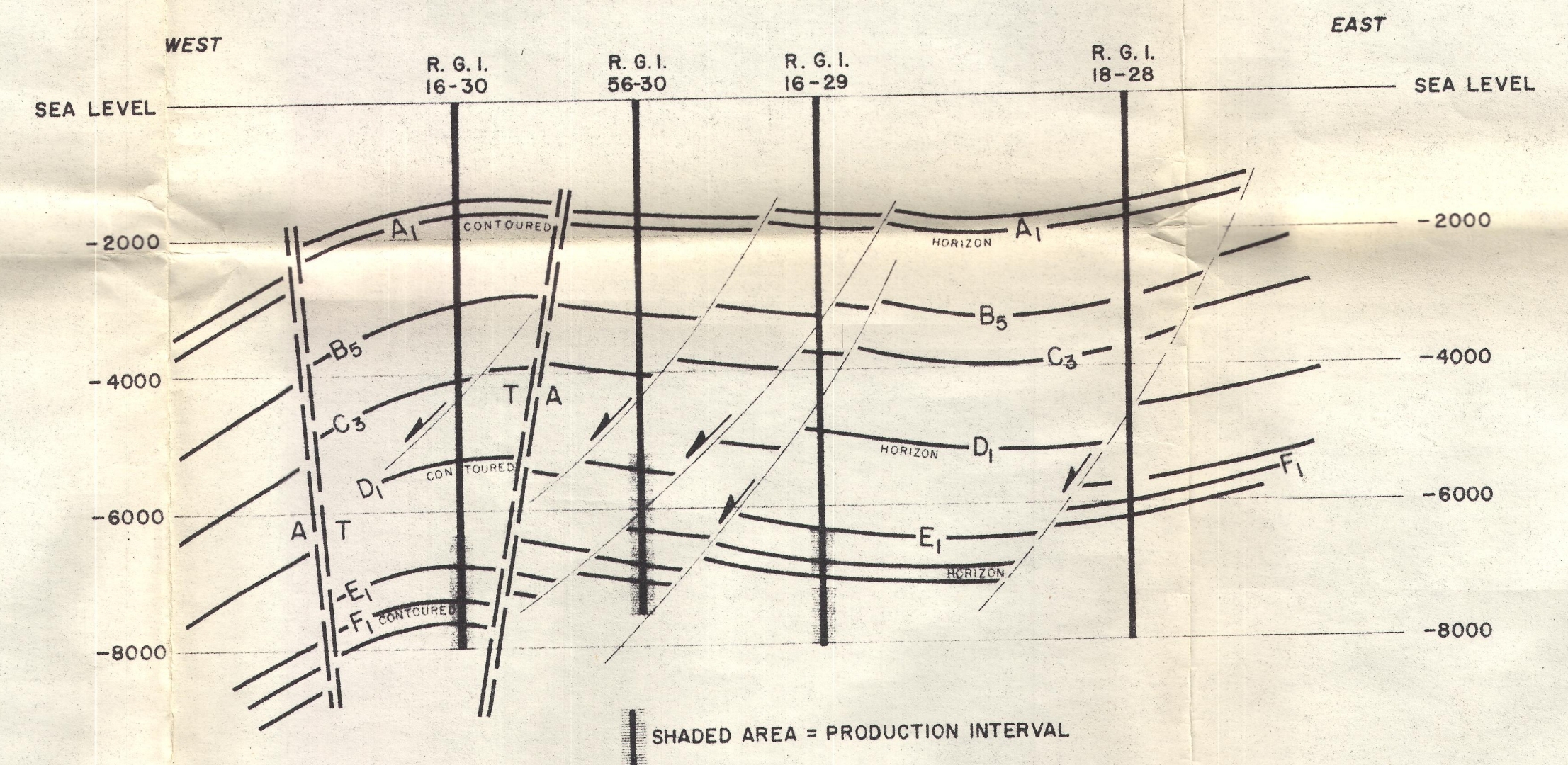
EAST MESA STRUCTURAL CROSS SECTION SCALE: 1" = 2000'
