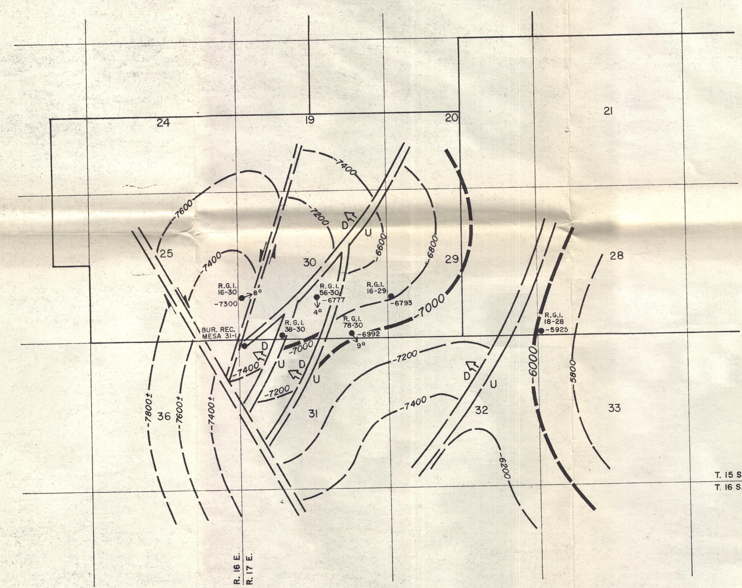
EAST MESA STRUCTURE CONTOUR MAP F 1 HORIZON
