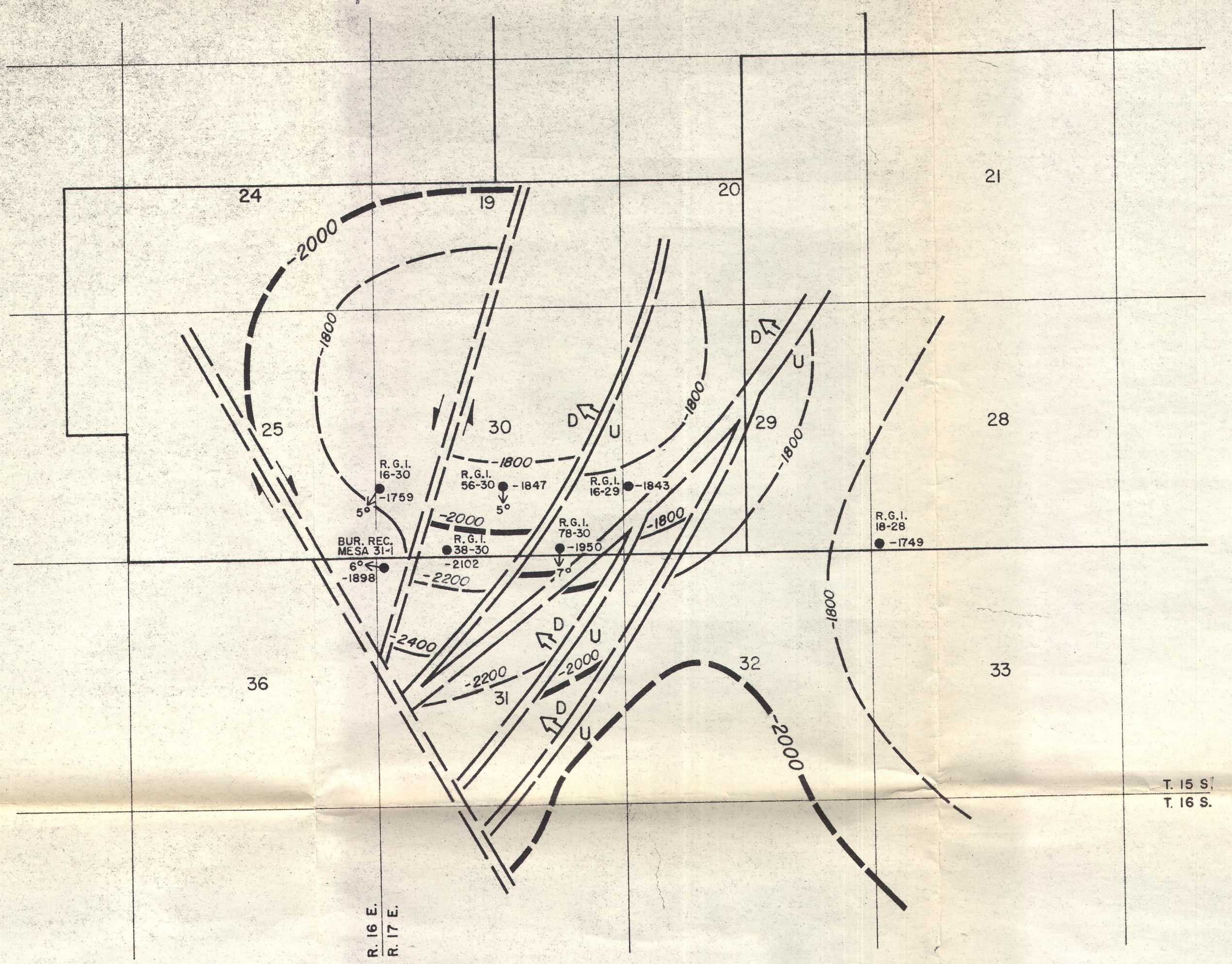
EAST MESA STRUCTURE CONTOUR MAP A 1 HORIZON
