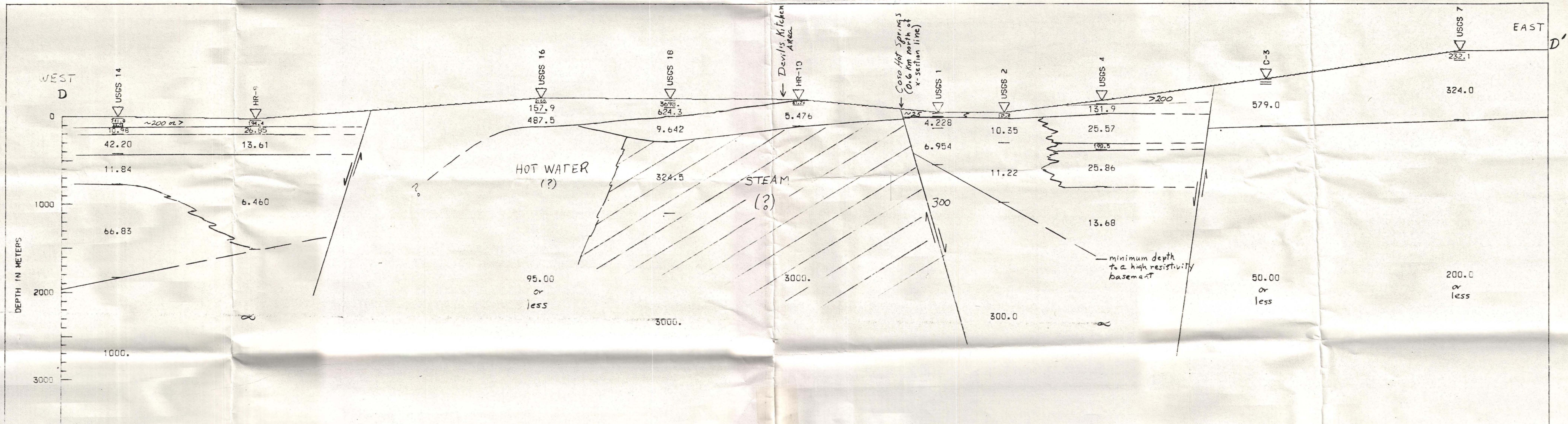
Plate 5.--True T.C. resistivity cross section D-D' (see plate 1 for location). Values are in ohm-m. Major resistivity boundaries are marked by solid or jagged lines; dashed where approximate. Short horizontal lines mark layer boundaries that lie within the major resistivity units. Open triangles are station locations.
