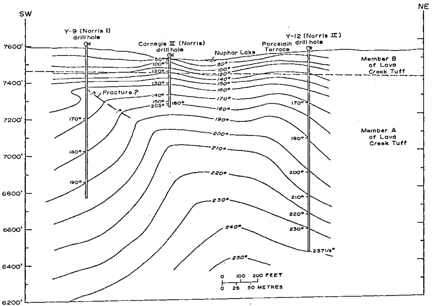
FIGURE 5. Vertical section through Norris Basin drill holes Y-9, Carnegie II, and Y-12, showing bedrock, measured bottom-hole temperatures, and inferred temperature contours. Note contrast between measured and inferred temperatures in Carnegie II drill hole. The inferred fracture near Y-9 presumably connects with others (not shown) that account for the activity near Carnegie II and Congress Pool. Redrafted from White and others, 1975.
