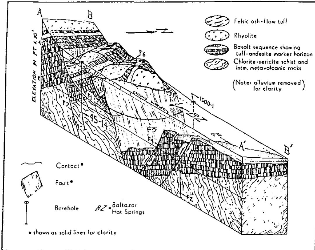
Figure 3. Interpretive 3-D geologic section AA'-BB' through Baltazor Hot Springs and deep well BZ45-14.
