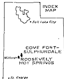
Figure 1. Index Map of Utah illustrating the locations of the Cove Fort-Sulphurdale and Roosevelt Hot Springs KGRA.
