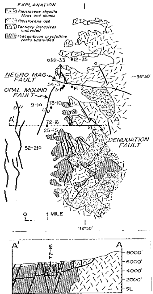
Figure 3. Geology of the Roosevelt Hot Springs Geothermal Area.
