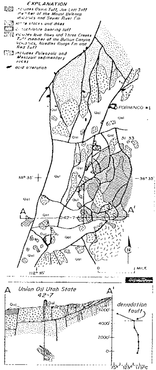
Figure 2. Geology of the Cove Fort-Sulphurdale Geothermal Area.
