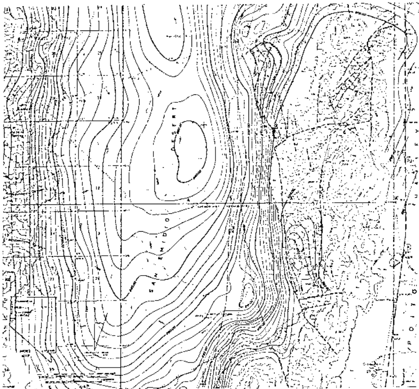
FIGURE 3 BOUGUER GRAVITY MAP
