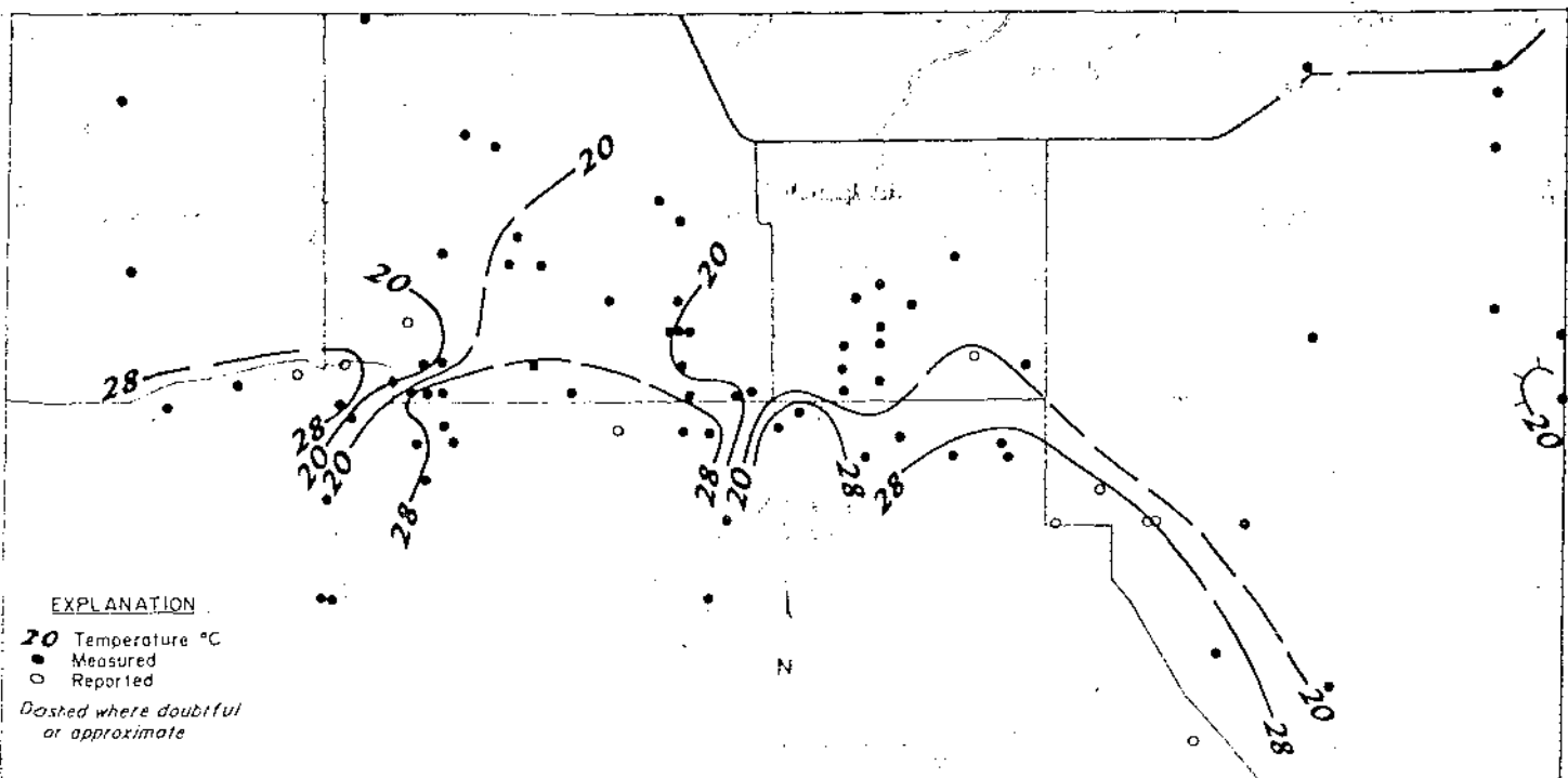
Figure 8. Map of calculated hydrothermal gradients.
