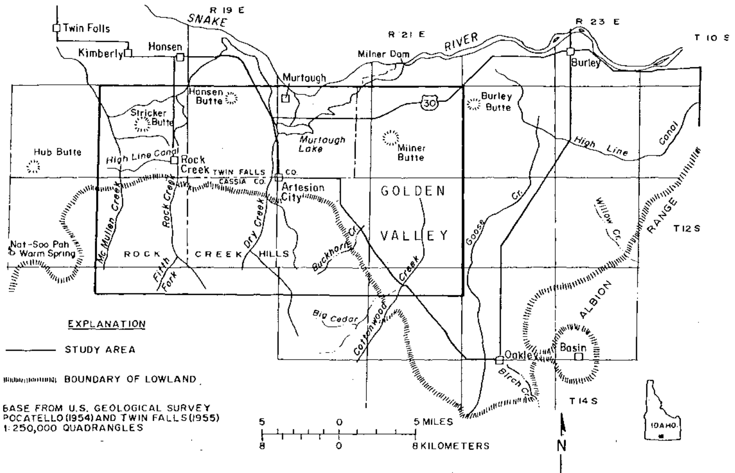
Figure 1. Location map of the Artesian City study area.
