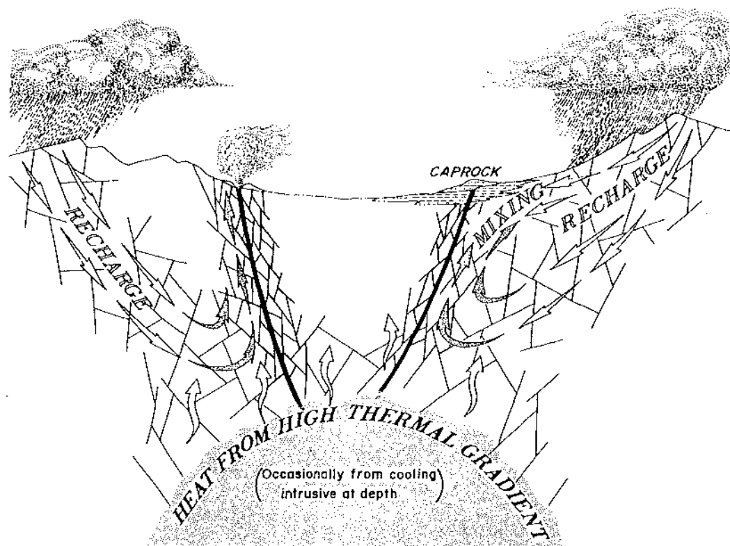
FIG. 1—Generalized model of convective hydrothermal system.
