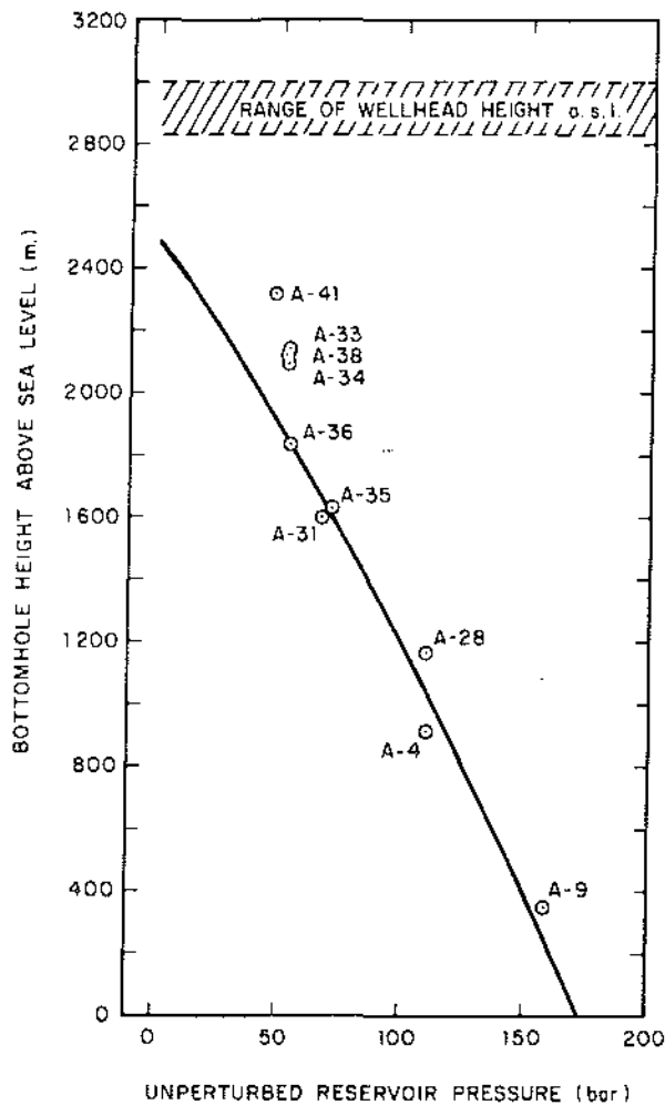
Figure 5. Unperturbed reservoir pressure-depth profile.
