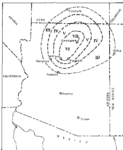
Figure 4: Isoseismal maps
