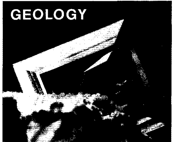
Wulfenite from the 79 mine, Gila County, Arizona. A favorite with mineral collectors, wulfenite occurrence patterns may also help explorationists in their search for porphyry copper deposits (see text). Photo: Stanley Keith.
