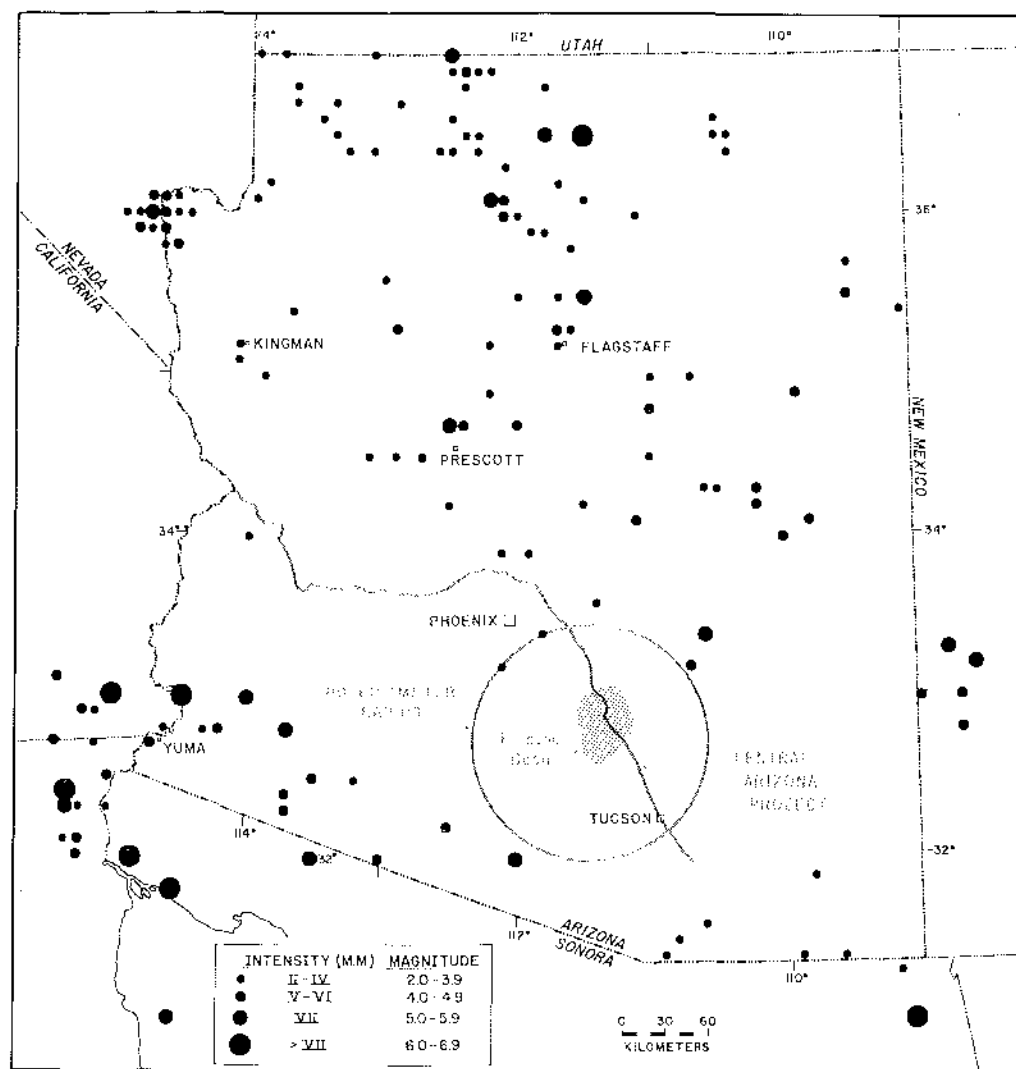
Figure 3: DuBois: Preliminary map of historical earthquake epicenters.
