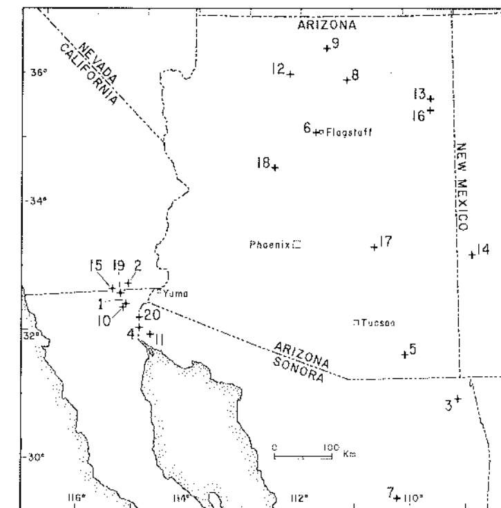
Figure 2: Epicenter locations corresponding to earthquakes in Figure 1.
