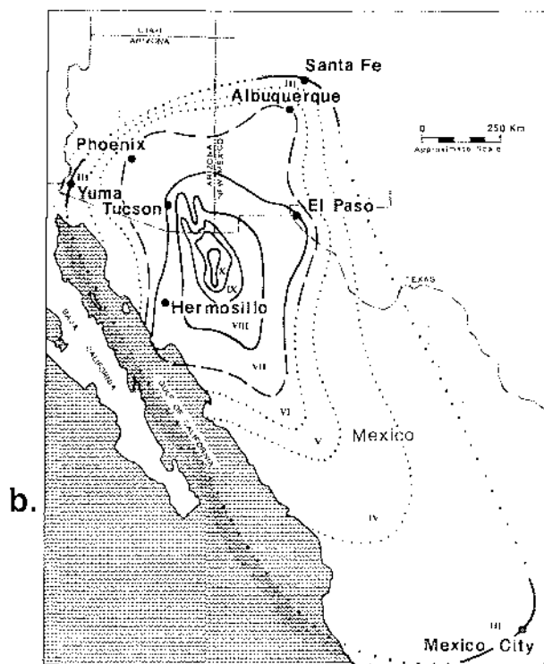
Figure 4: Isoseismal maps
