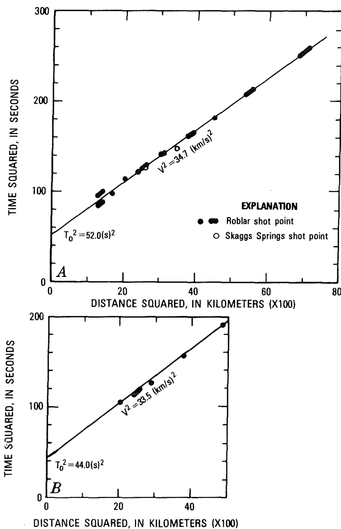
FIGURE 100.—Plots of time squared ( T^2 ) versus distance squared ( X^2 ). V^2 , average velocity squared from surface to point of reflection. T_0^2 , two-way travelttime squared, for vertical path at zero distance. A, Roblar shotpoint, northwest and Skaggs Springs shotpoint, southeast. B, Skaggs Springs shotpoint, northwest.
