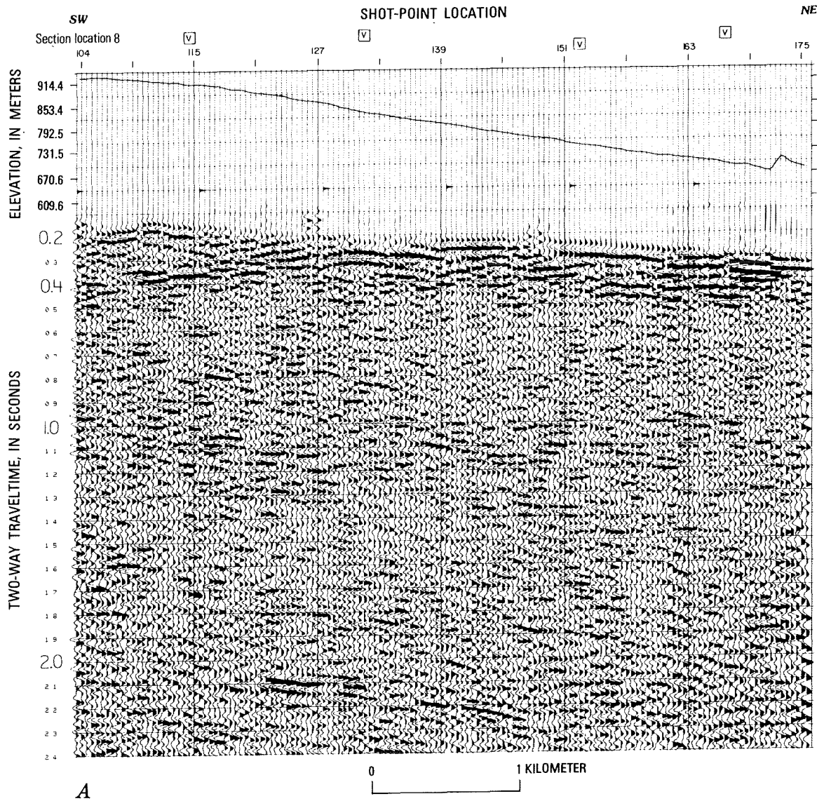
FIGURE 65.—Stacked seismic section along line one showing reflection profile and two-way traveltime. V's mark the position of velocity analyses. Intersection of line two is at section location 8. Deep reflector near 2.1 seconds dipping northeast may represent a major tectonic boundary in the Franciscan assemblage. A, Amplitudes normalized to near-surface rms amplitude. B, Structures accentuated for comparison with geologic section of figure 66. C, Relative amplitudes preserved.
