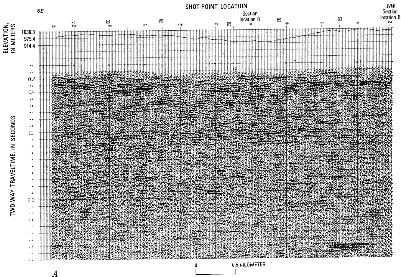
FIGURE 62.—Stacked seismic section along line two showing reflection profile and two-way traveltime. V's mark position of velocity analyses. Southwest end of line one intersects at section location 8. A, Amplitudes normalized to near-surface rms amplitude. B, Structures accentuated for comparison with geologic section of figure 63. C, Relative amplitudes preserved.
