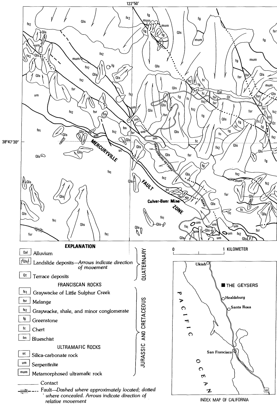
FIGURE 118.—Geologic map of the Geysers-Culver-Baer mine area (from McLaughlin, 1975a).
