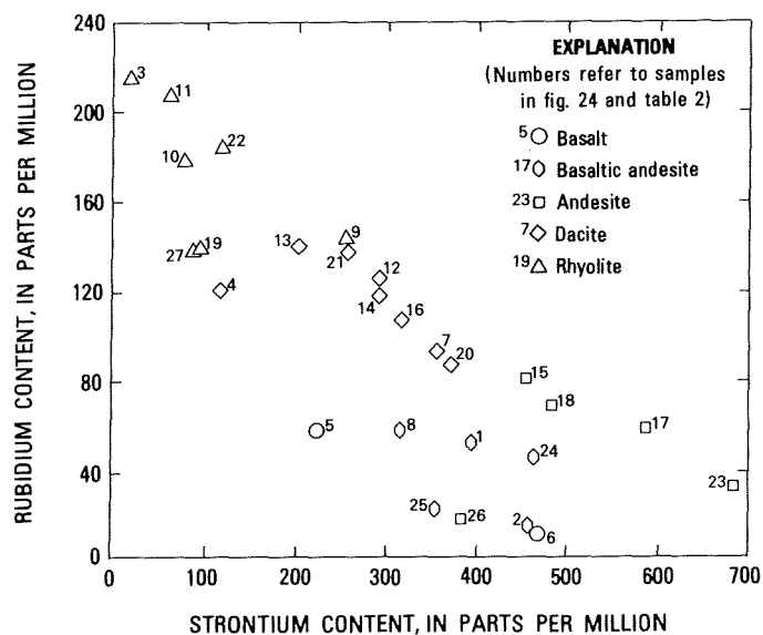
FIGURE 26.—Rubidium versus strontium concentrations.
