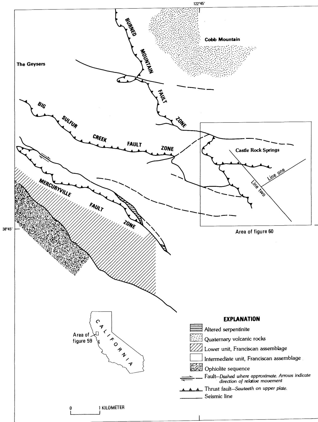
FIGURE 59.—Regional geology and structure of the Geysers-Castle Rock Springs geothermal area, modified from McLaughlin (1978).
