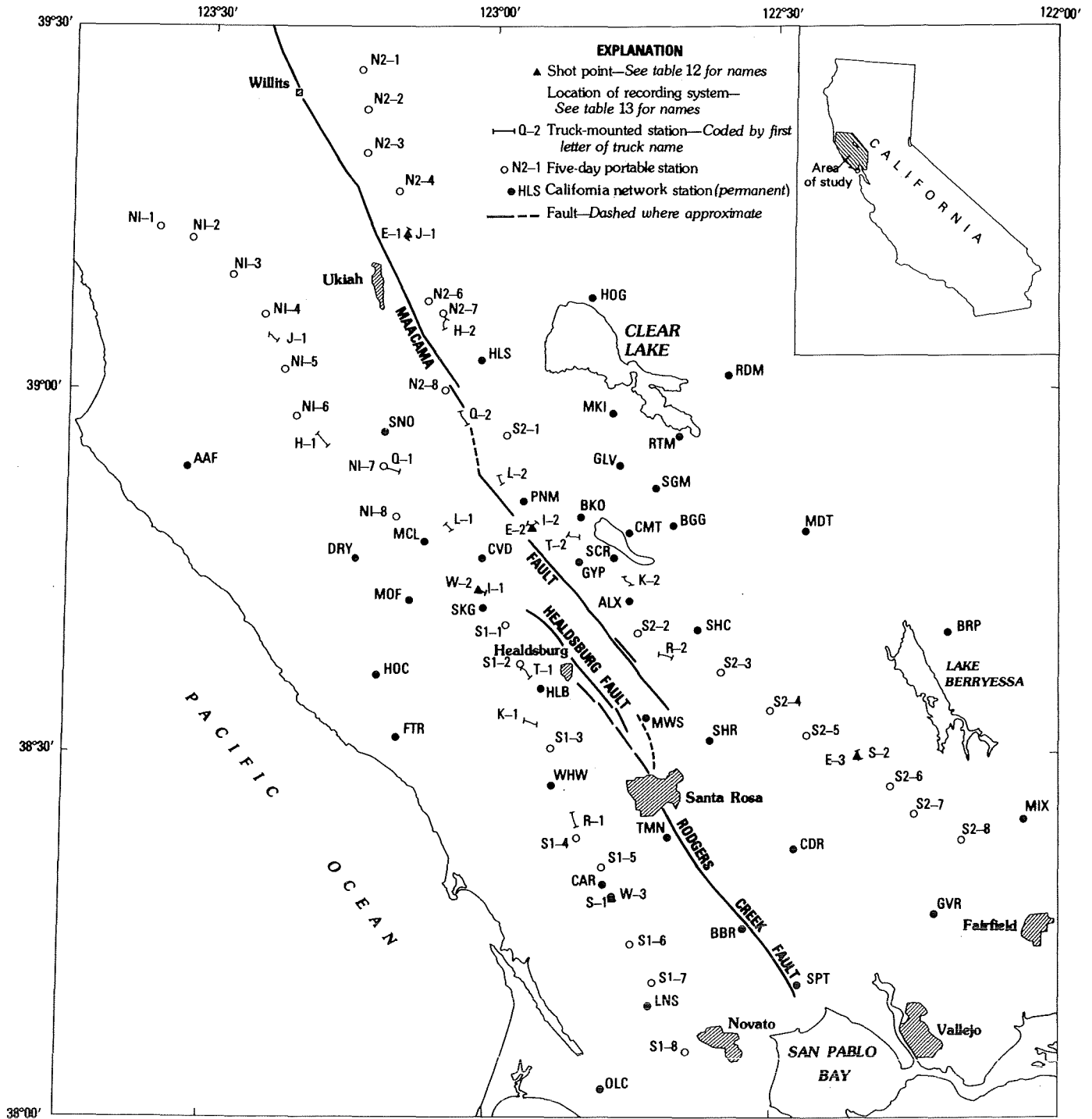
FIGURE 94.—Locations of seismic recording stations, shotpoints, and faults in the Santa Rosa-Ukiah area, California.
