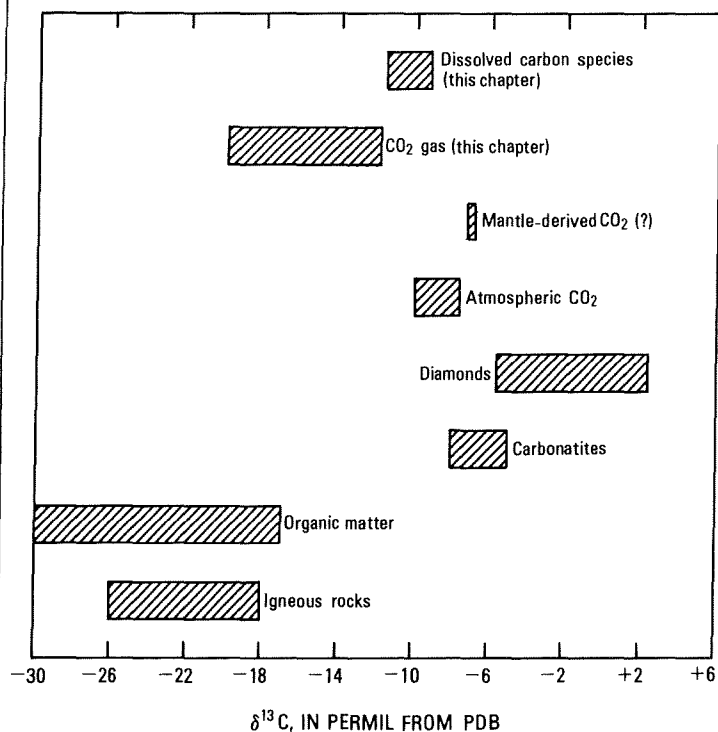
FIGURE 106.—Carbon isotope composition of samples from the Geysers-Clear Lake region compared with isotopic compositions of possible sources. Source data derived from Craig (1963), Taylor, French, and Degens (1967), and Fuex and Baker (1973). PDB, Peedee belemnite standard.
