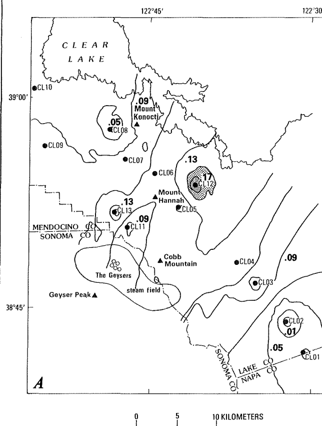
FIGURE 88.—Two-dimensional contoured surface fitted to averaged \delta t^* . Contour interval, 0.02 s. A, \delta t^* data for seismic waves from the southwest. B, \delta t^* data from southeast. C, \delta t^* data from the northwest. \delta t^* is assumed zero at reference station, CL02. Solid area has maximum value of \delta t^* .
