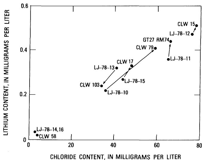
FIGURE 108.—Plot of lithium versus chloride.
