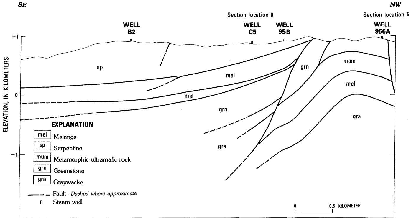
FIGURE 63.—Geological section along reflection line two.
