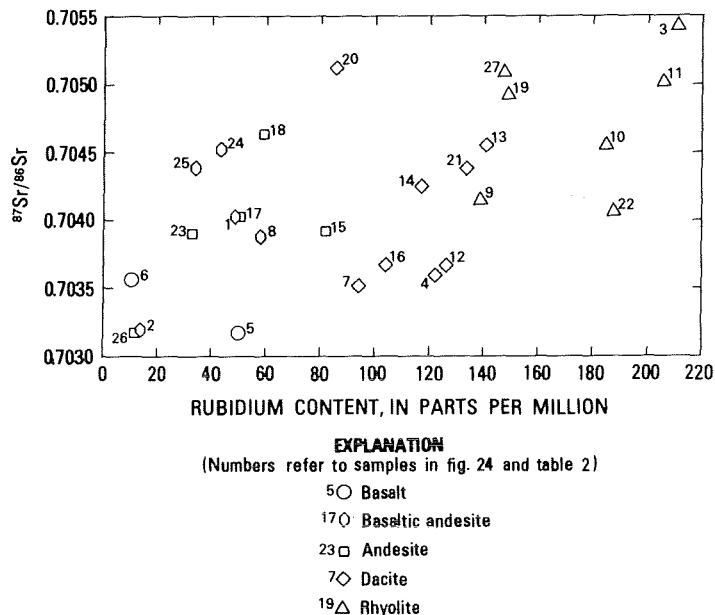
FIGURE 27.— ^{87}\text{Sr}/^{86}\text{Sr} ratios versus Rb concentrations.
