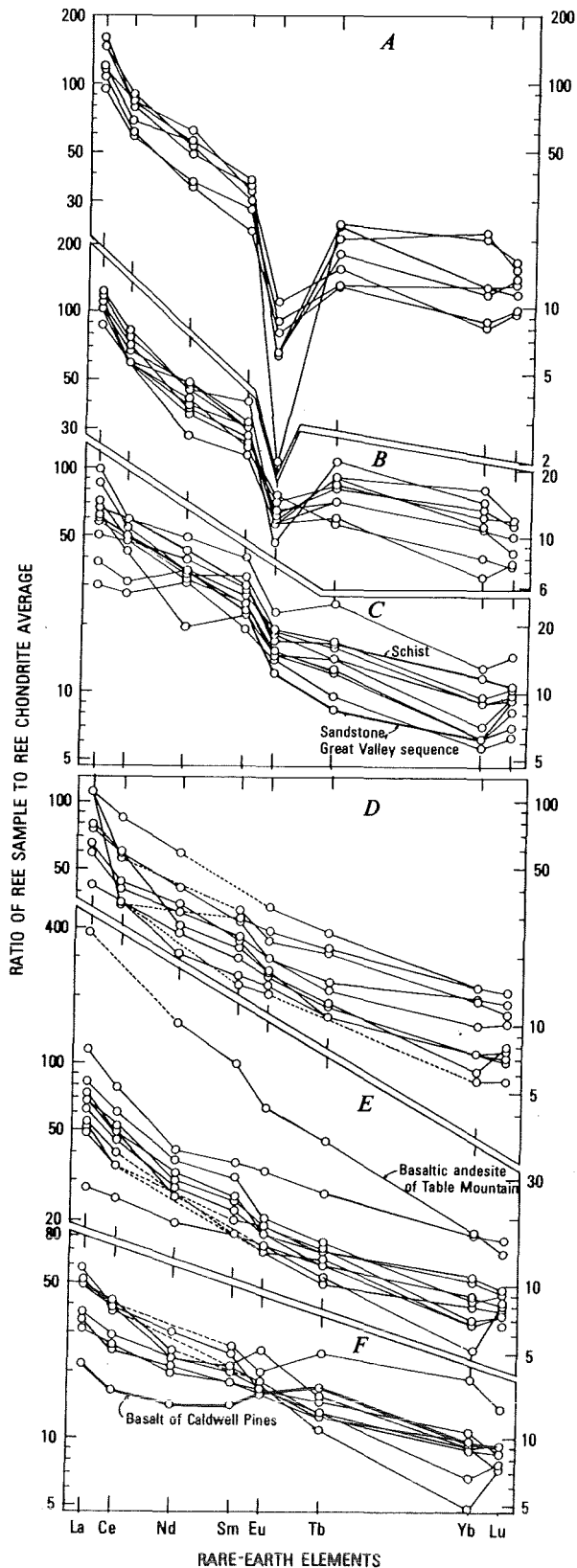
FIGURE 19.—Representative chondrite-normalized rare-earth element (REE) patterns of Clear Lake Volcanics, inclusions, and Great Valley sandstone. A, Rhyolites. B, Dacites. C, Diabase-textured and granular inclusions, schist inclusion in andesite of Perini Hill, and sandstone of Great Valley sequence from unit IVD of Swe and Dickinson (1970). D, Andesites. E, Basaltic andesites. F, Basalts. Neutron-activation analyses by P. A. Baedeker, L. J. Schwarz, and J. J. Rowe, U.S. Geological Survey.
