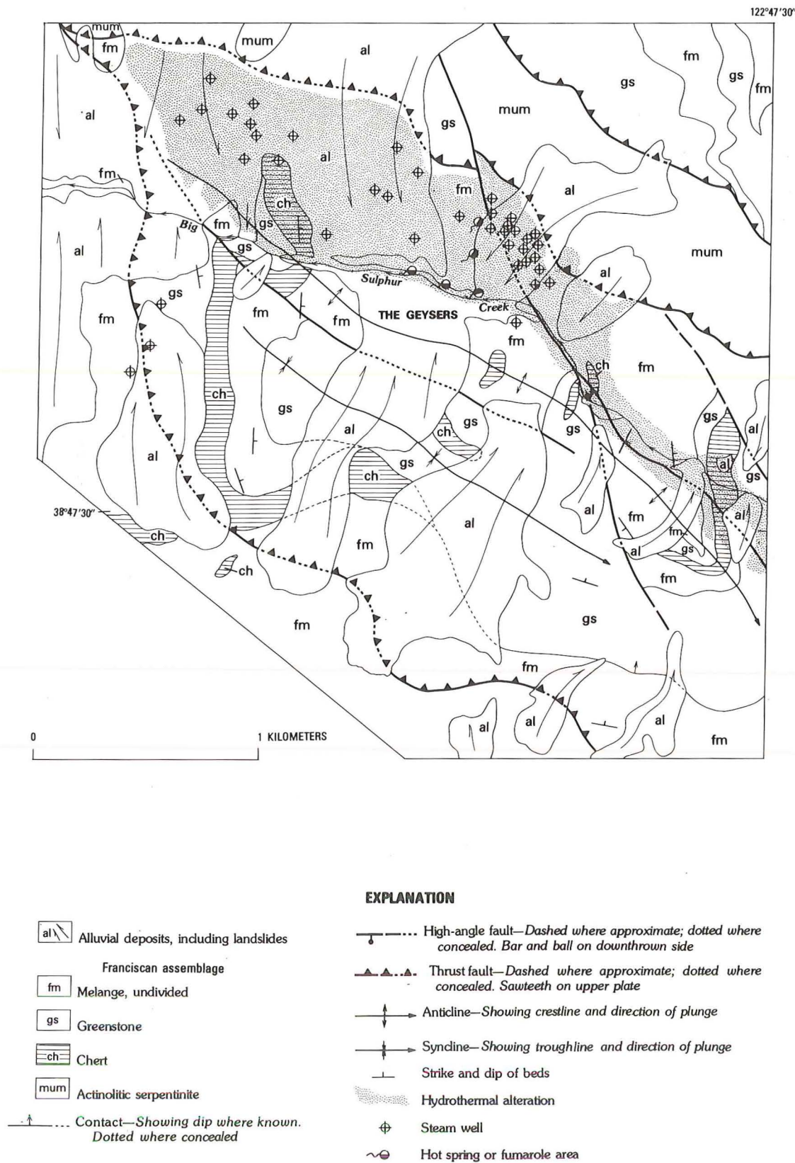
FIGURE 10.—Geology of the Geysers area, illustrating folds in Franciscan chert and extensive hydrothermal activity along Big Sulphur Creek.
