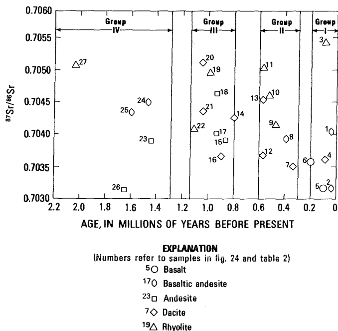
FIGURE 25.— ^{87}\text{Sr}/^{86}\text{Sr} ratios versus K-Ar ages. Groups I-IV are separated according to age (see table 1).
