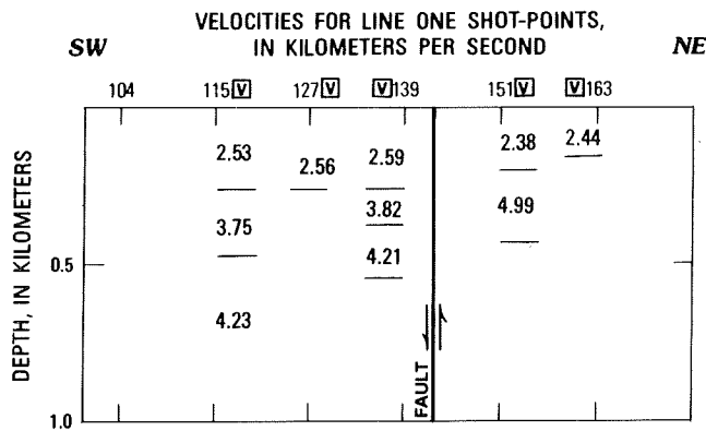
FIGURE 67.— Interval velocity section calculated for seismic line one. Major fault near shotpoint 139 is a tectonic boundary evident from reflection data, surface geology, and lithologic data at Borrows well (see fig. 61).
