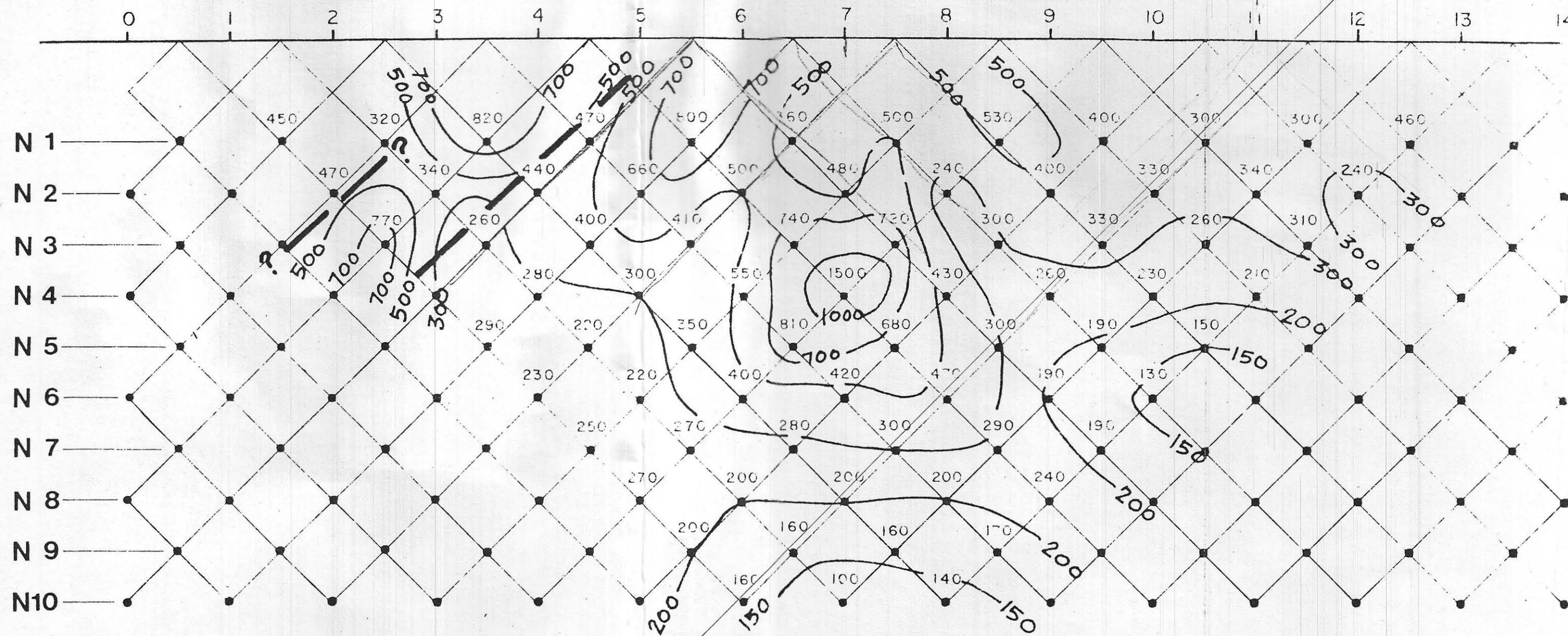
FIGURE 5 DIPOLE - DIPOLE RESISTIVITY PSEUDO - SECTION LINE 3
