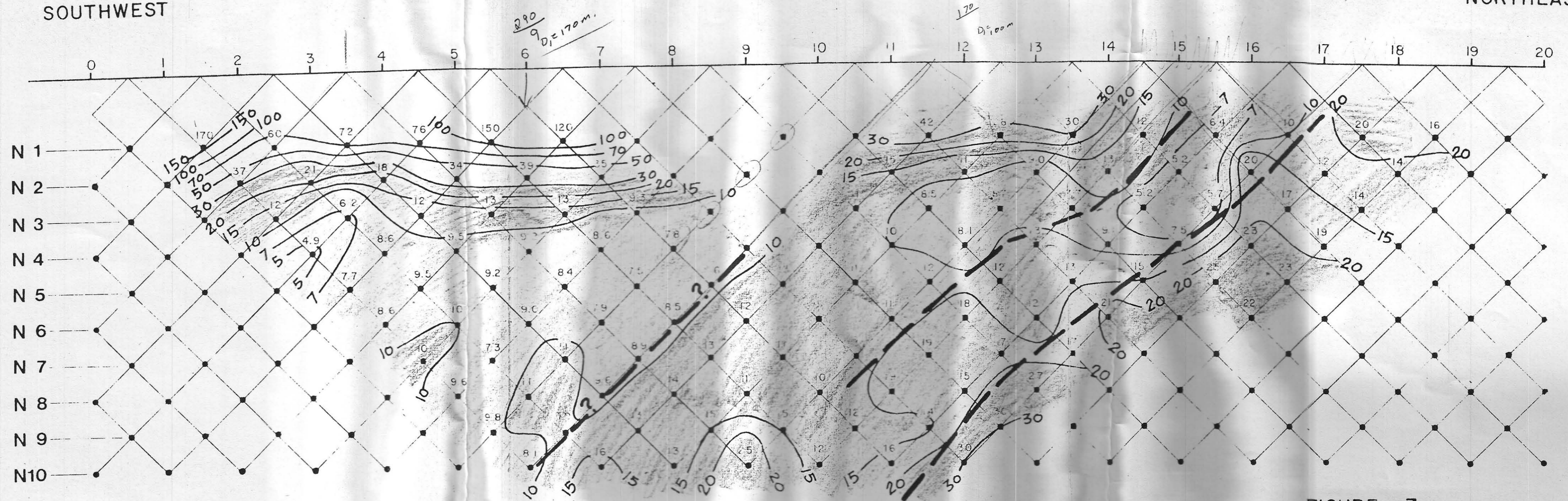
FIGURE 7 DIPOLE-DIPOLE RESISTIVITY PSEUDO-SECTION LINE 5
