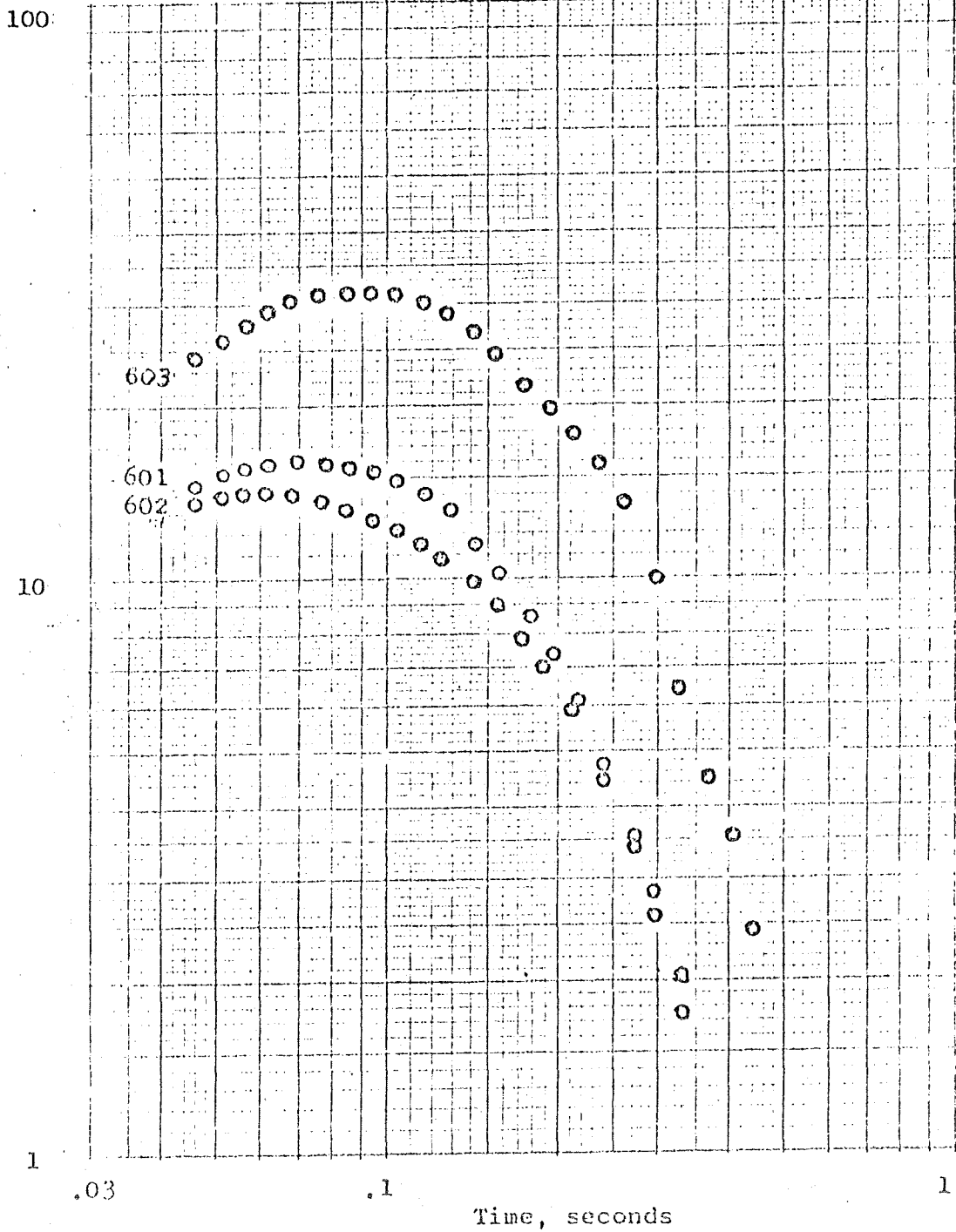
Figure 2Q. Electromagnetic soundings 601, 602 and 603.
