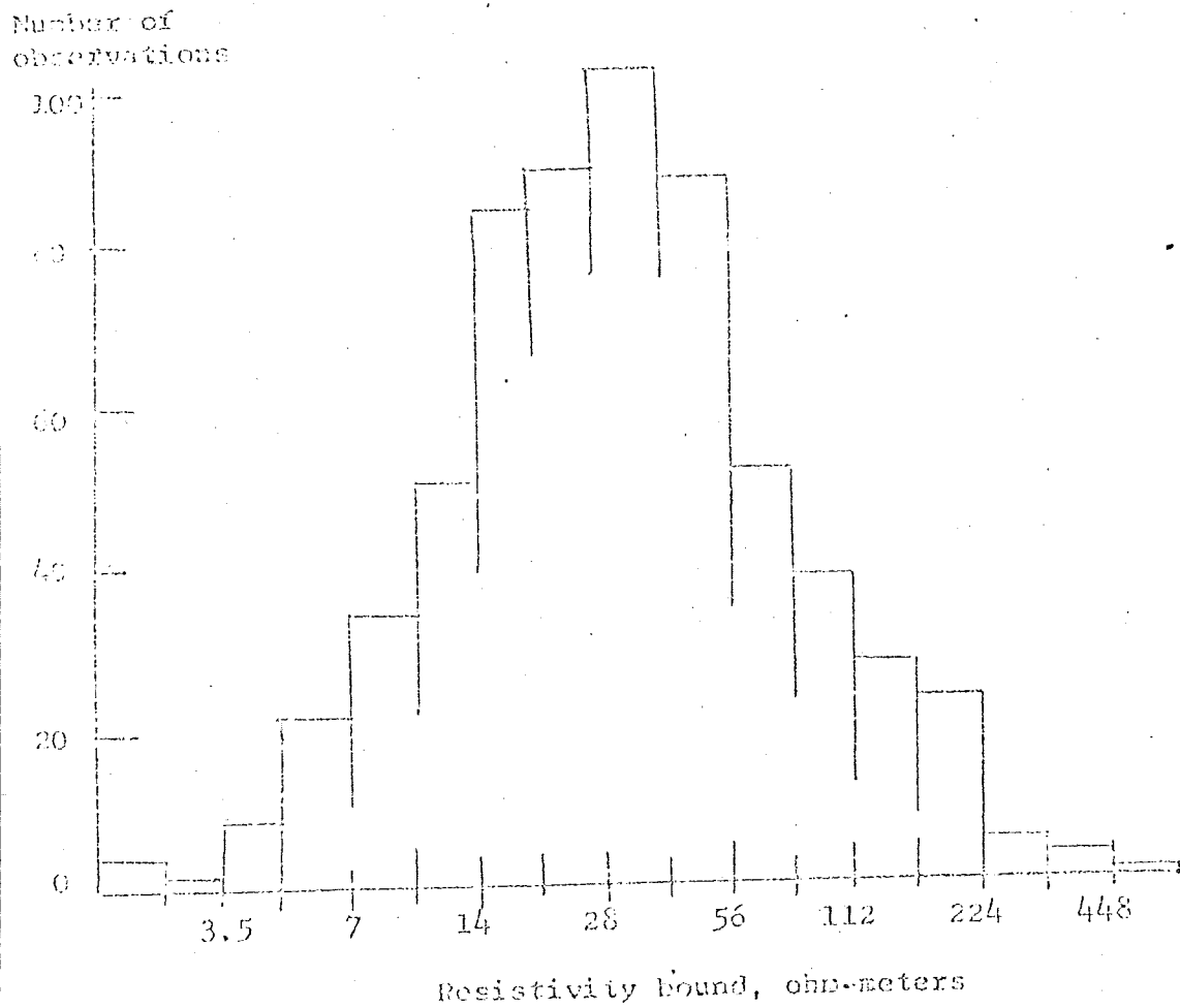
Figure 2. Histogram showing distribution of apparent resistivity values for all measurements made during dipole mapping surveys in the Valles Caldera.
