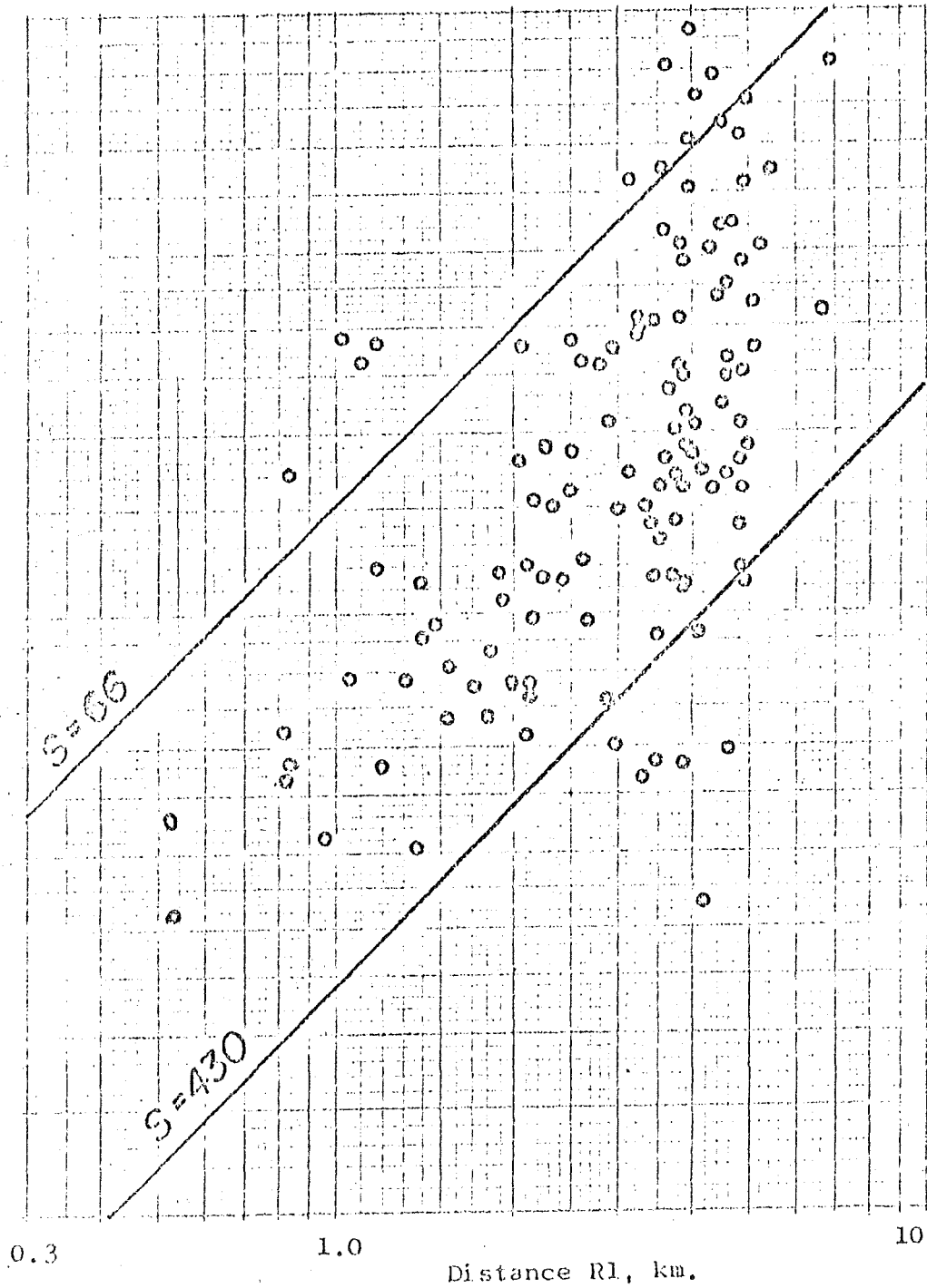
Figure 12. Apparent resistivities measured about source 1, plotted as a function of the distance to the nearer end of the source dipole.
