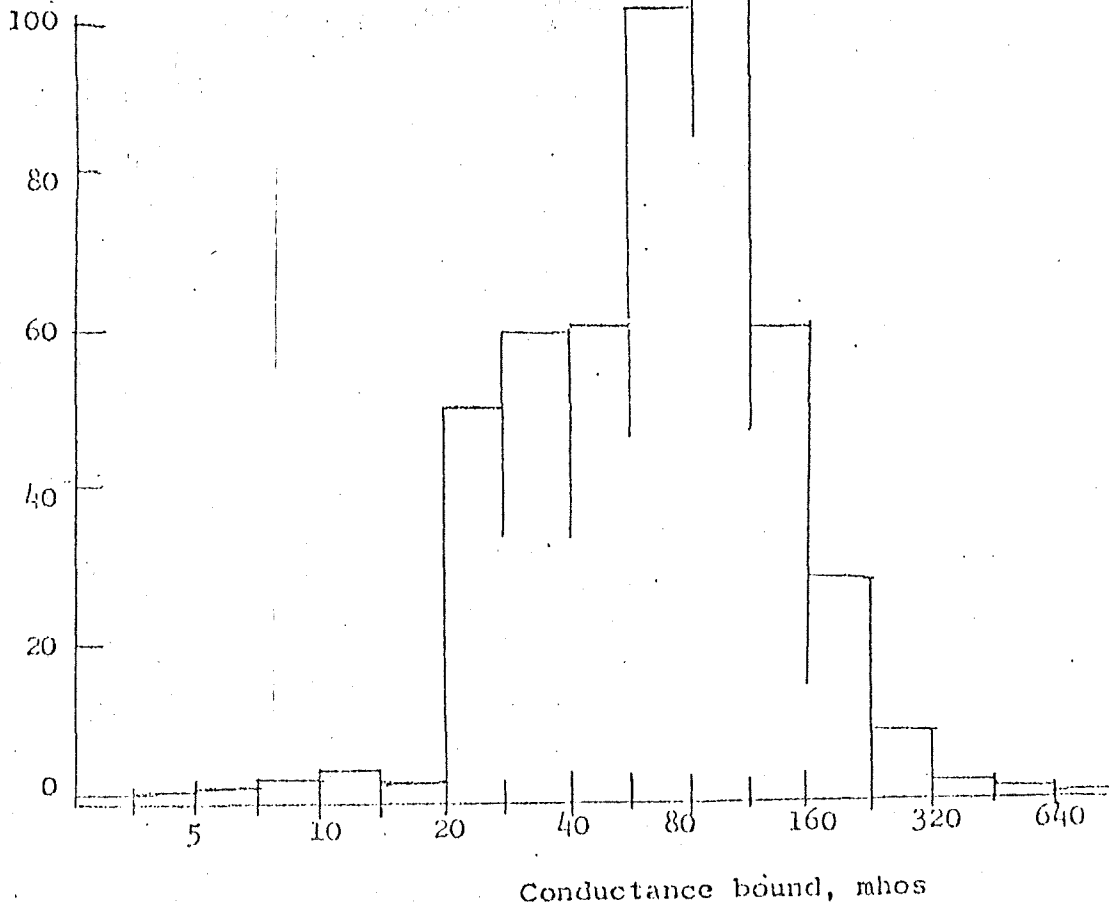
Figure 3. Histogram showing distribution of apparent conductance values for all measurements made during dipole mapping surveys in the Valles Caldera.
