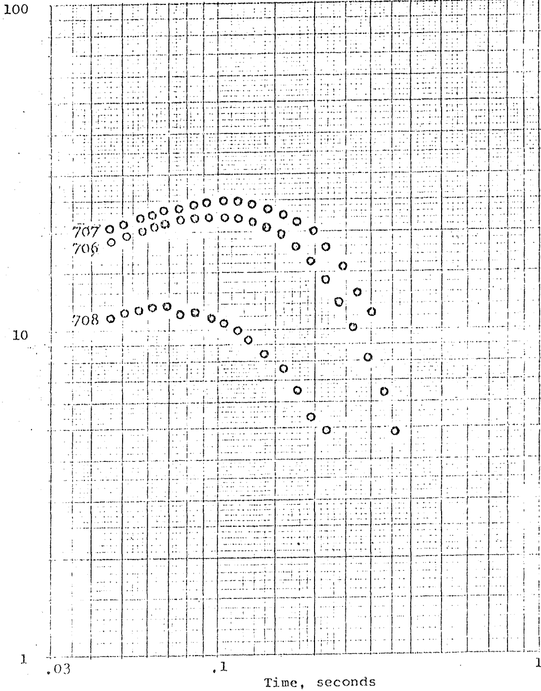
Figure 33. Electromagnetic soundings 706, 707 and 708.
