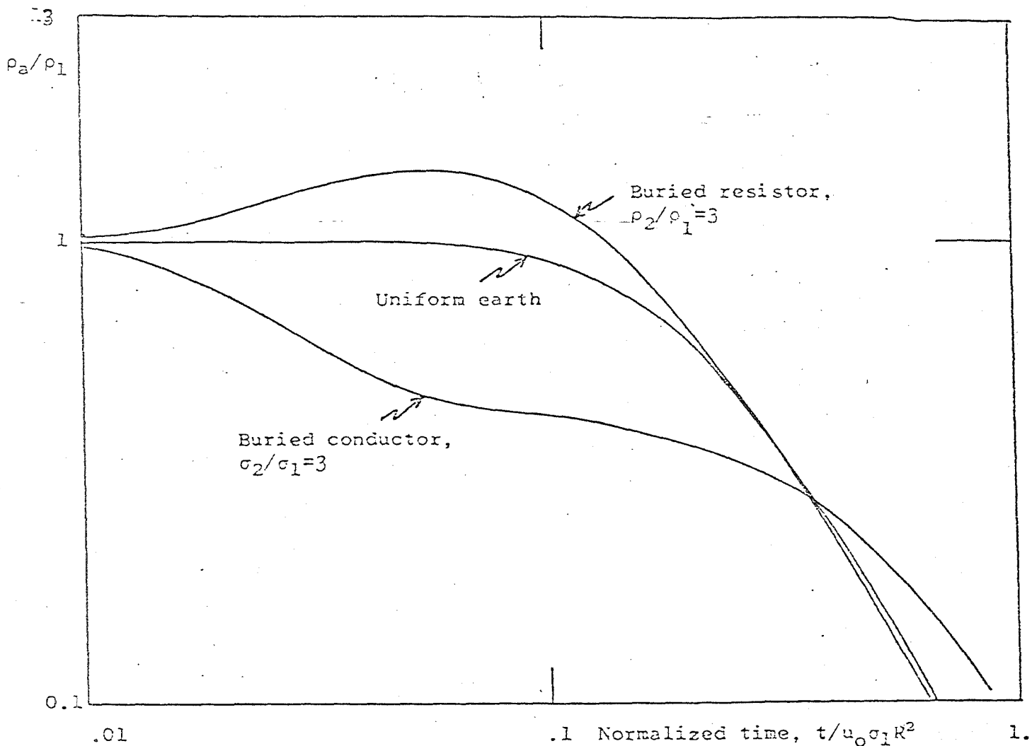
Figure 25. Examples of two-layer electromagnetic sounding curves for the case in which the thickness of the first layer is 1/16 the separation, R.
