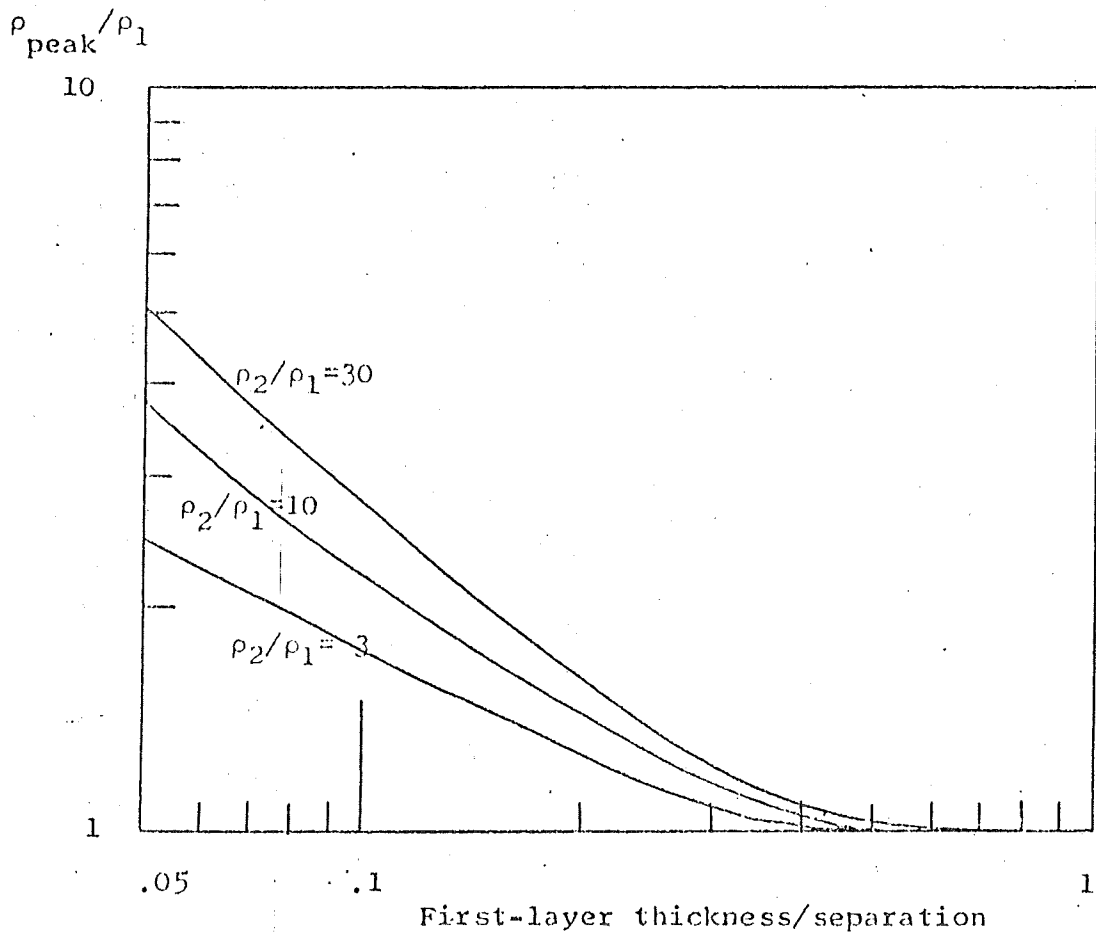
Figure 27. Interpretation chart for evaluating an electromagnetic sounding made over a sequence of two layers in which the second layer is more resistive than the first. Interpretation is based on the ratio of the peak resistivity recorded on the sounding to the first-layer resistivity.
