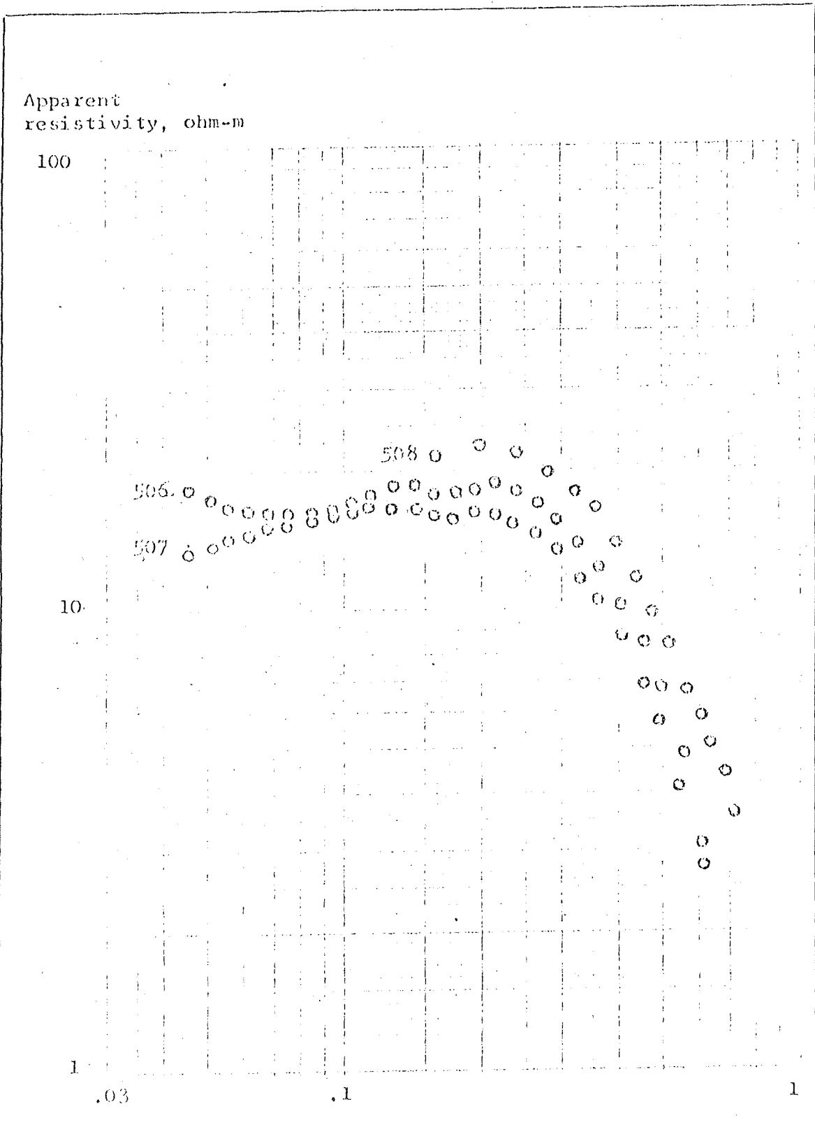
Figure 29. Electromagnetic soundings 506, 507 and 508.
