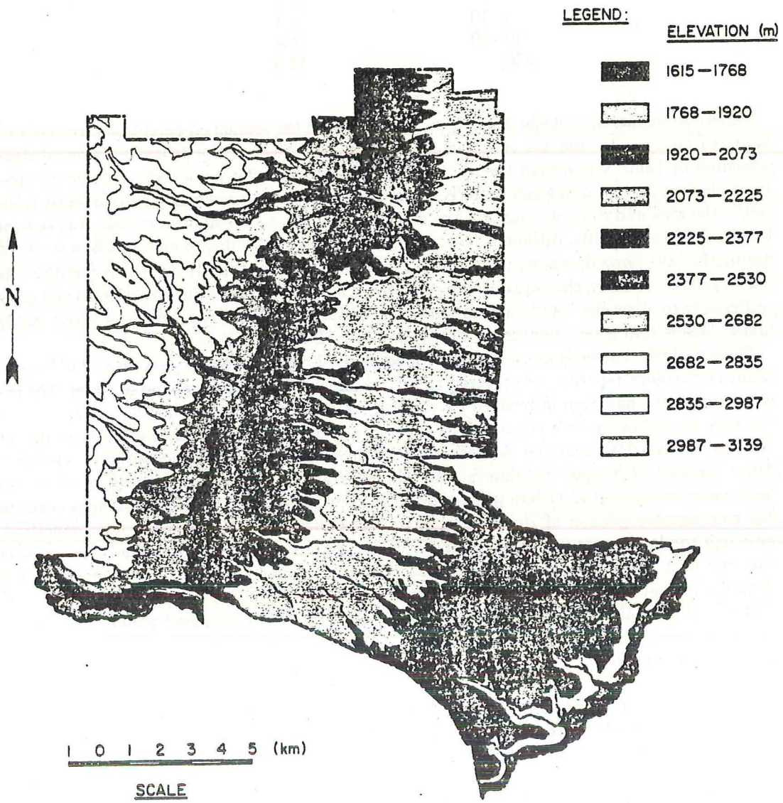
Fig. 6. Topography and intermittent streams of Los Alamos County.
