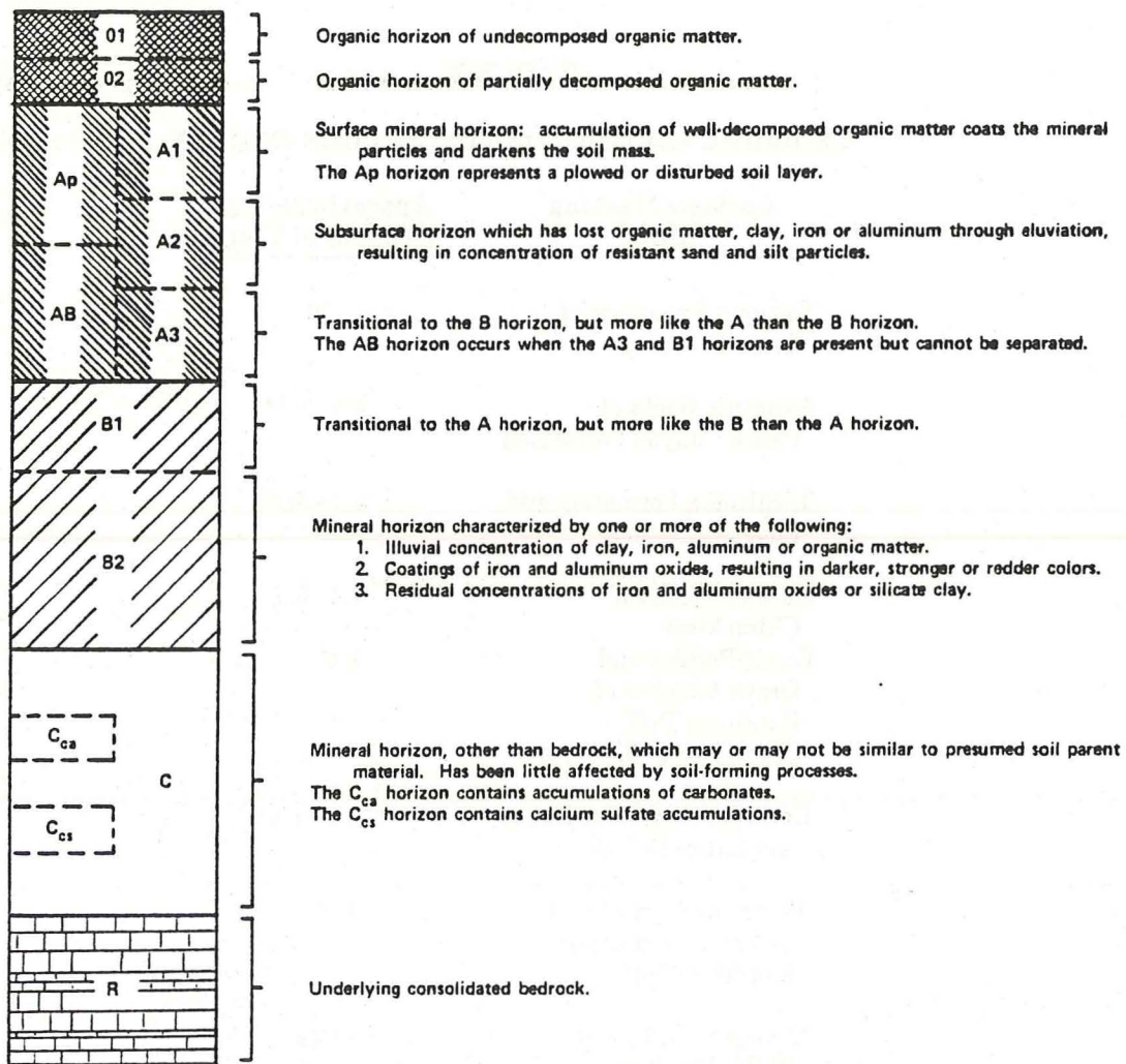
Fig. 7. Hypothetical soil profile showing principal horizons.
