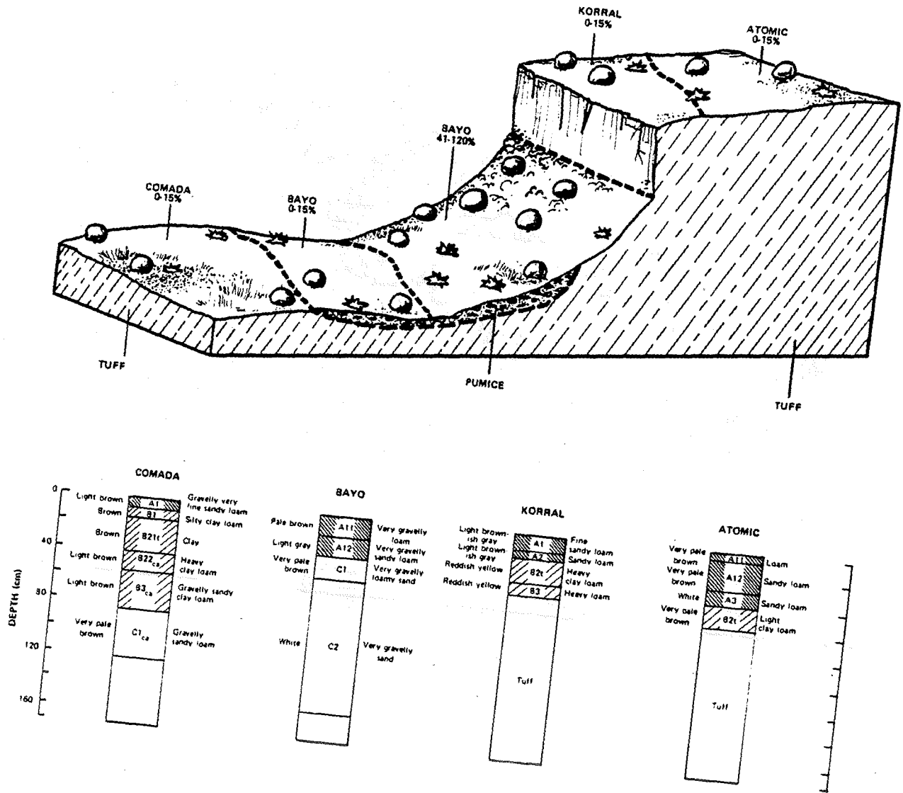
Fig. 17. Relationship of slope, vegetation, and parent material to Comada, Bayo, Korral, and Atomic soils.
