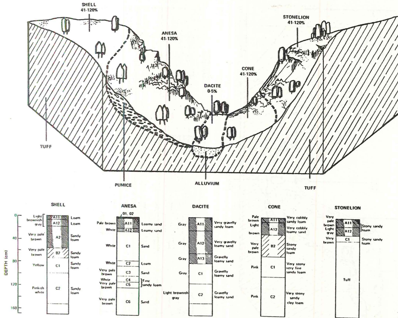
Fig. 20. Relationship of slope, vegetation, and parent material to Shell, Anesa, Dacite, Cone, and Stonelion soils.
