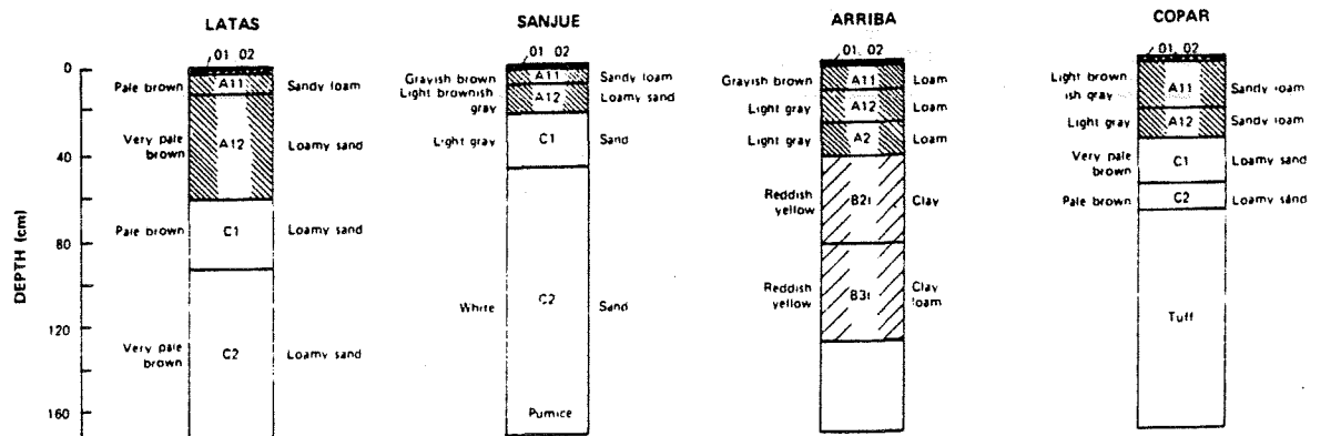
Fig. 16. Relationship of slope, vegetation, and parent material to Latas, Sanjue, Arriba, and Copar soils.
