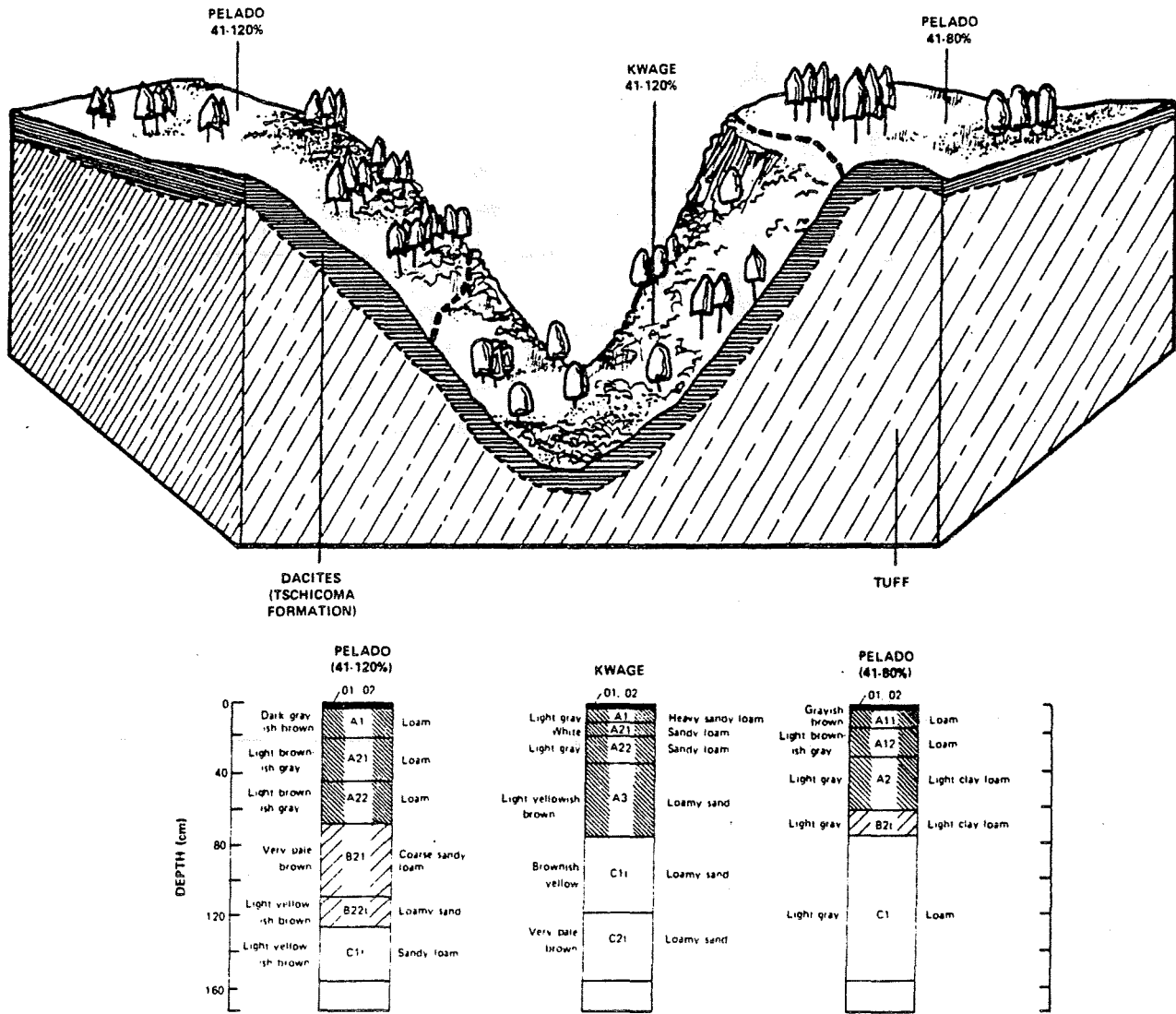
Fig. 22. Relationship of slope, vegetation, and parent material to Pelado and Kwage soils.
