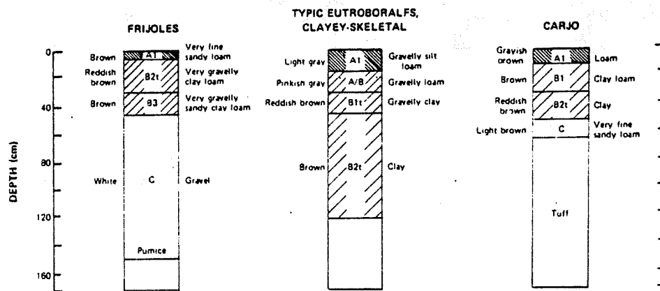
Fig. 10. Relationship of slope, vegetation, and parent material to Frijoles, Typic Eutroboralfs, clayey-skeletal, and Carjo soils.
