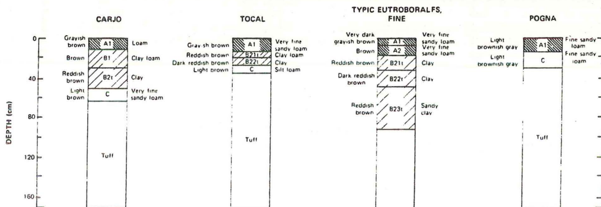
Fig. 9. Relationship of slope, vegetation, and parent material to Carjo, Tocal, Typic Eutroboralfs, fine, and Pogna soils.
