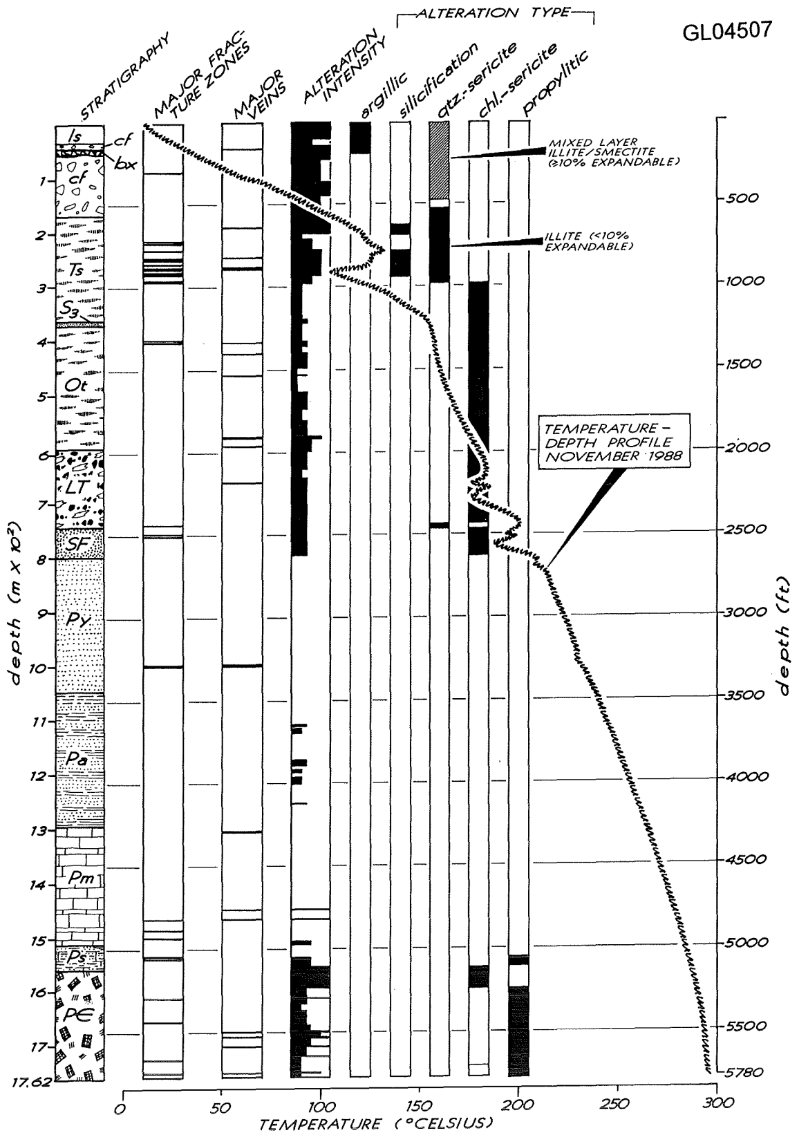
Figure 2. Summarized geologic log for CSDP corehole VC-2B, Sulphur Springs area, Valles caldera, New Mexico.
