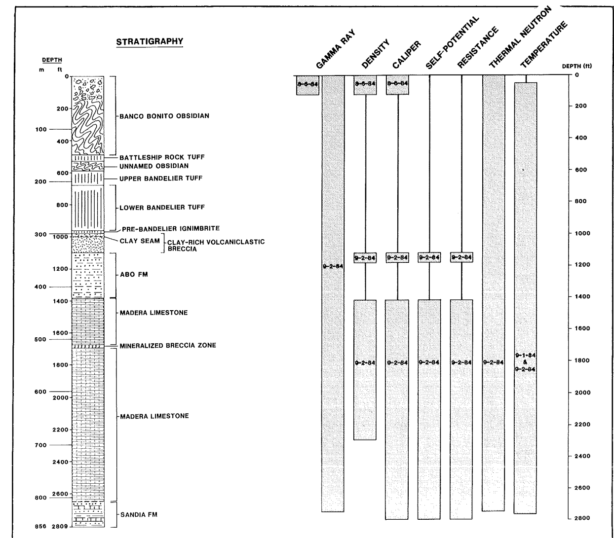
Fig. 27. Geophysical logging intervals in VC-1, in relationship to stratigraphy. Stippled bars with dates indicate logged intervals.
