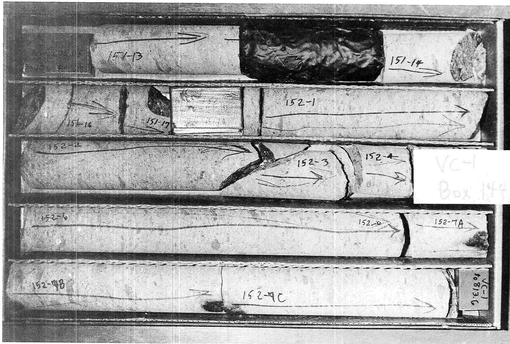
Fig. 19. Core runs 151 and 152, depth 805 to 813.6 ft. Densely welded Lower Bandelier Tuff showing core markings. Note the waxed section. Note excellent recovery of intact core (see Fig. 17).
