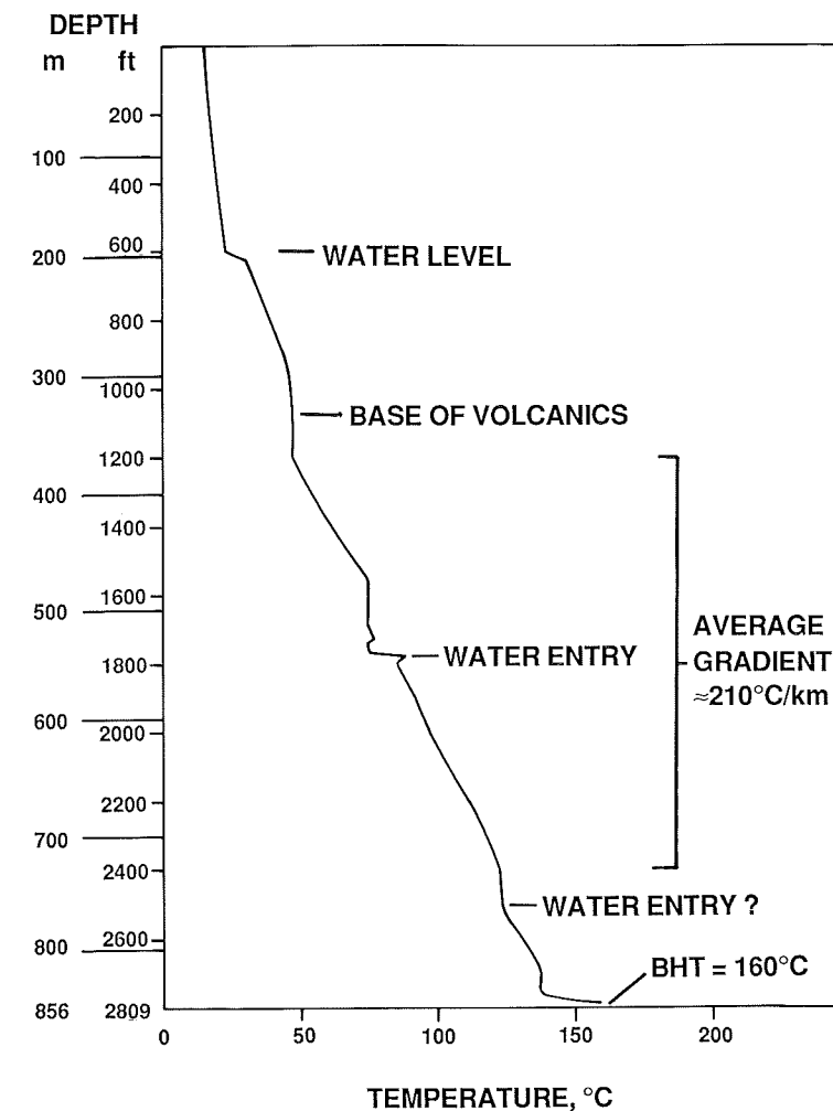
Fig. 3. VC-1 Temperature gradient (24 h after completion).
