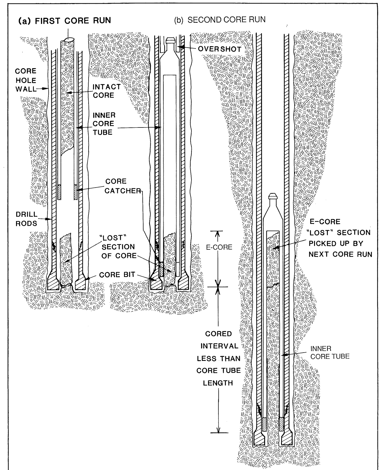
Fig. A-4. Example of extra core (E-Core).
