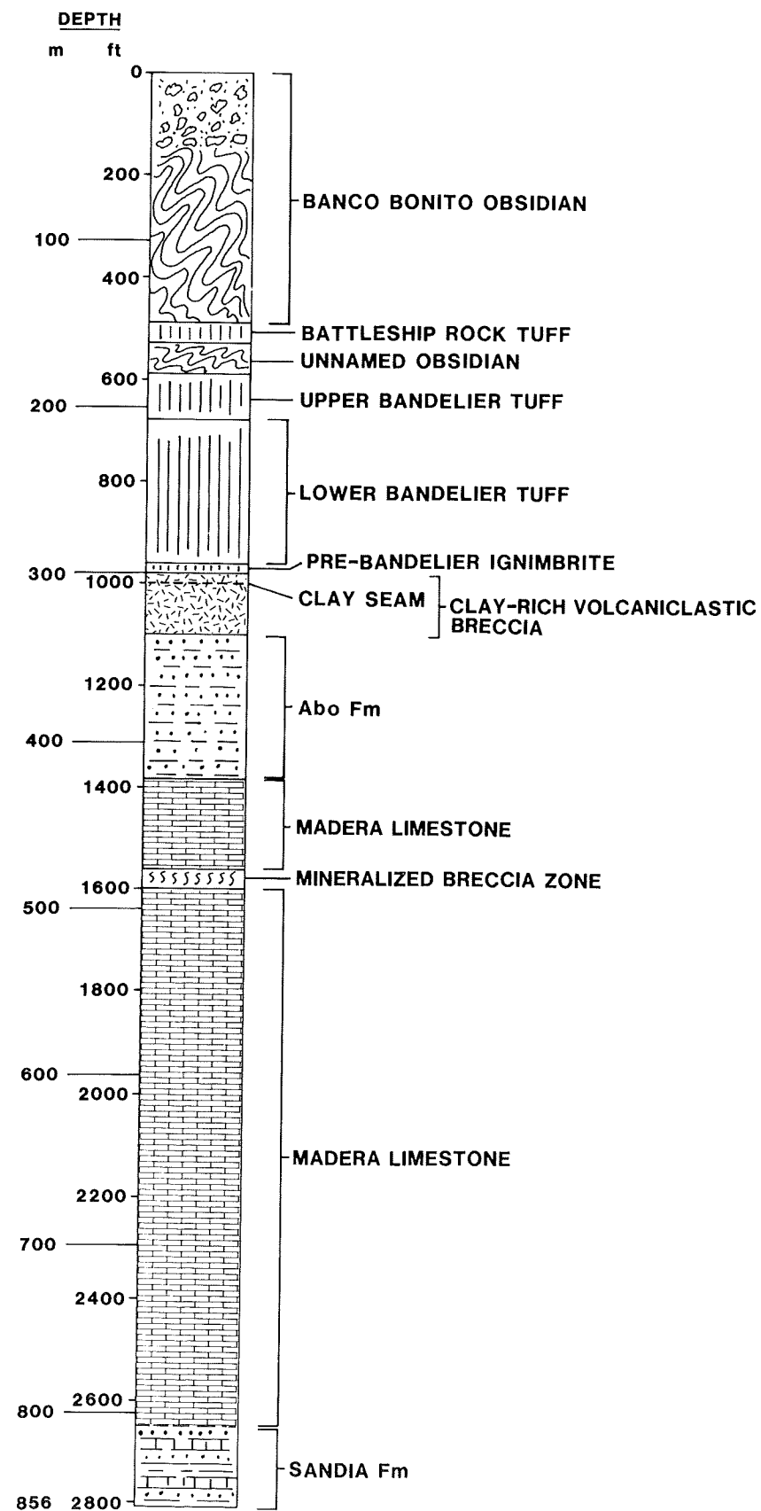
Fig. 2. Core hole VC-1 stratigraphy.
