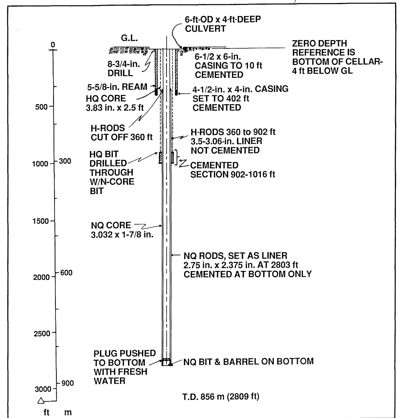
Fig. 13. Actual (as-built) VC-1 configuration.
