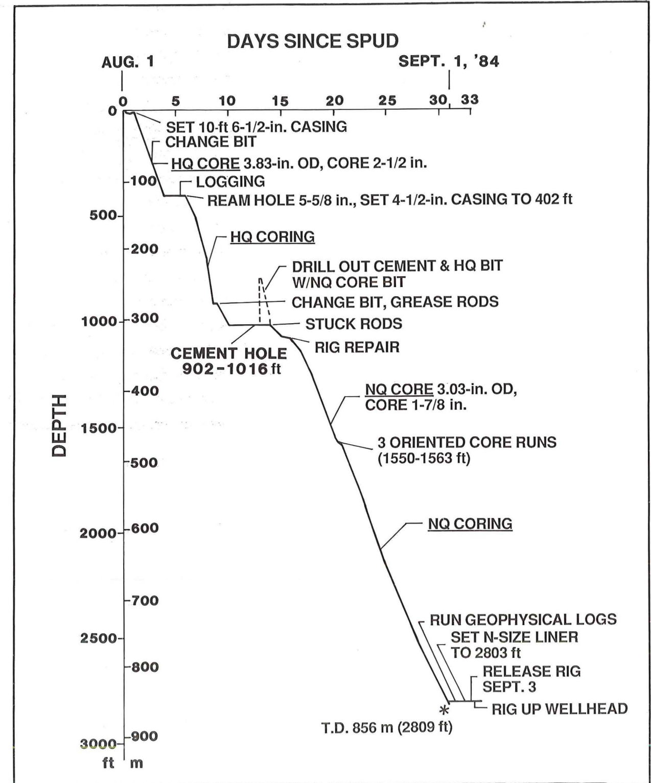
Fig. 12. Coring operations history for VC-1.
