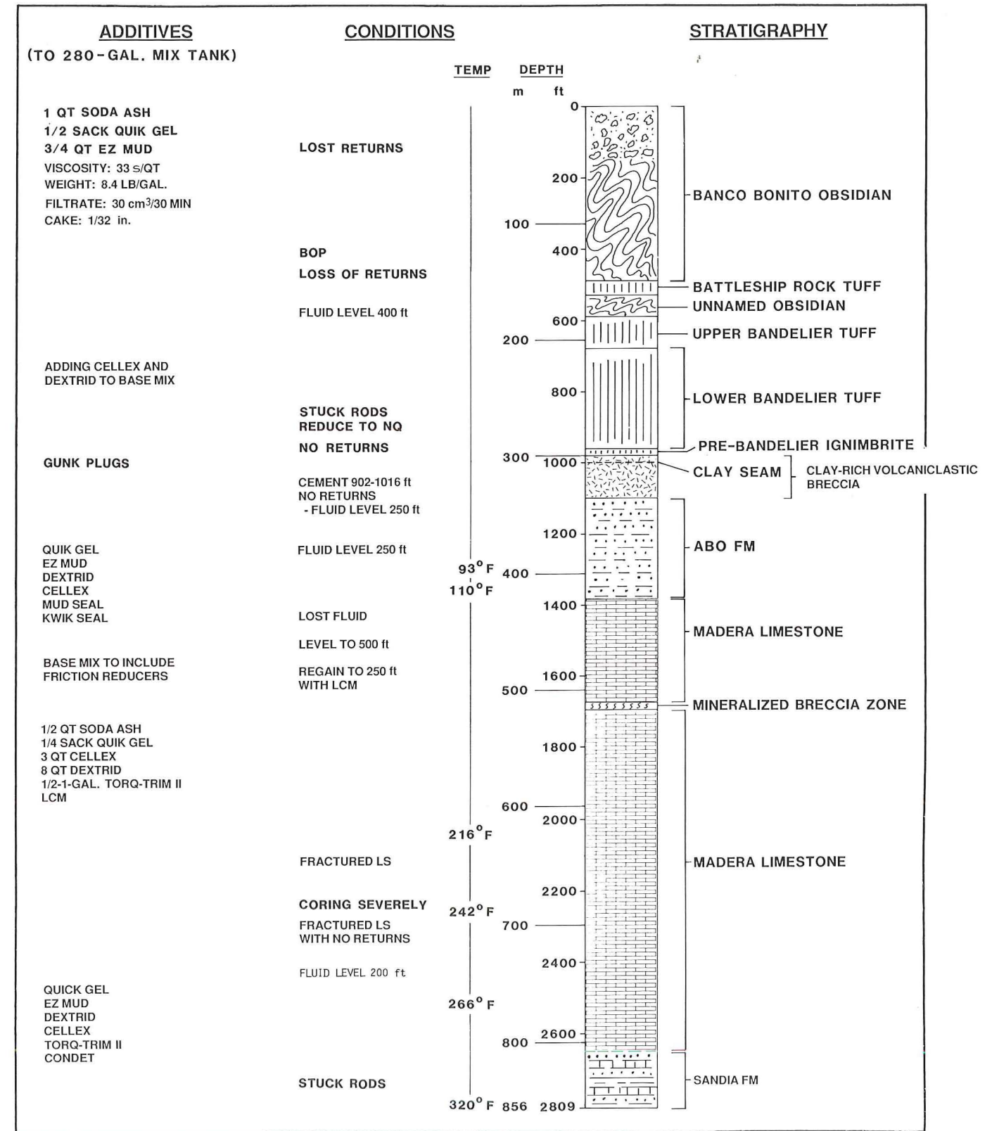
Fig. 24. Drilling fluid program and conditions for VC-1 coring and relation to stratigraphy.
