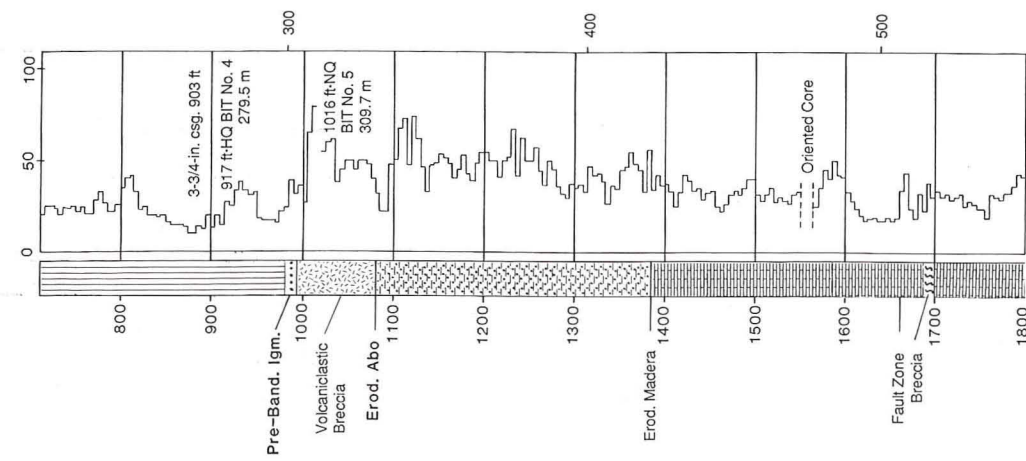
Fig. 22. Time to penetrate 1.5 m (5 ft) as a function of depth and stratigraphy in VC-1.
