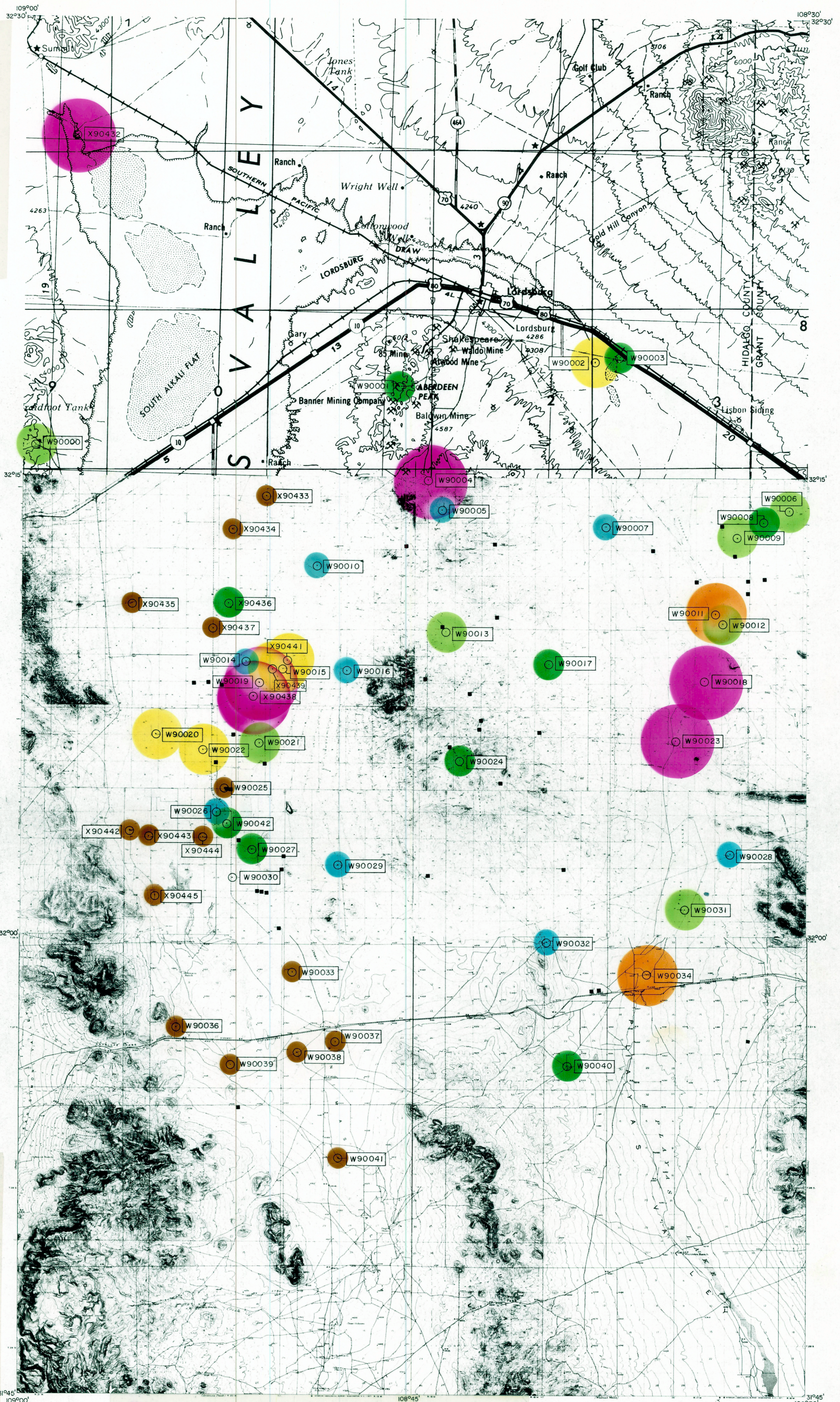
Chloride Distribution In mg/l Logarithmic Base
