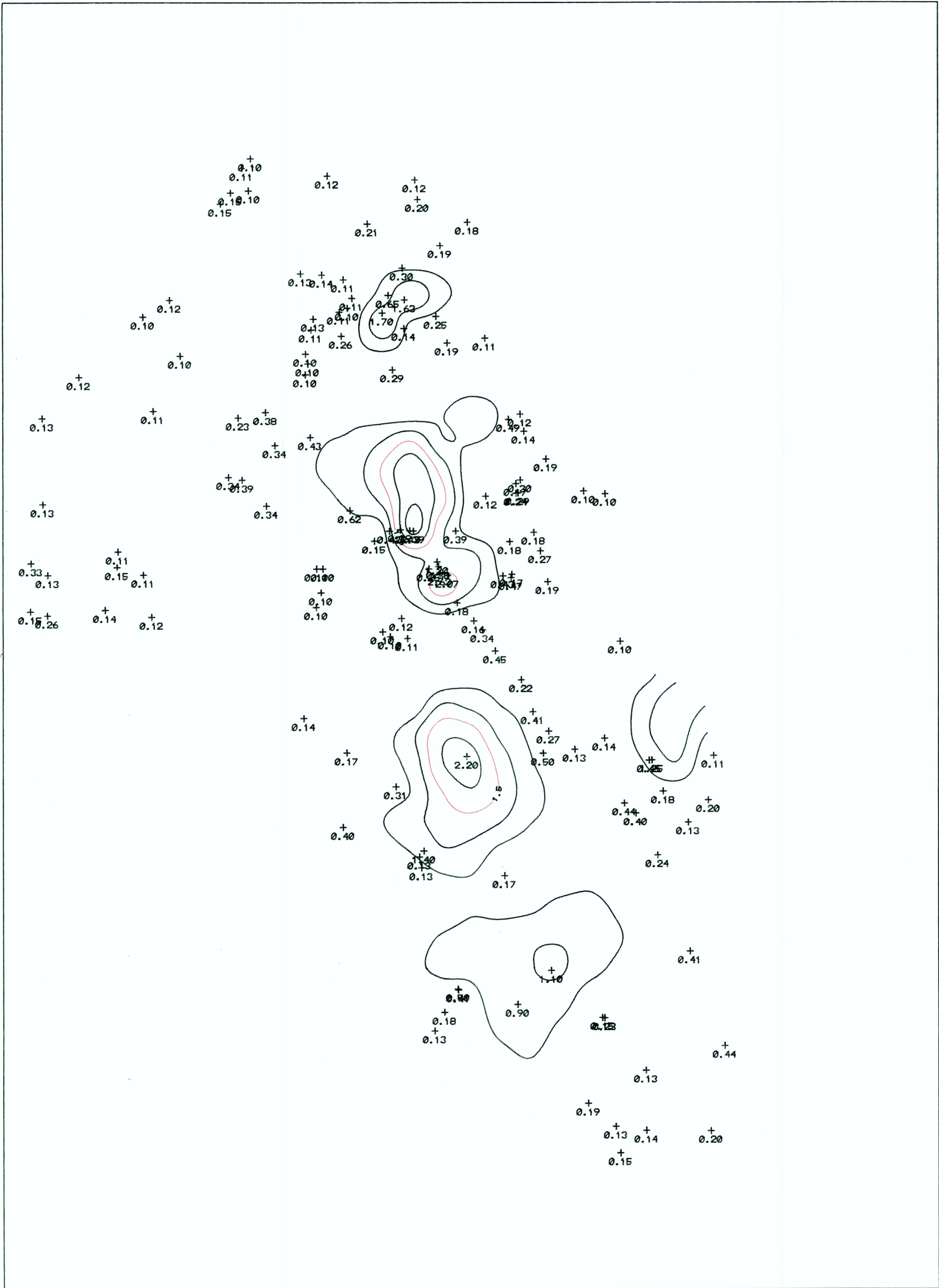
FLUORINE (F)
