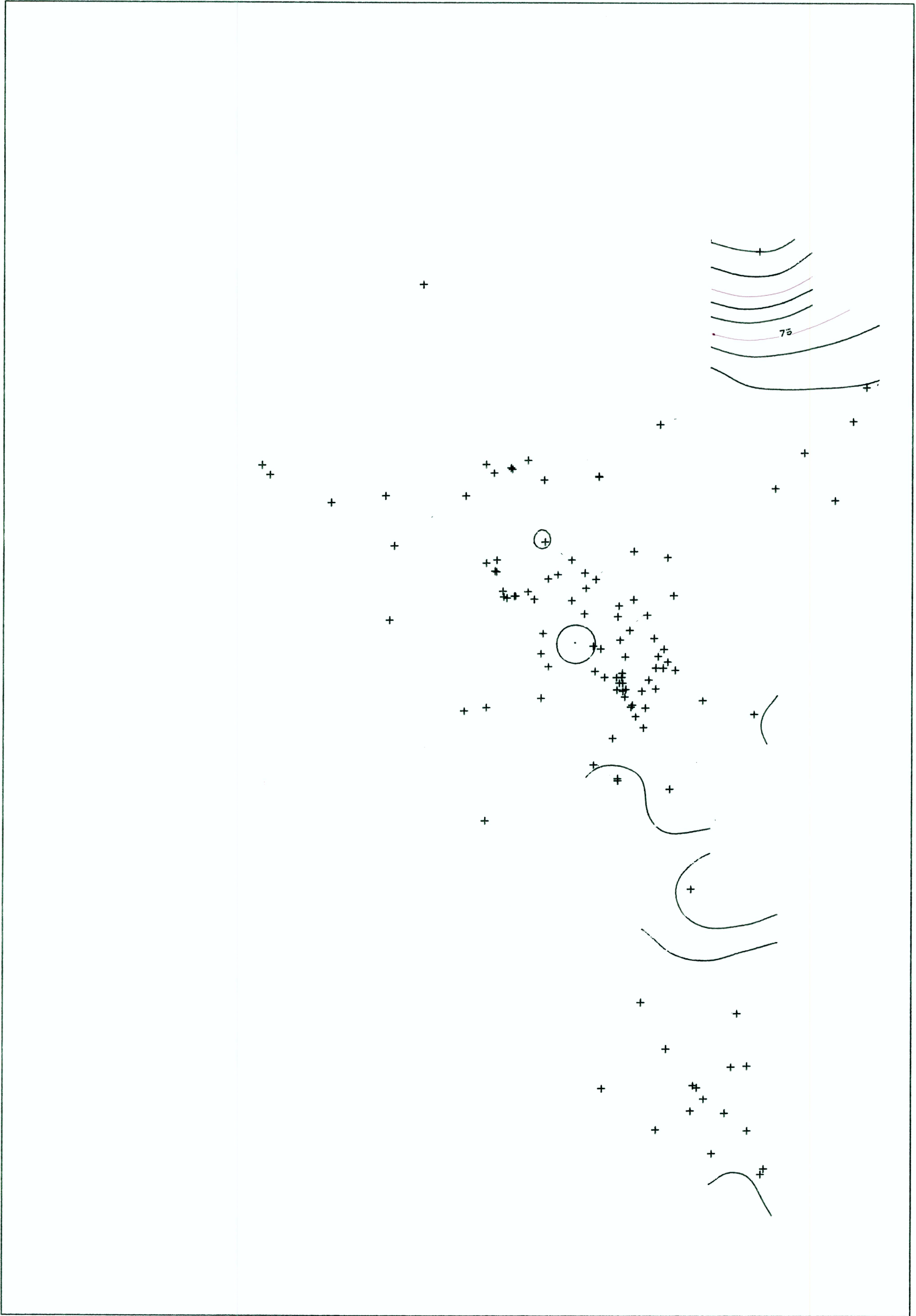
PLOT: (NA + K) / (CA + MG) REGION: MAYACMAS MOUNTAINS CONTOUR INTERVAL: 25.0
