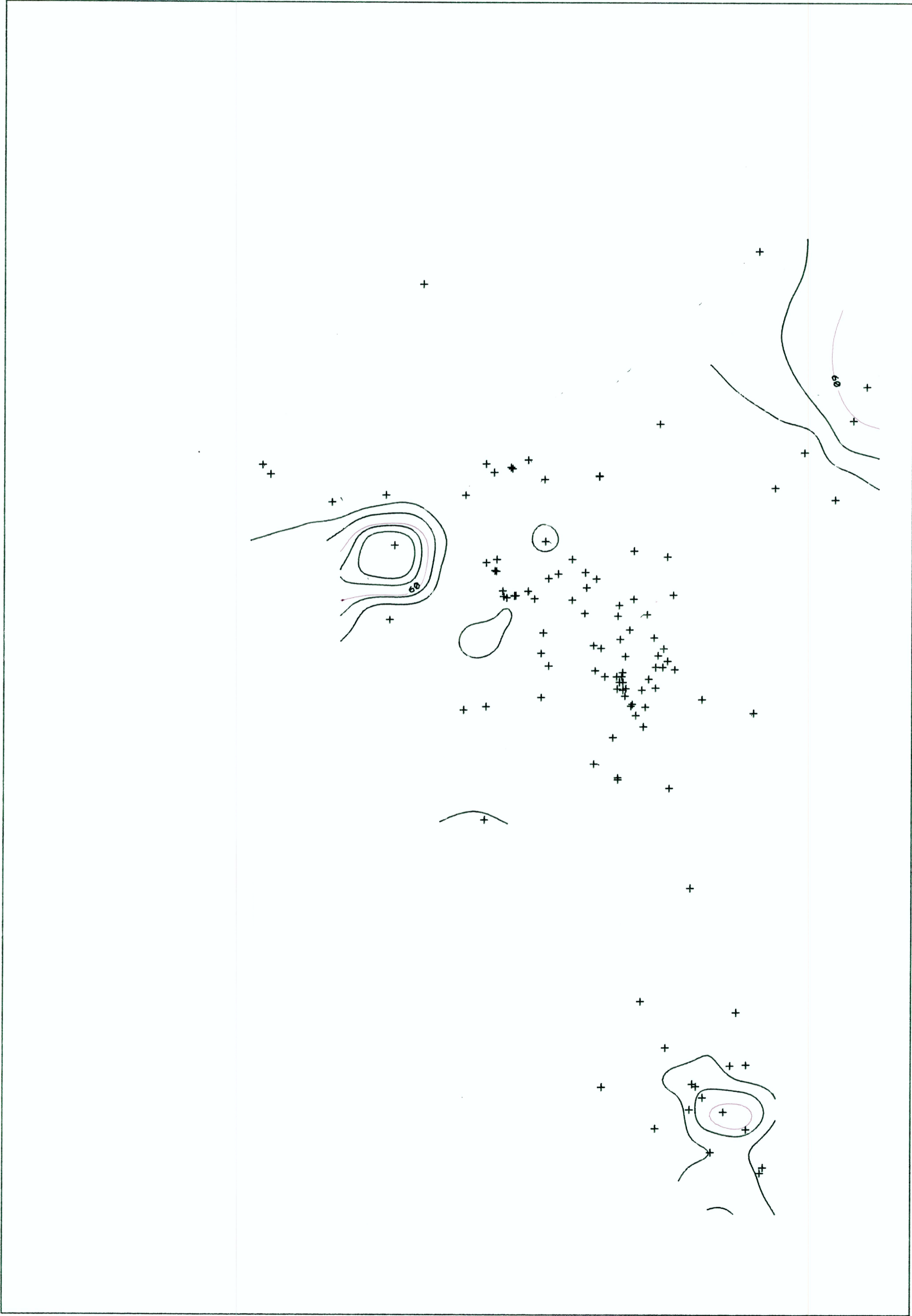
PLOT: CL / B REGION: MAYACMAS MOUNTAINS CONTOUR INTERVAL: 20.0
