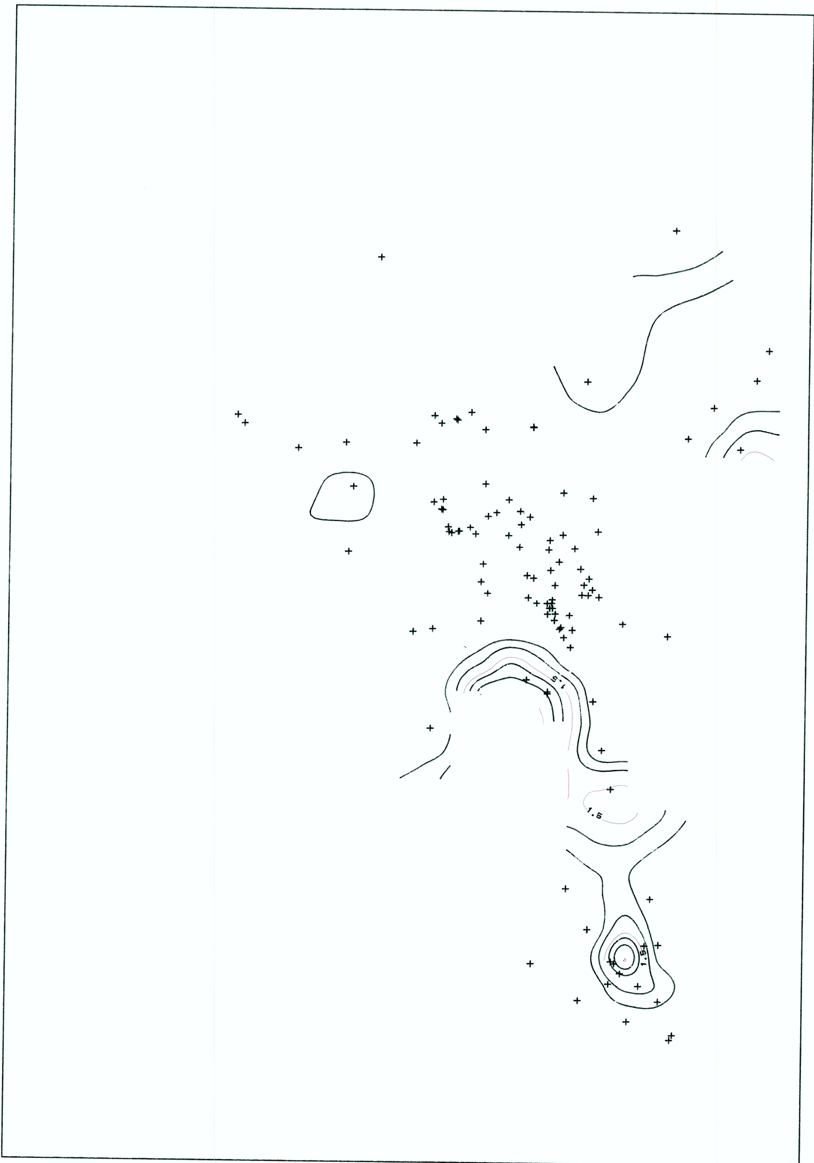
PLOT: CL / (HCO_3 + CO_3) REGION: MAYACMAS MOUNTAINS CONTOUR INTERVAL: 0.5
