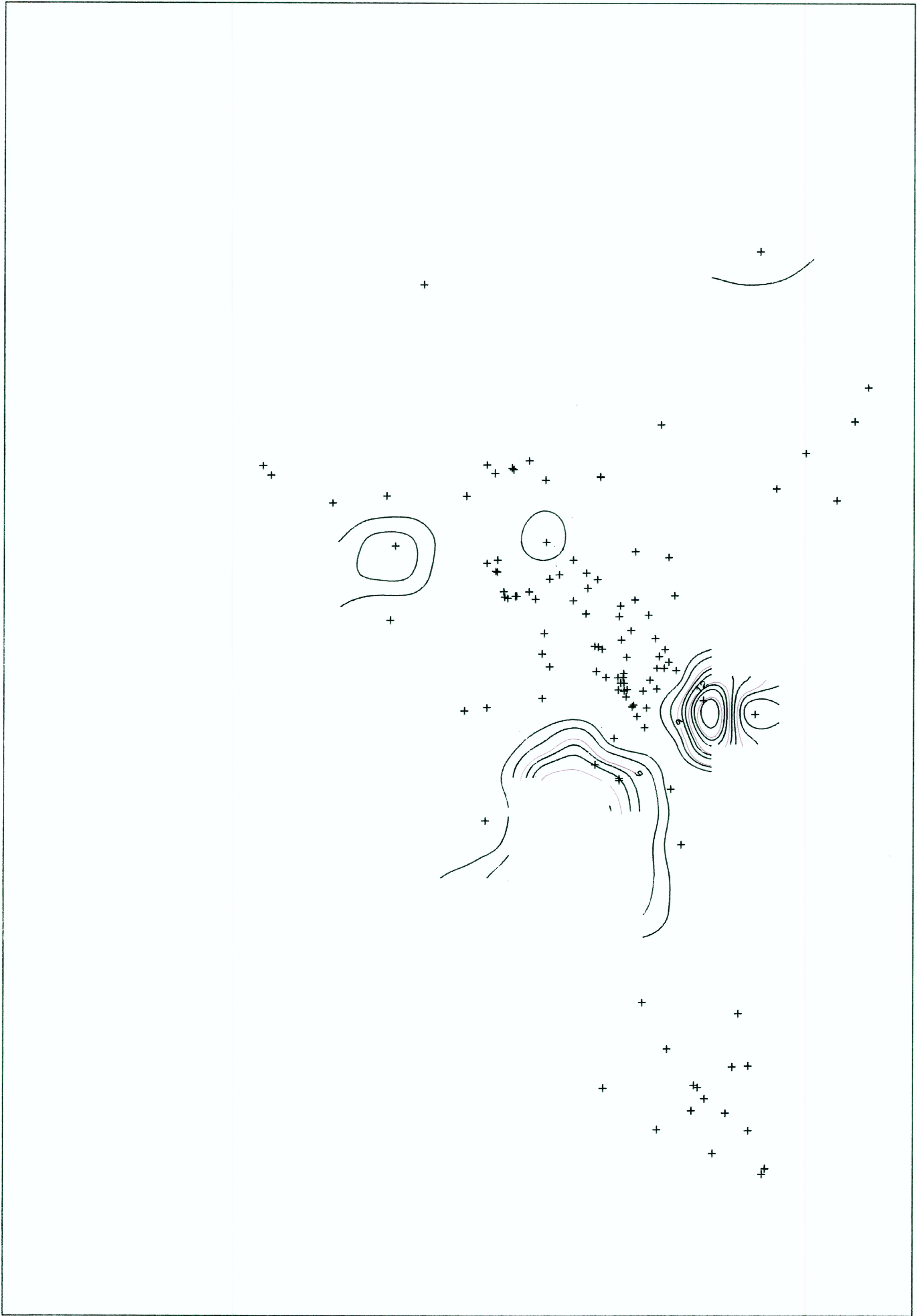
PLOT: FLUORINE (F) REGION: MAYACMAS MOUNTAINS CONTOUR INTERVAL: 2.0
