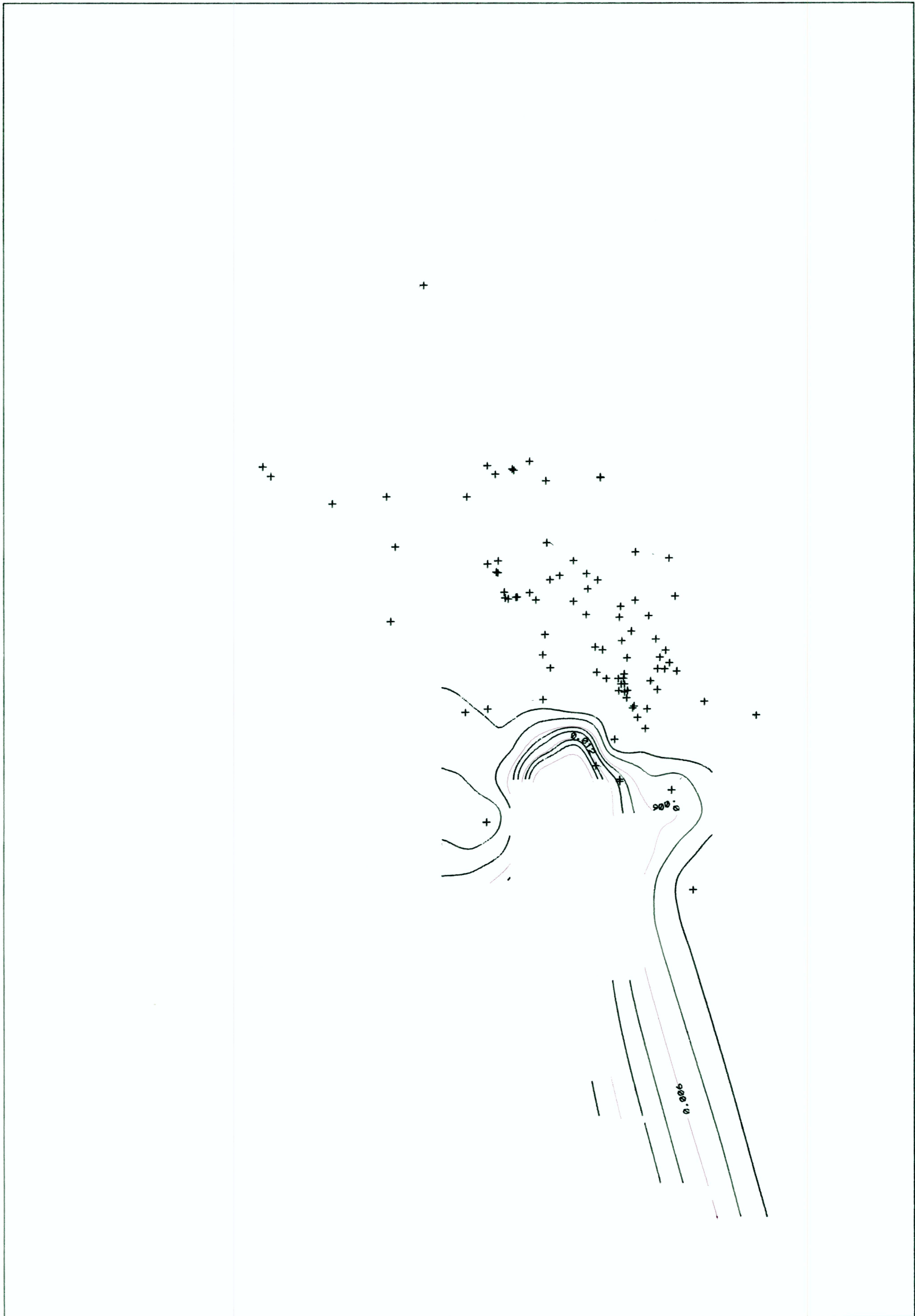
PLOT: MOLYBDENUM (MO) REGION: MAYACMAS MOUNTAINS CONTOUR INTERVAL: 0.002
