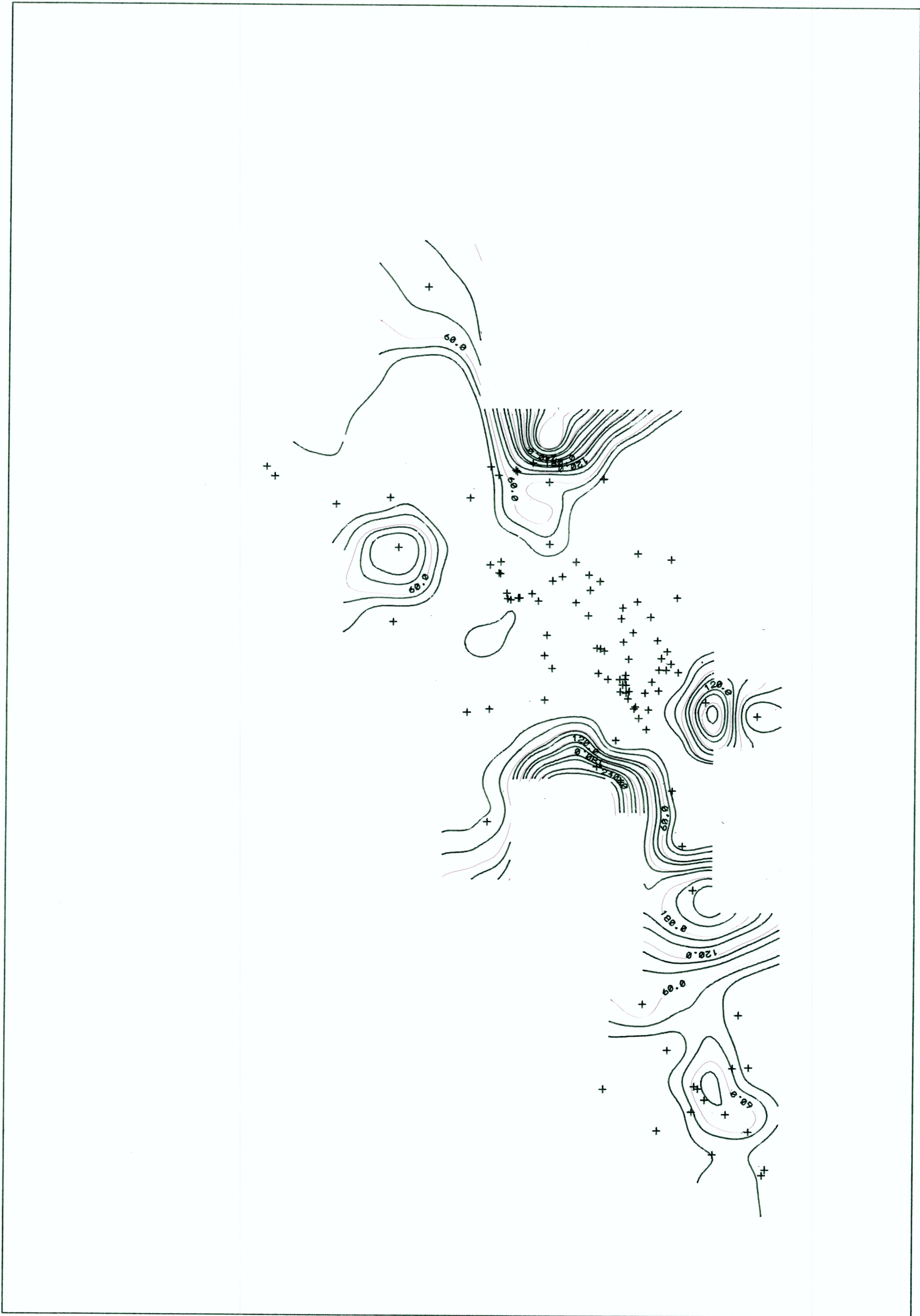
PLOT: CHLORINE (CL) REGION: MAYACMAS MOUNTAINS CONTOUR INTERVAL: 20.0
