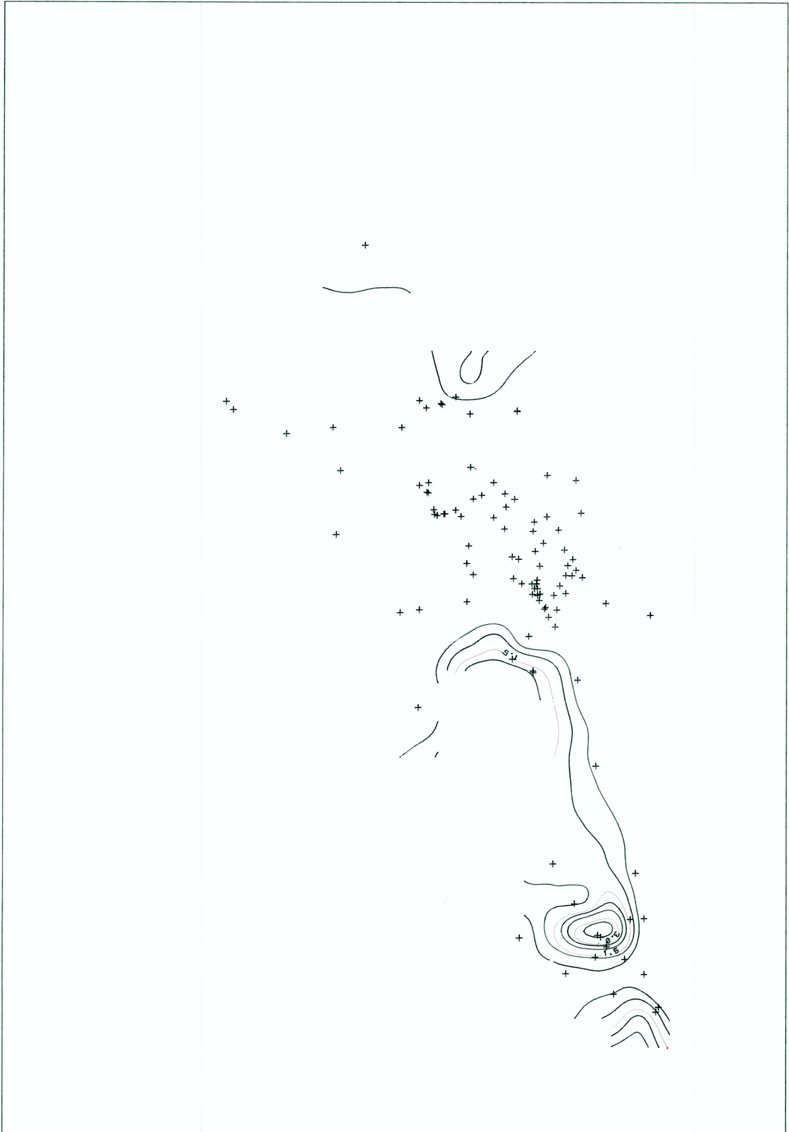
PLOT: LITHIUM (LI) REGION: MAYACMAS MOUNTAINS CONTOUR INTERVAL: .5
