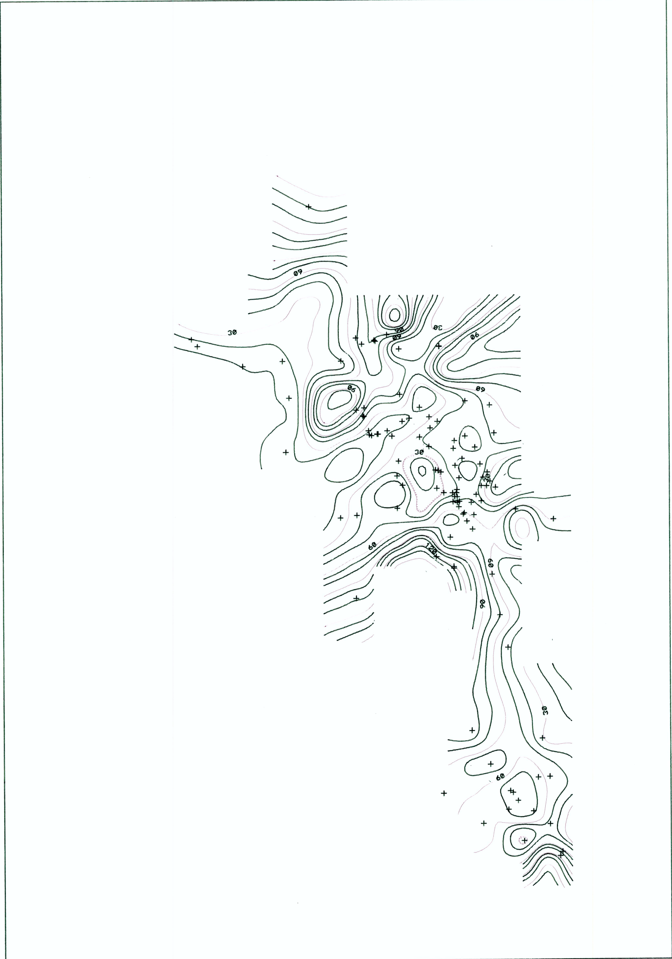
PLOT: SILICA (SI02) REGION: MAYACMAS MOUNTAINS CONTOUR INTERVAL: 10.0
