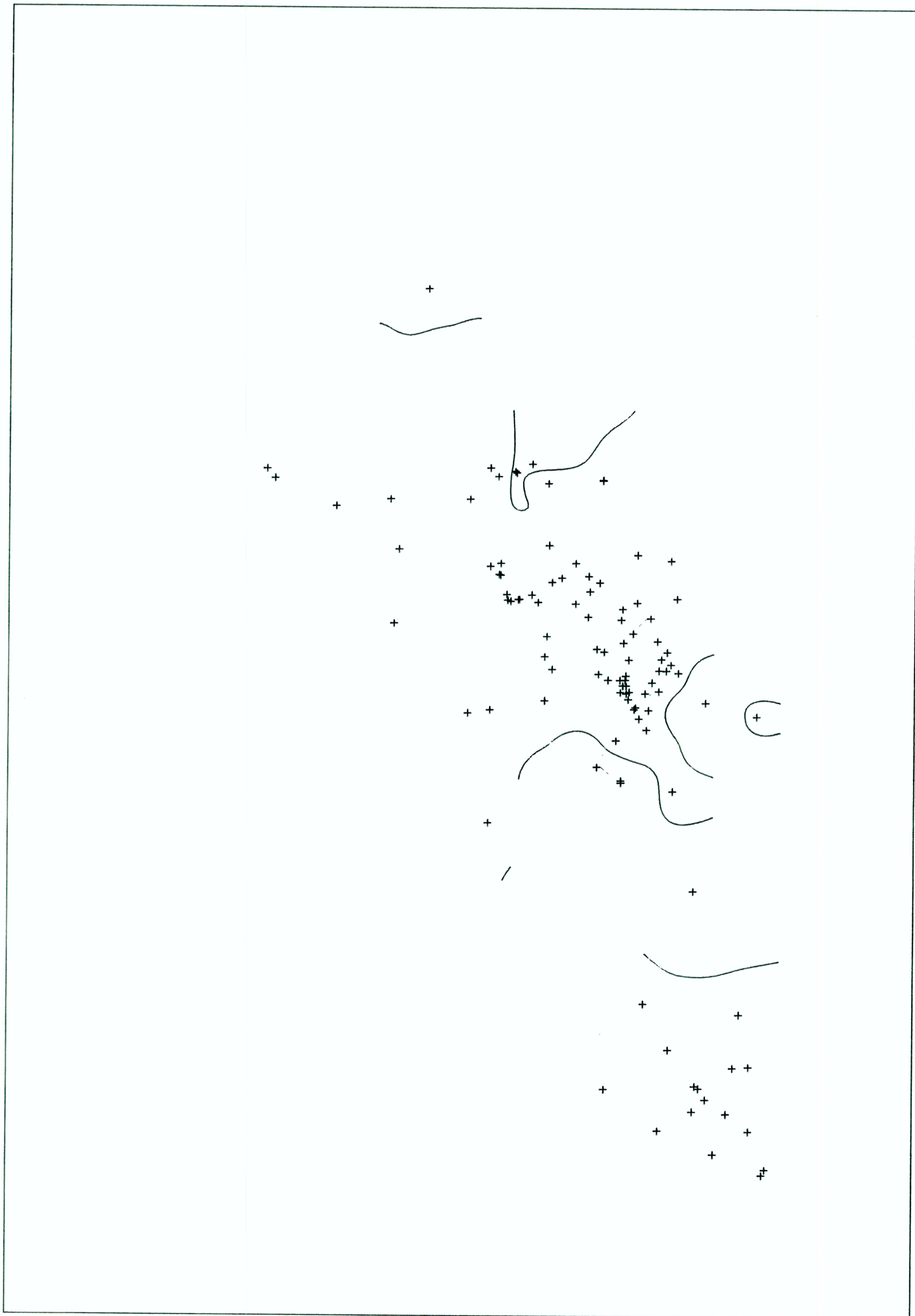
PLOT: BORON (B) REGION: MAYACMAS MOUNTAINS CONTOUR INTERVAL: 10.0
