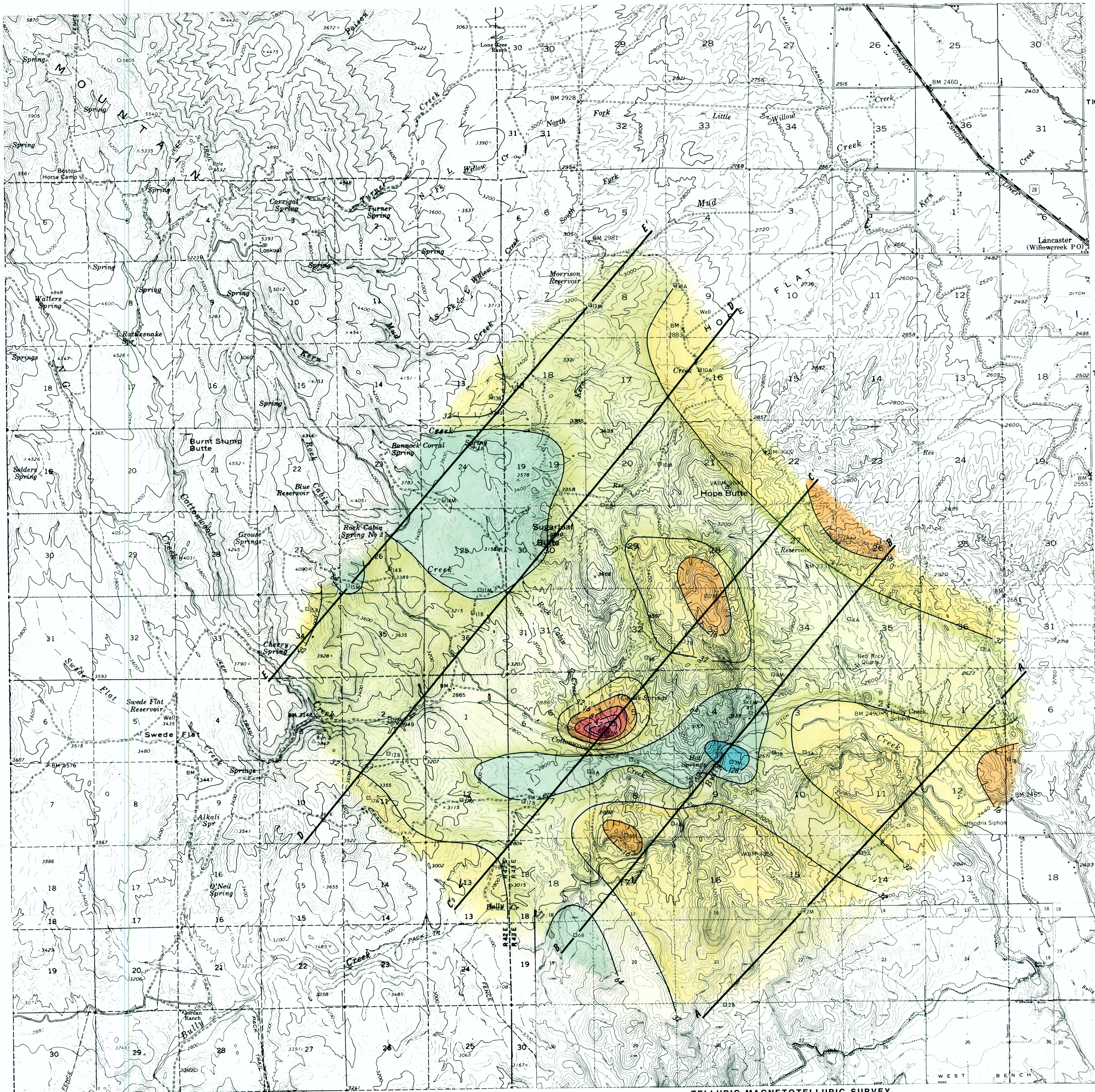
TELLURIC MAGNETOTELLURIC SURVEY Te-MODE I-D INVERSION DEPTH 3 km RESISTIVITY IN ΩM SCALE 1:24,000
