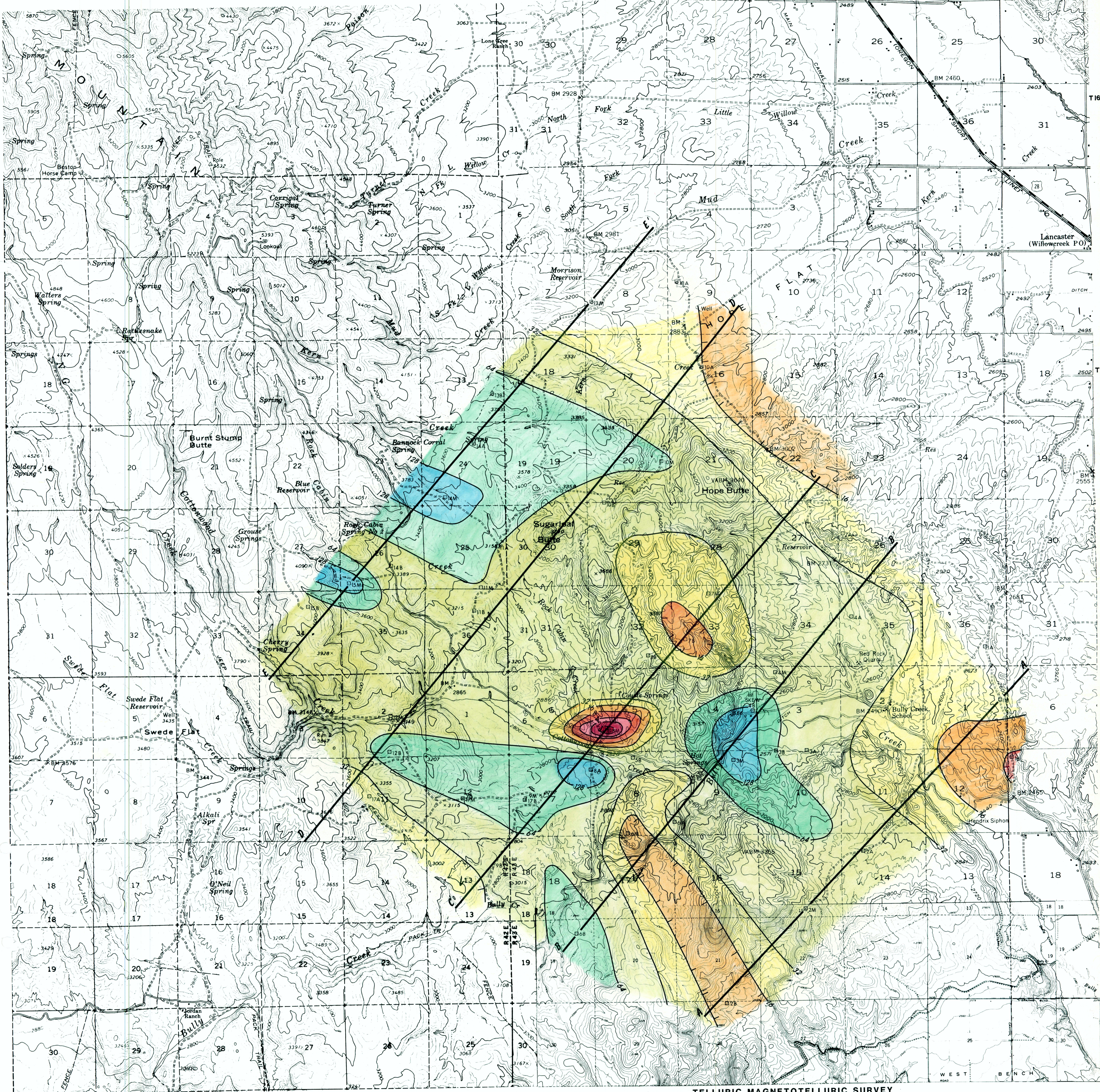
TELLURIC MAGNETOTELLURIC SURVEY Te-MODE I-D INVERSION DEPTH 5 km RESISTIVITY IN \Omega m
