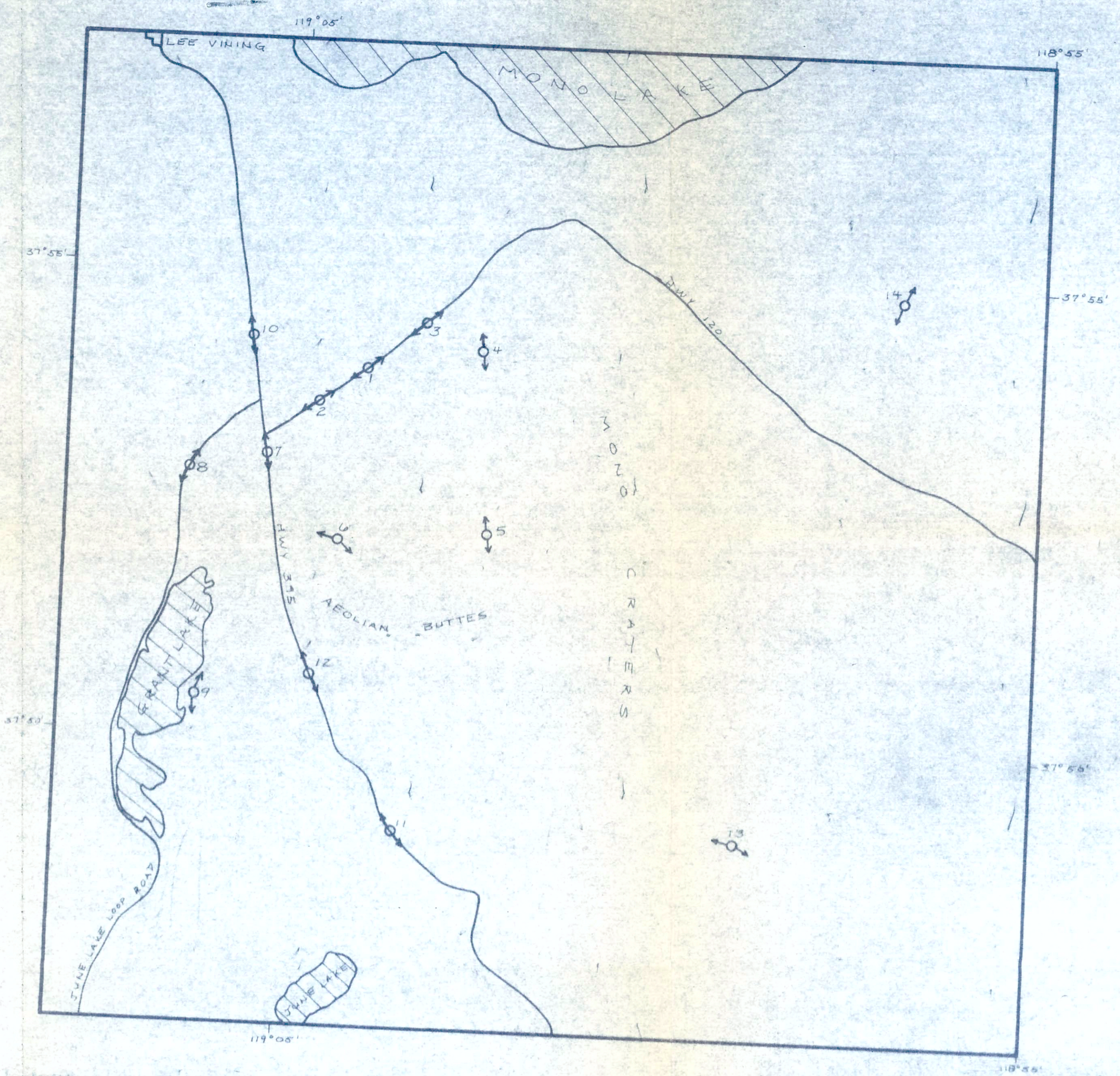
Plate 1 - Location map for Schlumberger soundings in the Aeolian Buttes area. Circles mark sounding location and arrows indicate direction of sounding expansion.
