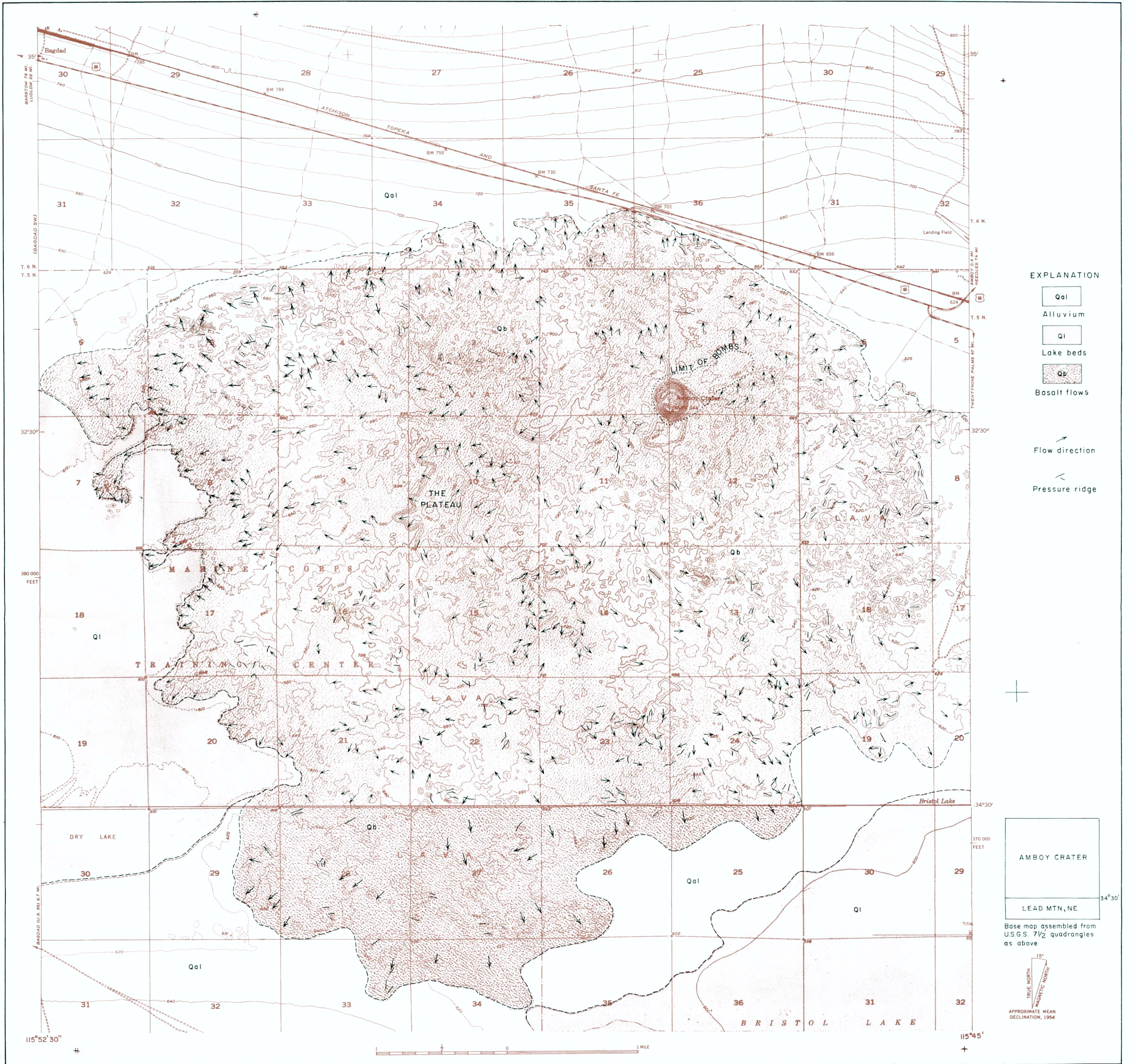
MAP OF AMBOY CRATER AREA BASALT FLOWS SAN BERNARDINO COUNTY, CALIFORNIA
