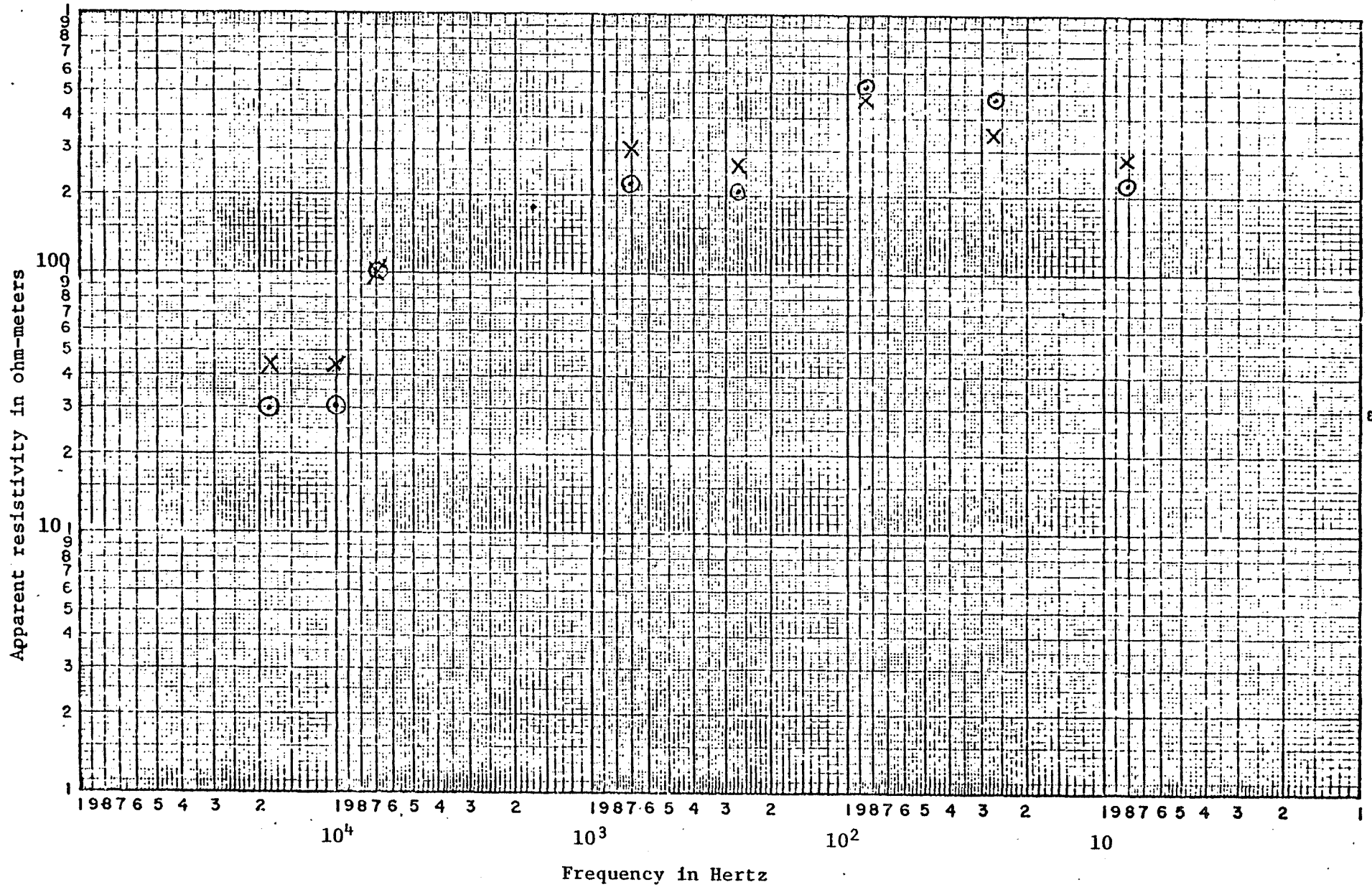
Figure 2. AMT sounding, Long Valley #1. x, electric line east, ⊙, electric line south.
