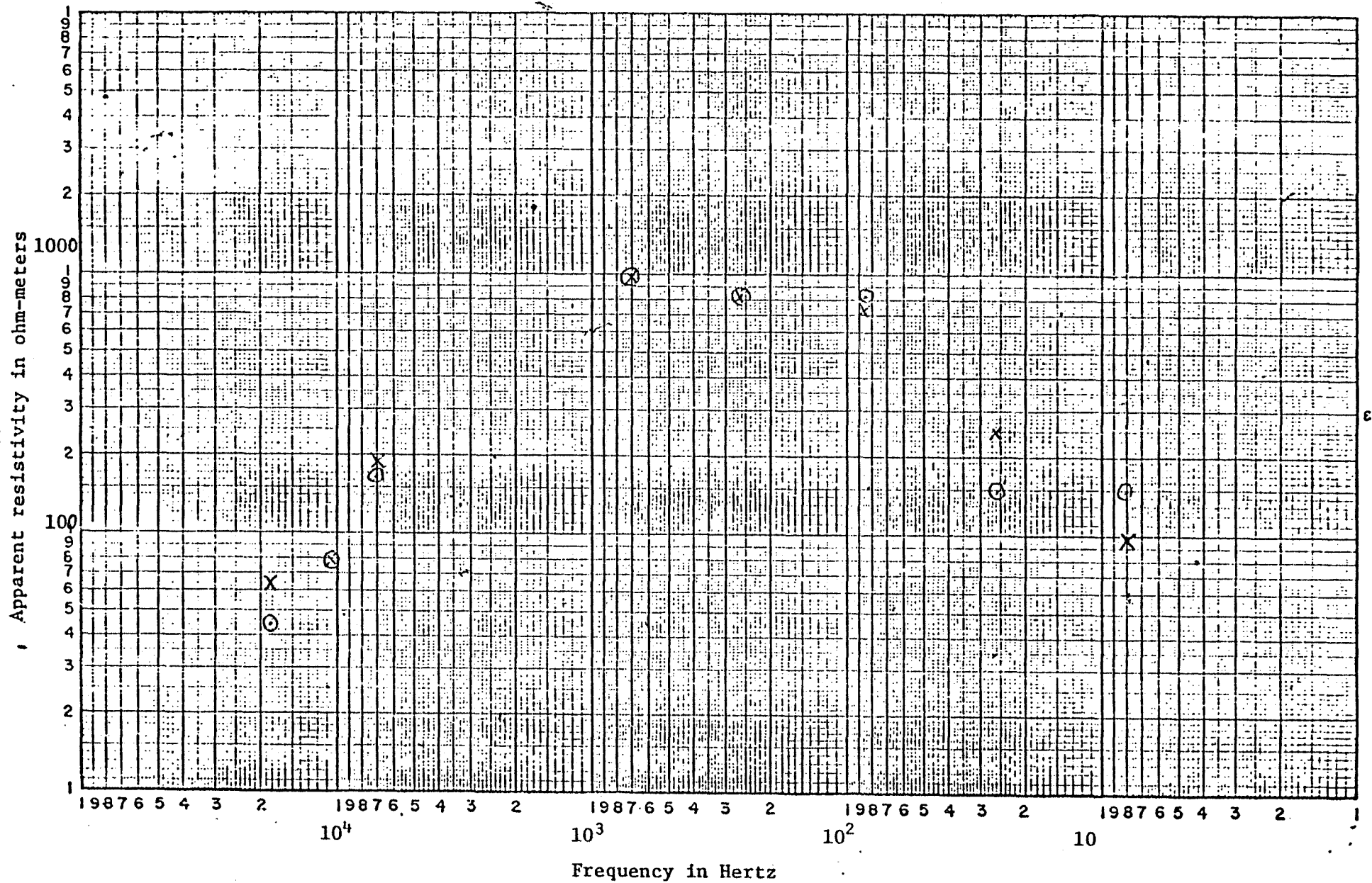
Figure 21. AMT sounding, Long Valley #26. x, electric line west, O electric line north.
