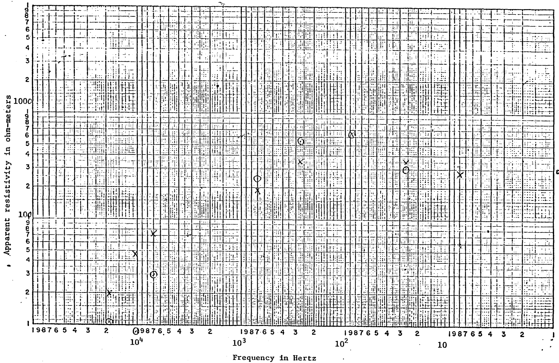
Figure 25. AMT sounding, Long Valley #30. x, electric line east, O, electric line south.
