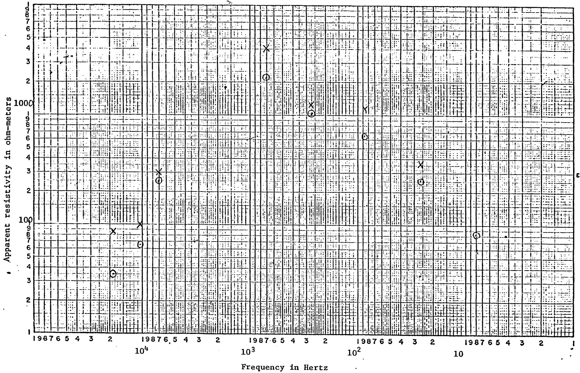
Figure 13. AMT sounding, Long Valley #18. x, electric line east, O electric line north.
