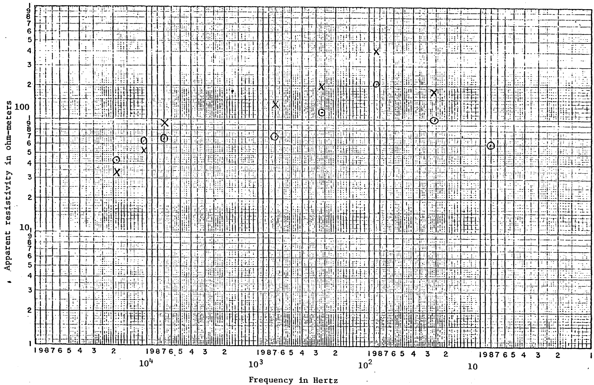
Figure 24. AMT sounding, Long Valley #29. x, electric line west, O electric line south.
