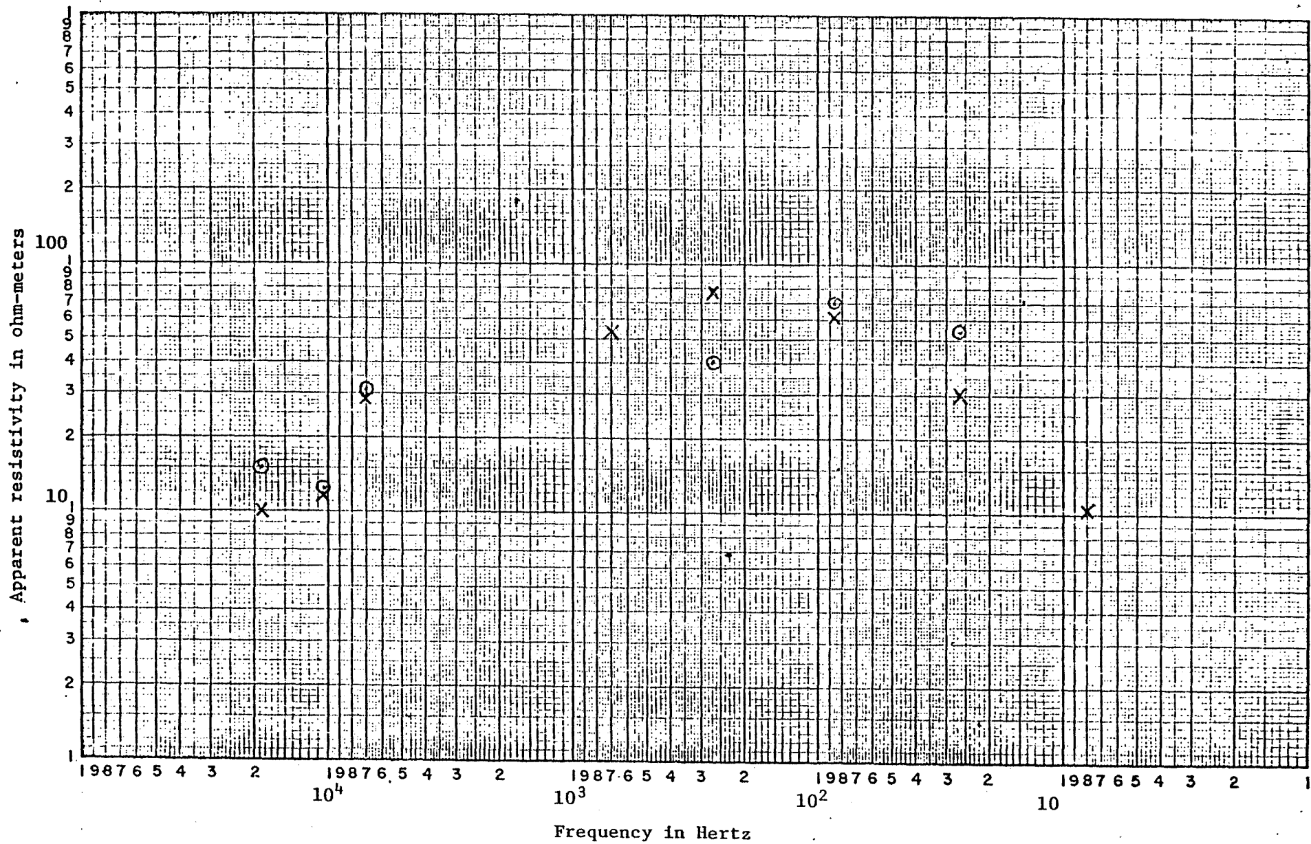
Figure 7. AMT sounding, Long Valley #6. x, electric line east, ⊙ electric line south.
