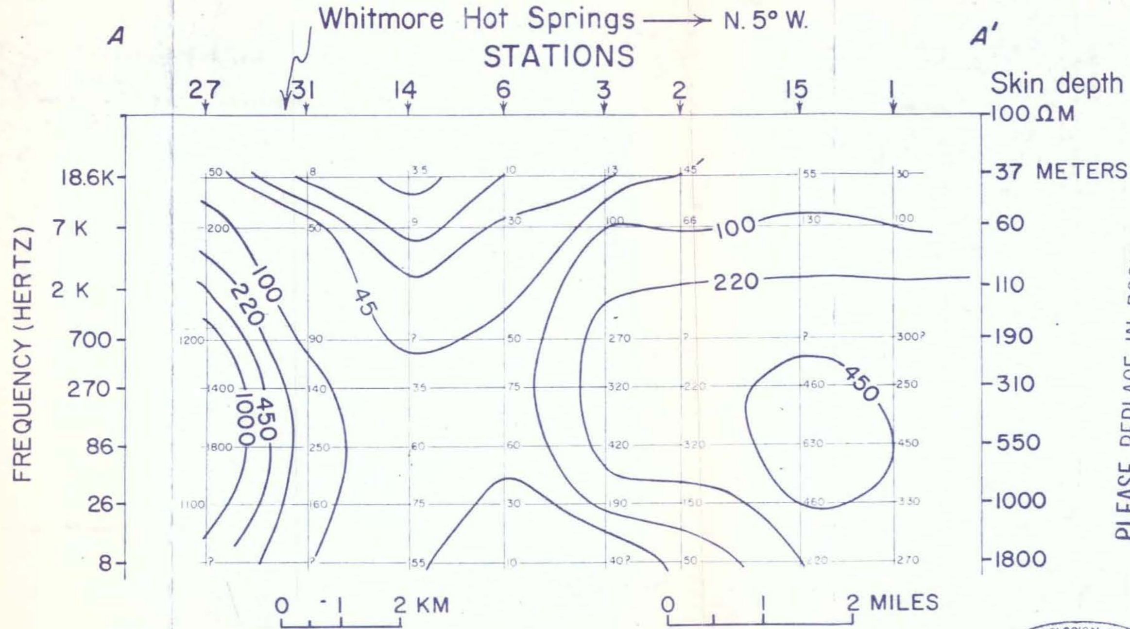
AMT PSEUDOSECTION ALONG A-A' (ELECTRIC LINE E-W) LONG VALLEY, CALIF. PLATE 8
