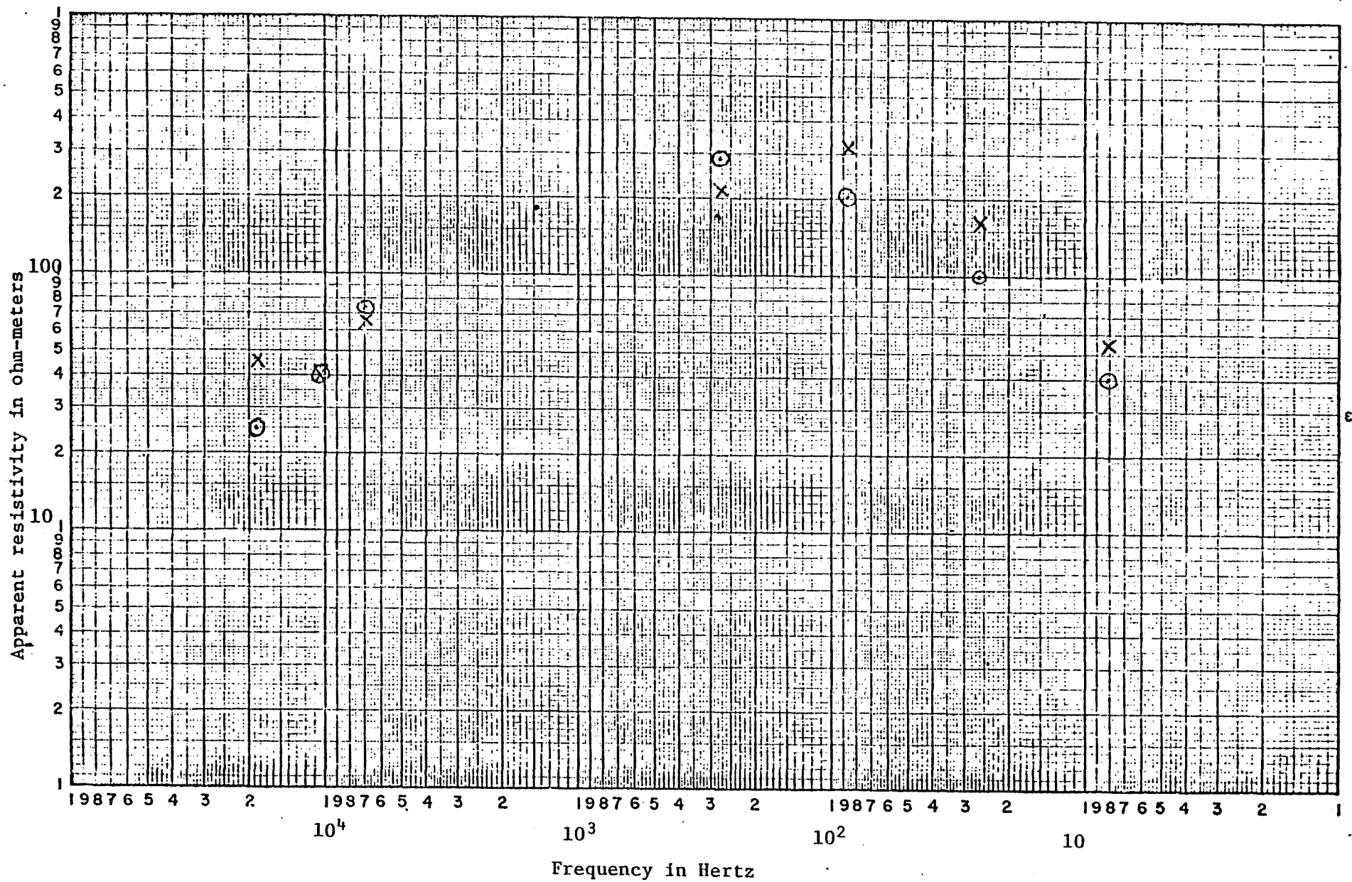
Figure 3. AMT sounding, Long Valley #2. x, electric line west, ⊗, electric line north.
