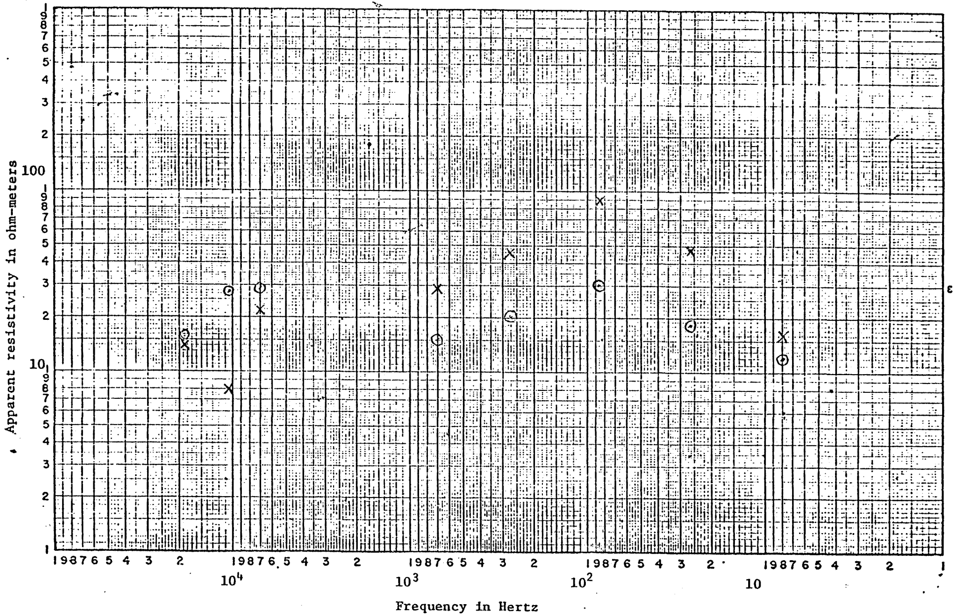
Figure 11. AMT sounding, Long Valley #16. x, electric line west, ⊙, electric line north.
