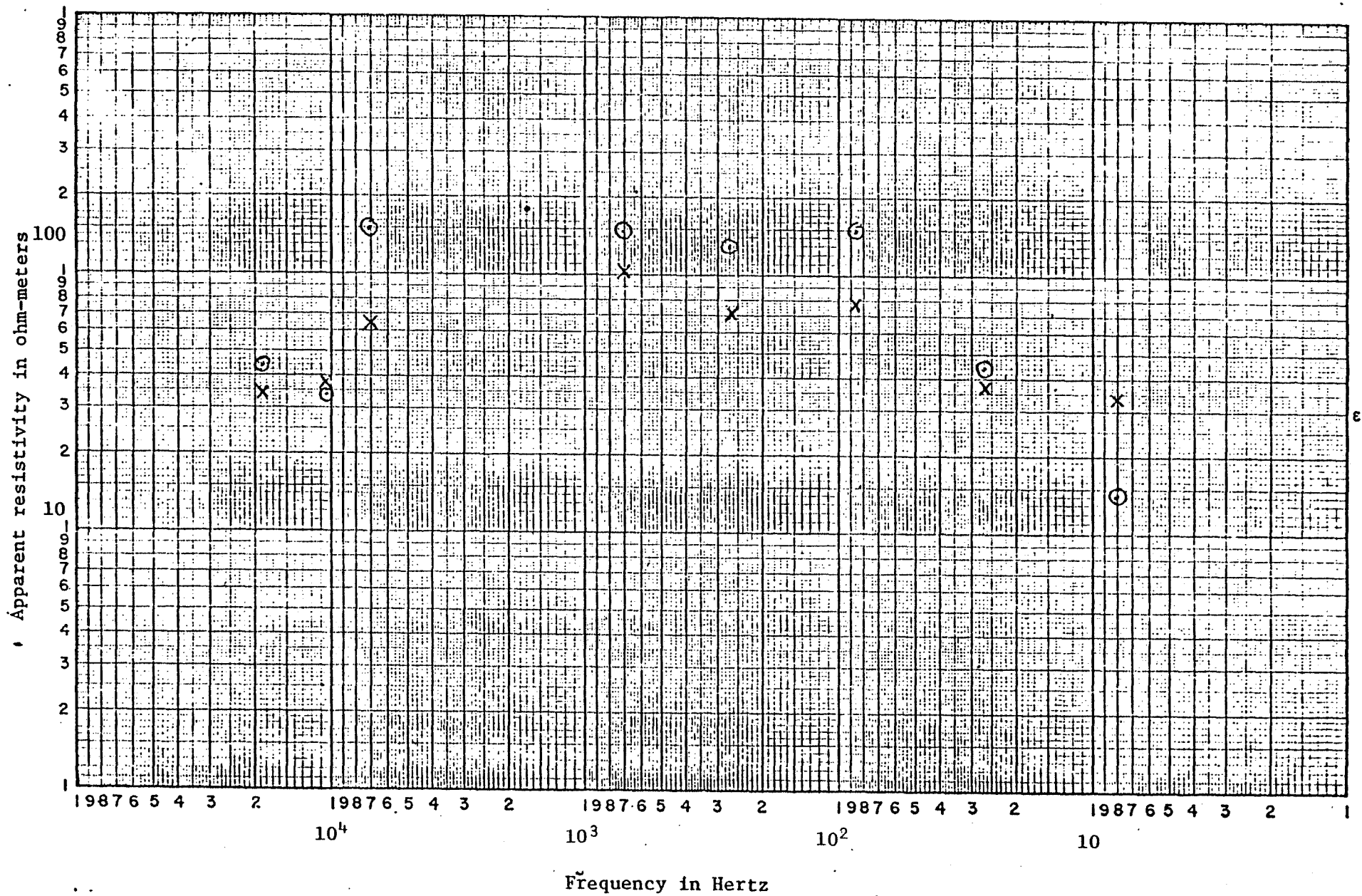
Figure 6. AMT sounding, Long Valley #5. x, electric line east, O, electric line south.
