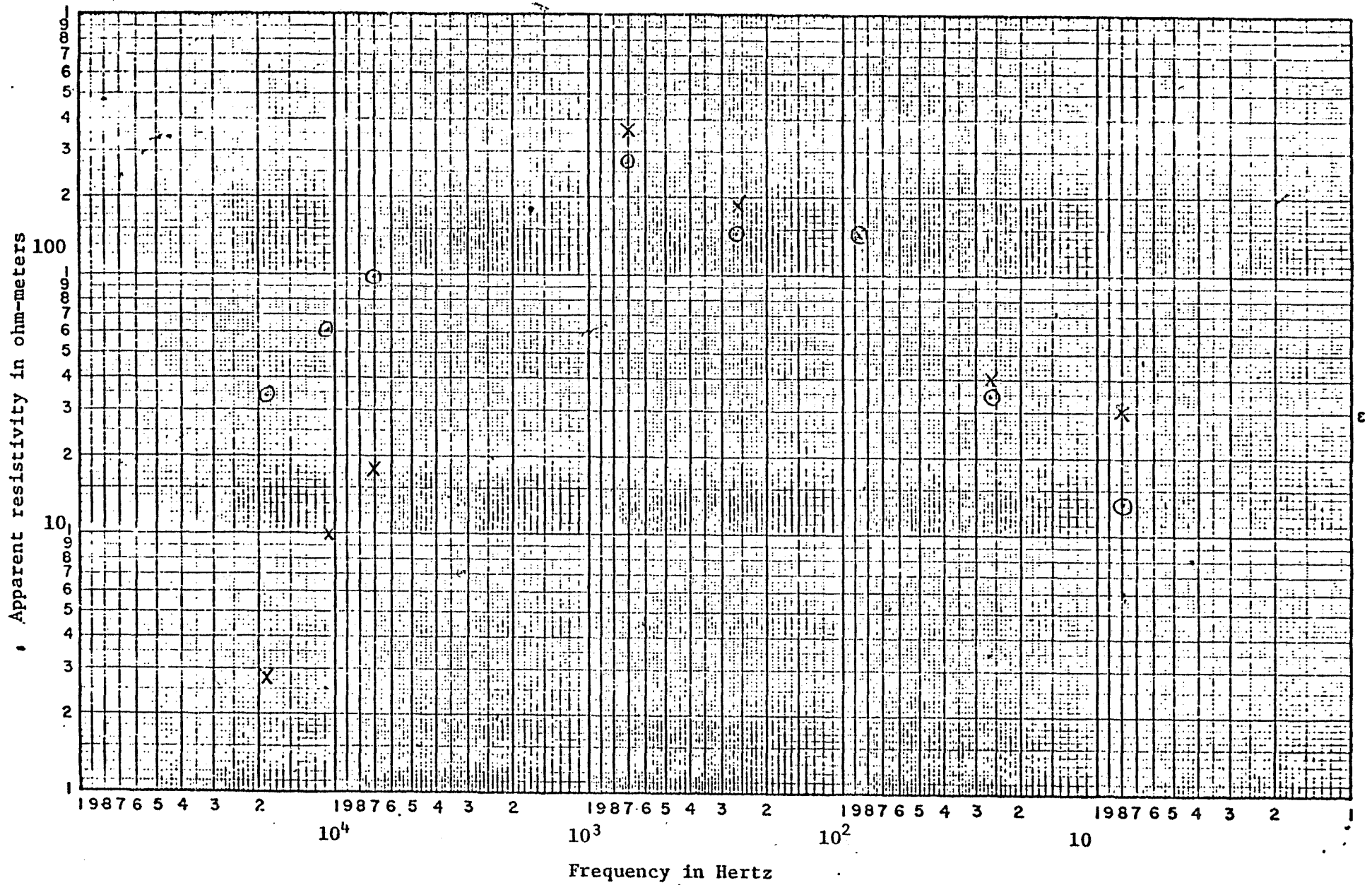
Figure 20. AMT sounding, Long Valley #25. x, electric line east, O electric line north.
