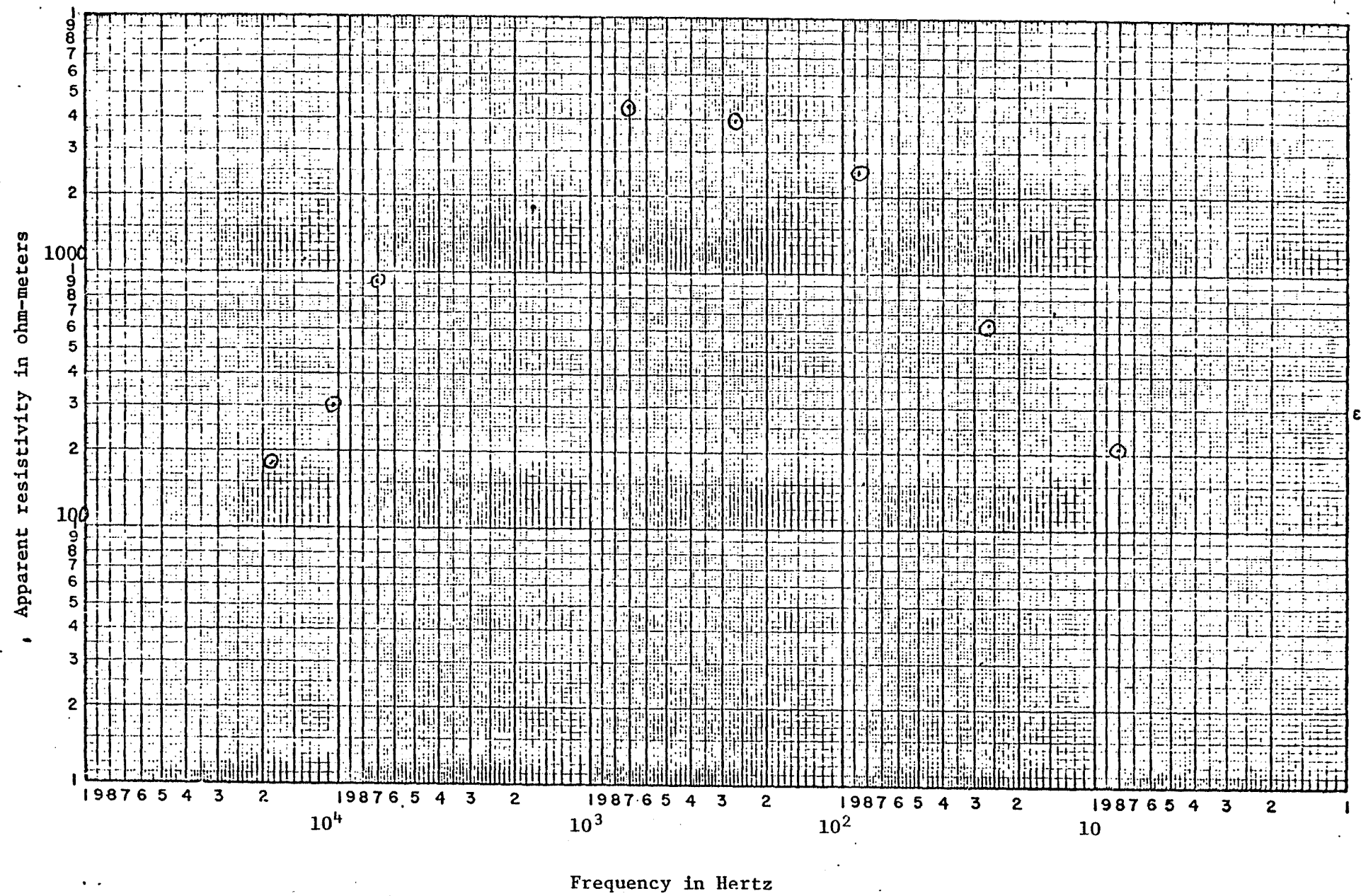
Figure 14. AMT sounding, Long Valley #19. ⊗ electric line north.
