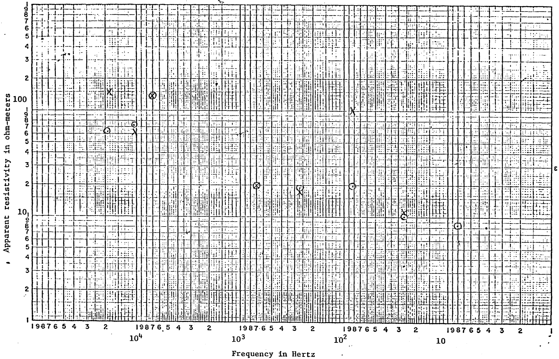
Figure 23. AMT sounding, Long Valley #28. x, electric line west, O electric line north.
