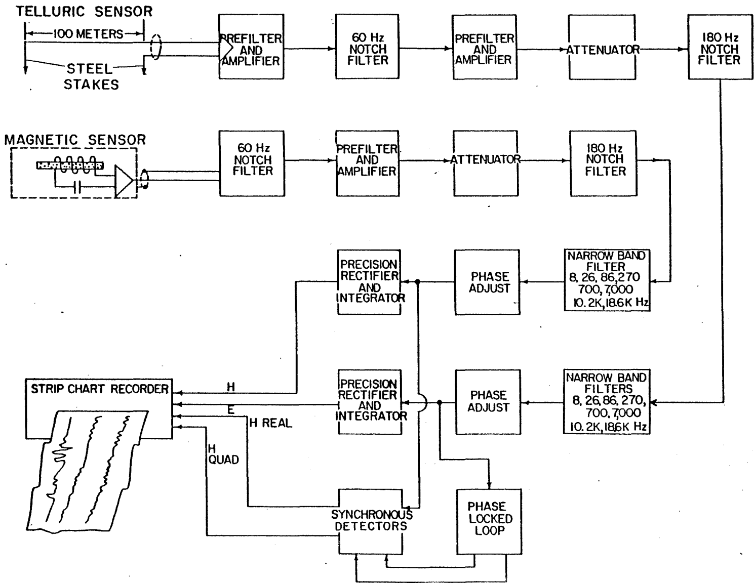
Figure 1.--USGS audio-magnetotelluric (AMT) system.
