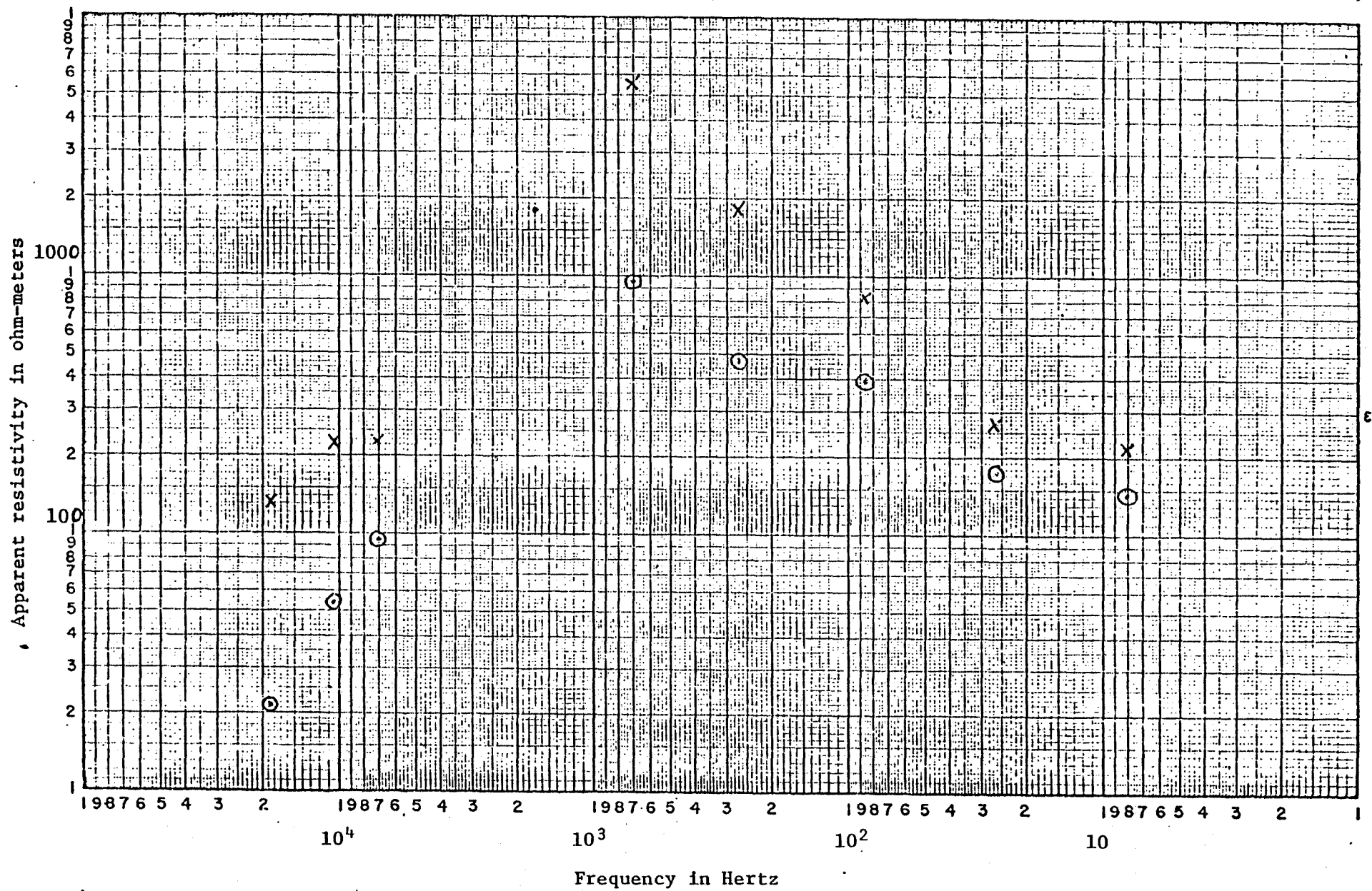
Figure 8. AMT sounding, Long Valley #13. x, electric line east, o electric line north.
