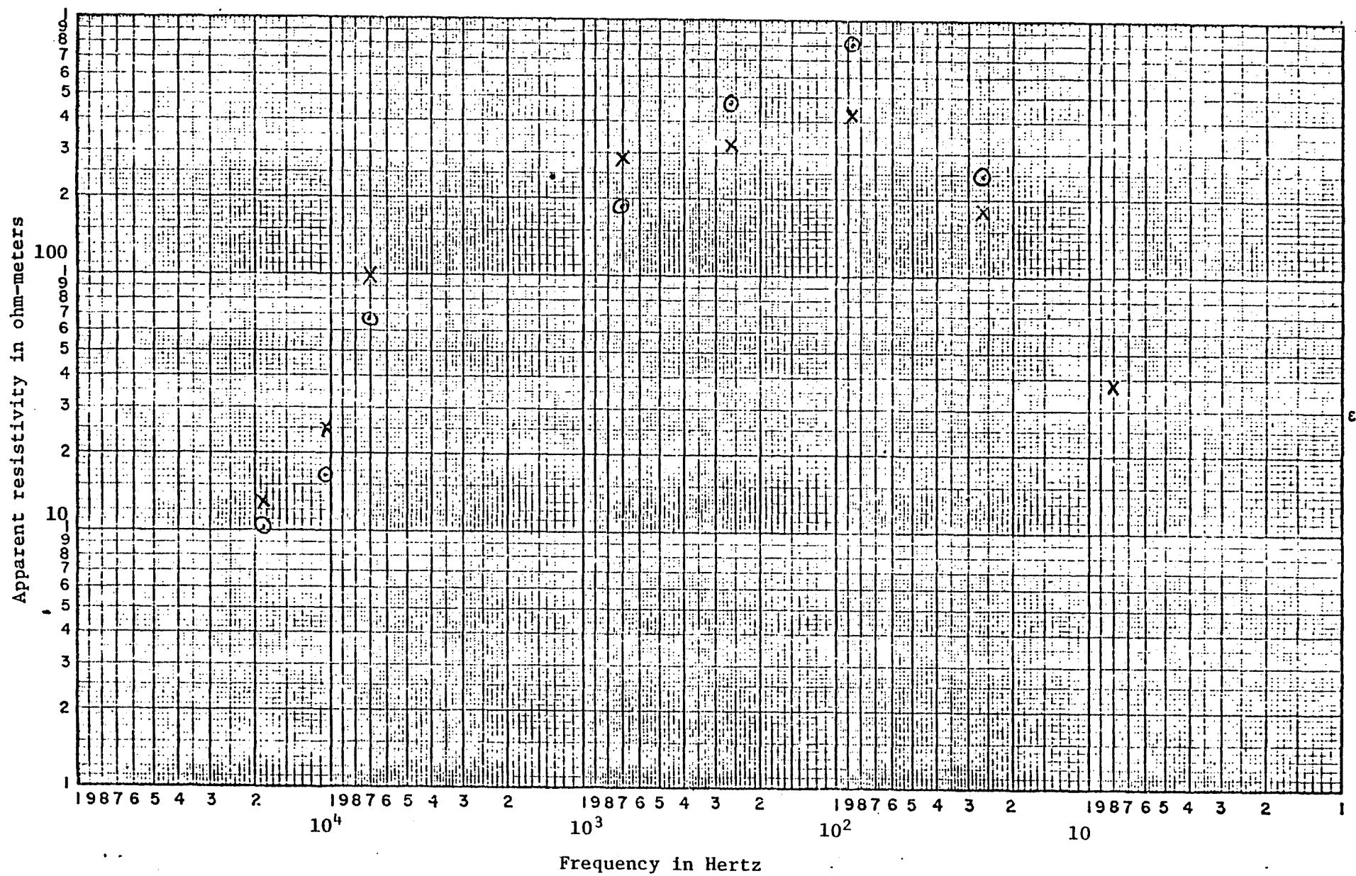
Figure 4. AMT sounding, Long Valley #3. x, electric line east, ⊙, electric line south.
