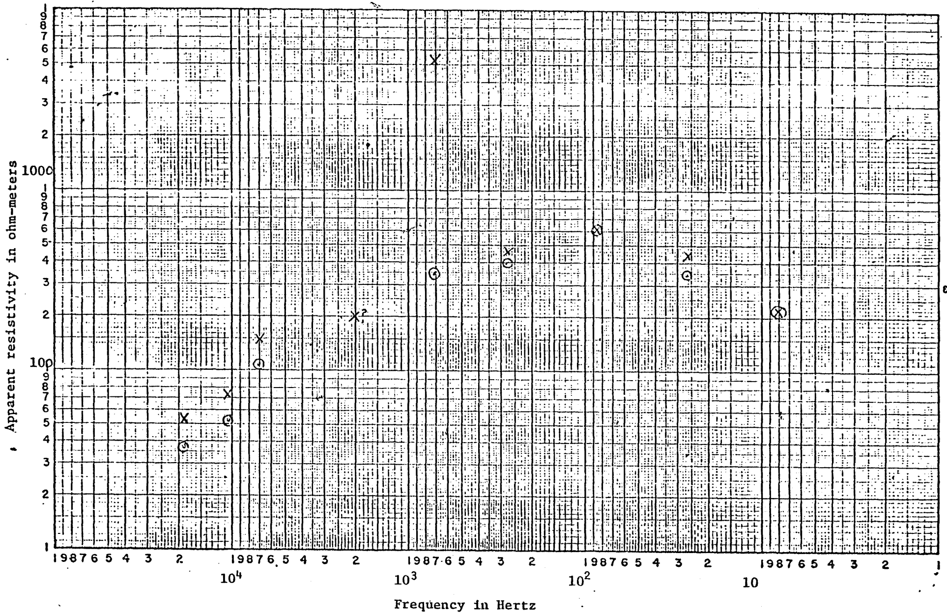
Figure 10. AMT sounding, Long Valley #15. x, electric line east, o, electric line south.
