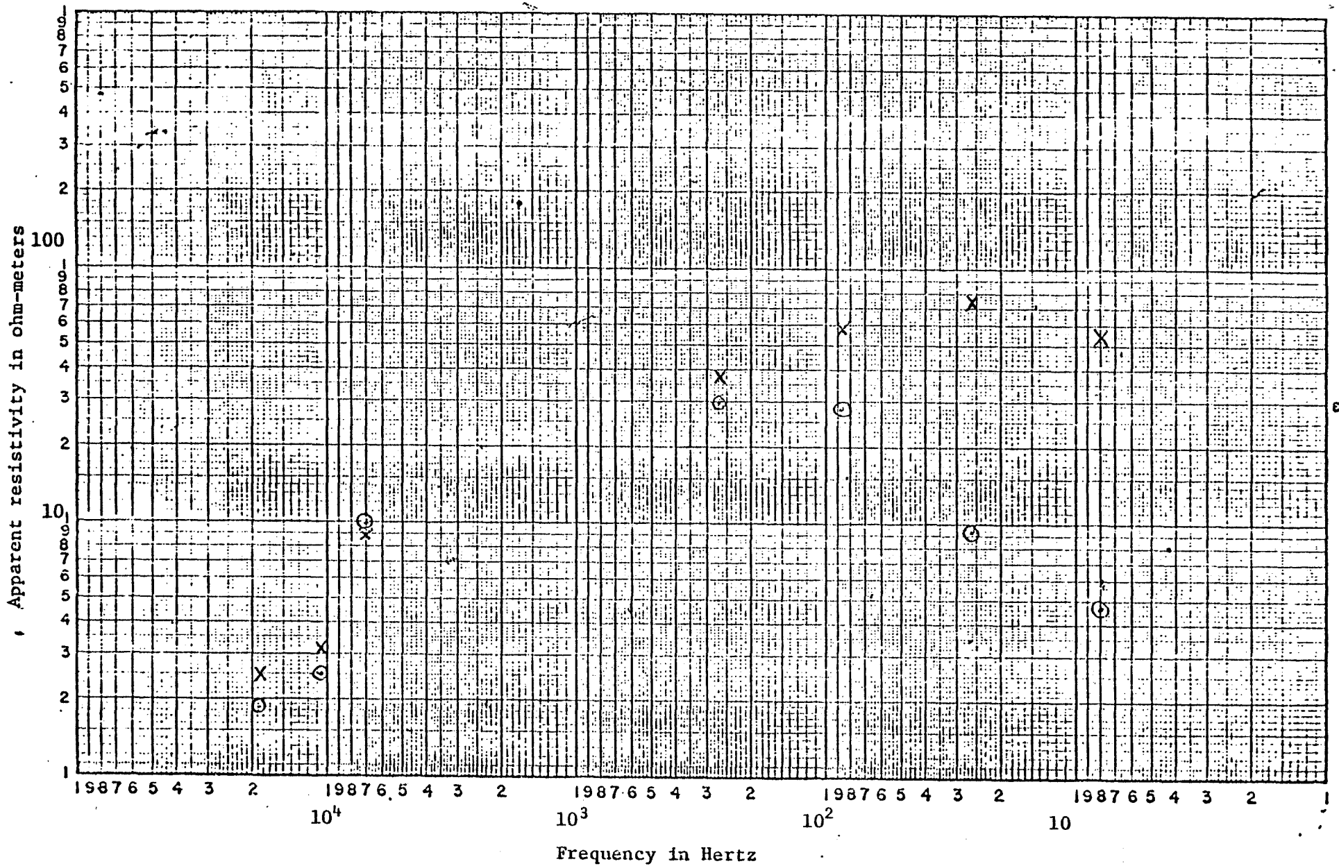
Figure 9. AMT sounding, Long Valley #14. x, electric line east, o, electric line south.
