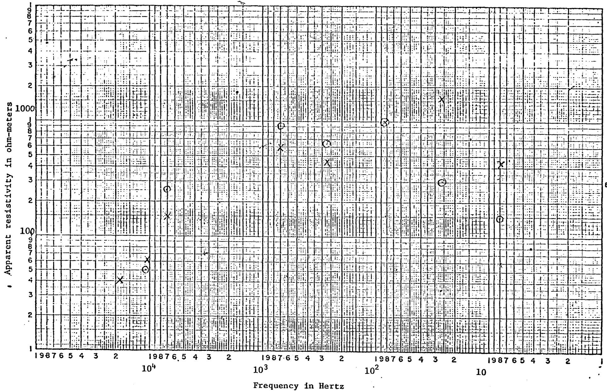
Figure 18 -- AMT sounding, Long Valley #23. x, electric line east, O electric line south.
