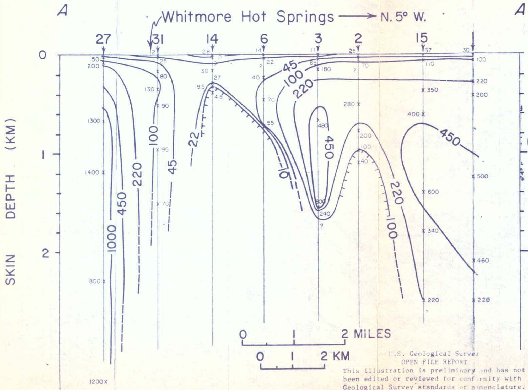
SKIN-DEPTH PSEUDOSECTION ALONG A-A' (ELECTRIC LINE N-S) LONG VALLEY, CALIF. PLATE II
