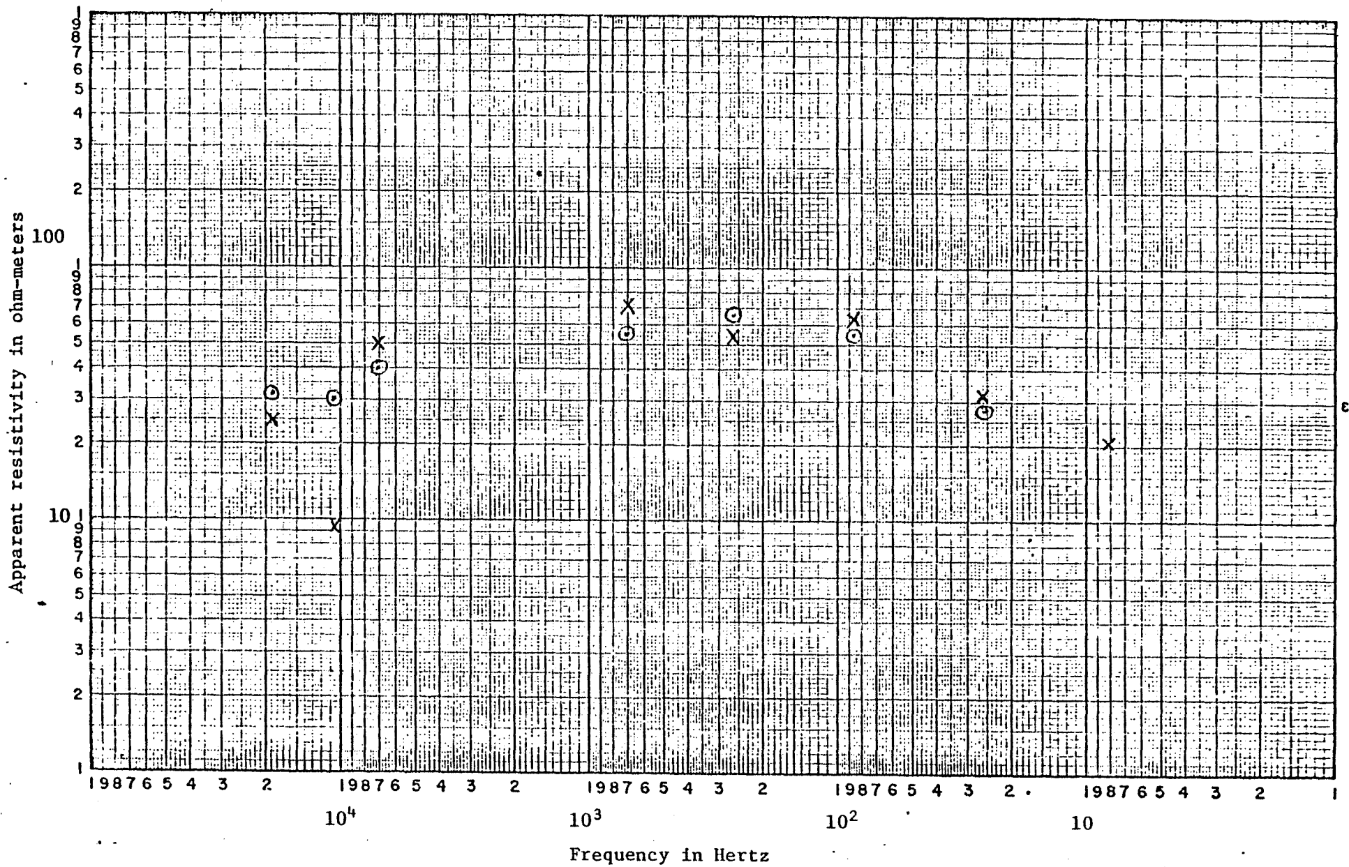
Figure 5. AMT sounding, Long Valley #4. x, electric line west, ⊙, electric line south.
