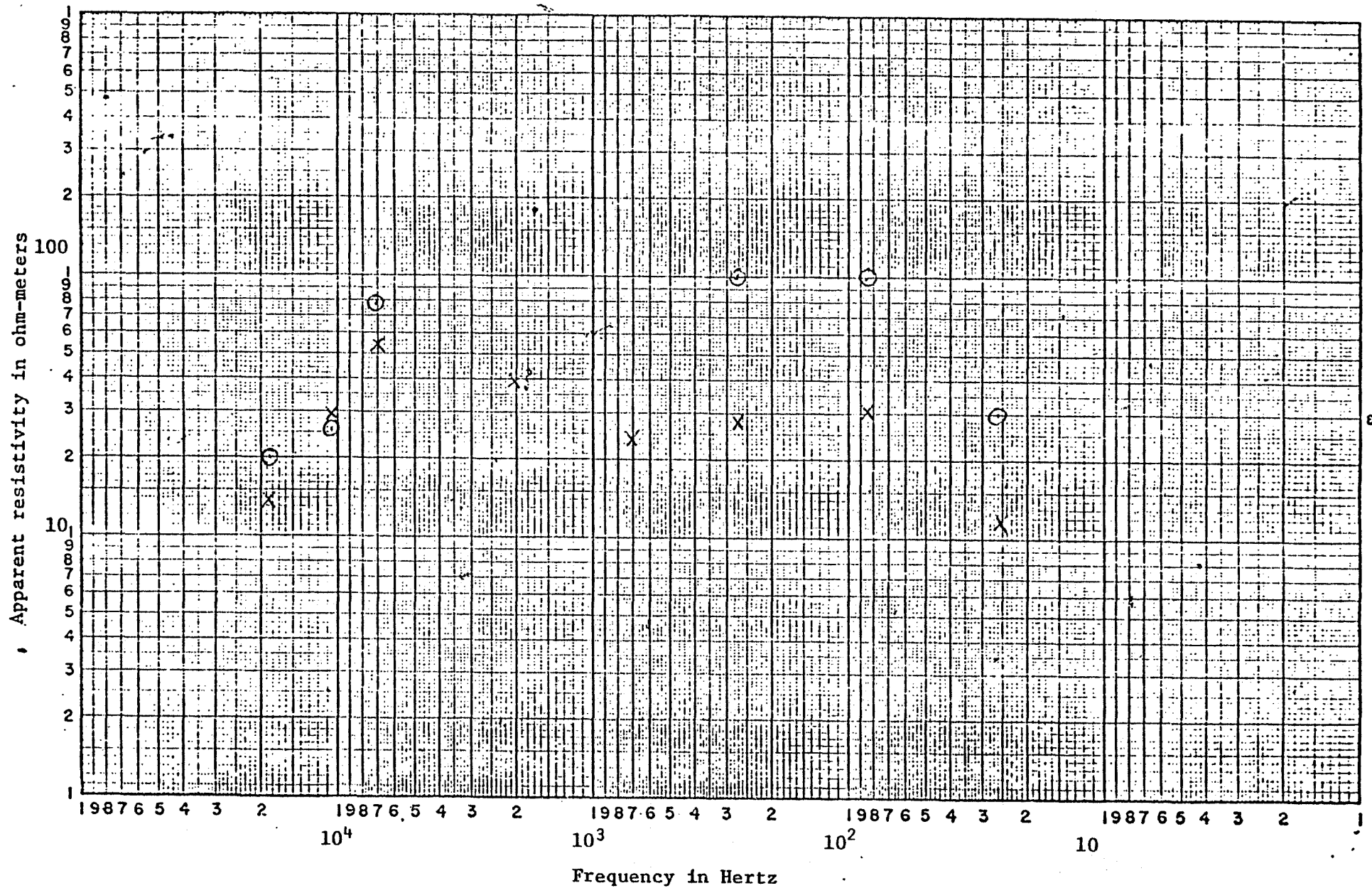
Figure 17. AMT sounding, Long Valley #22. x, electric line west, O electric line south.
