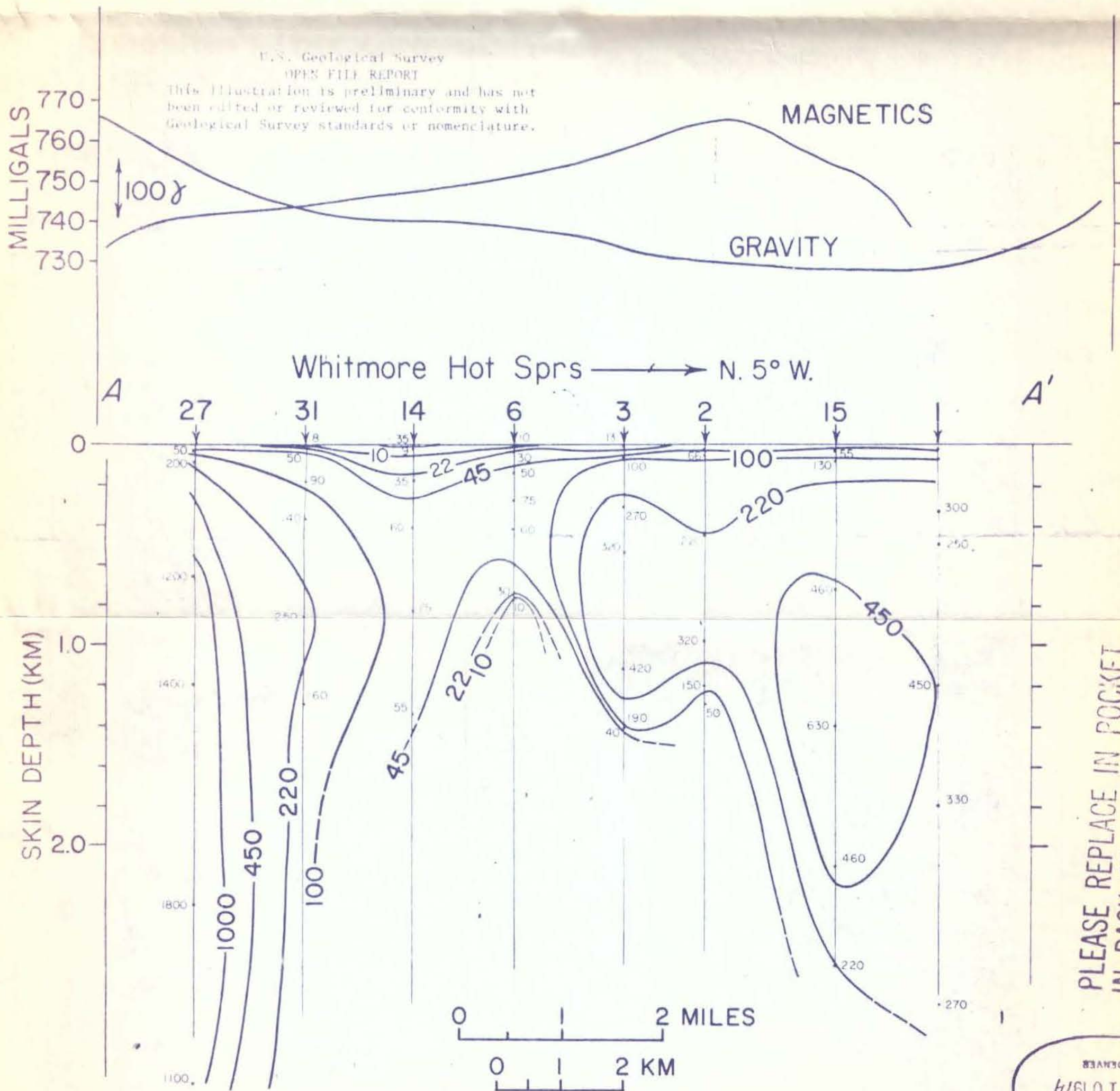
SKIN-DEPTH PSEUDOSECTION ALONG A-A' (ELECTRIC LINE E-W) LONG VALLEY, CALIF.
