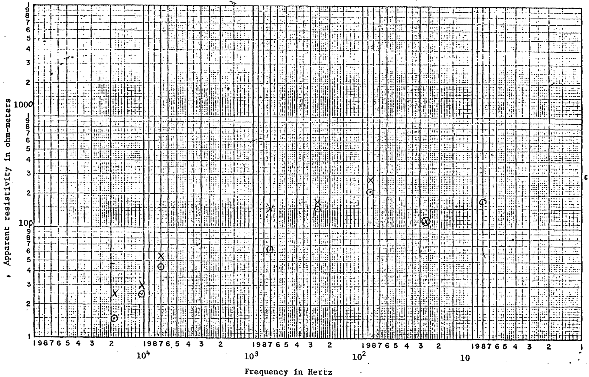
Figure 27. AMT sounding, Long Valley #32. x, electric line east, O electric line south.
