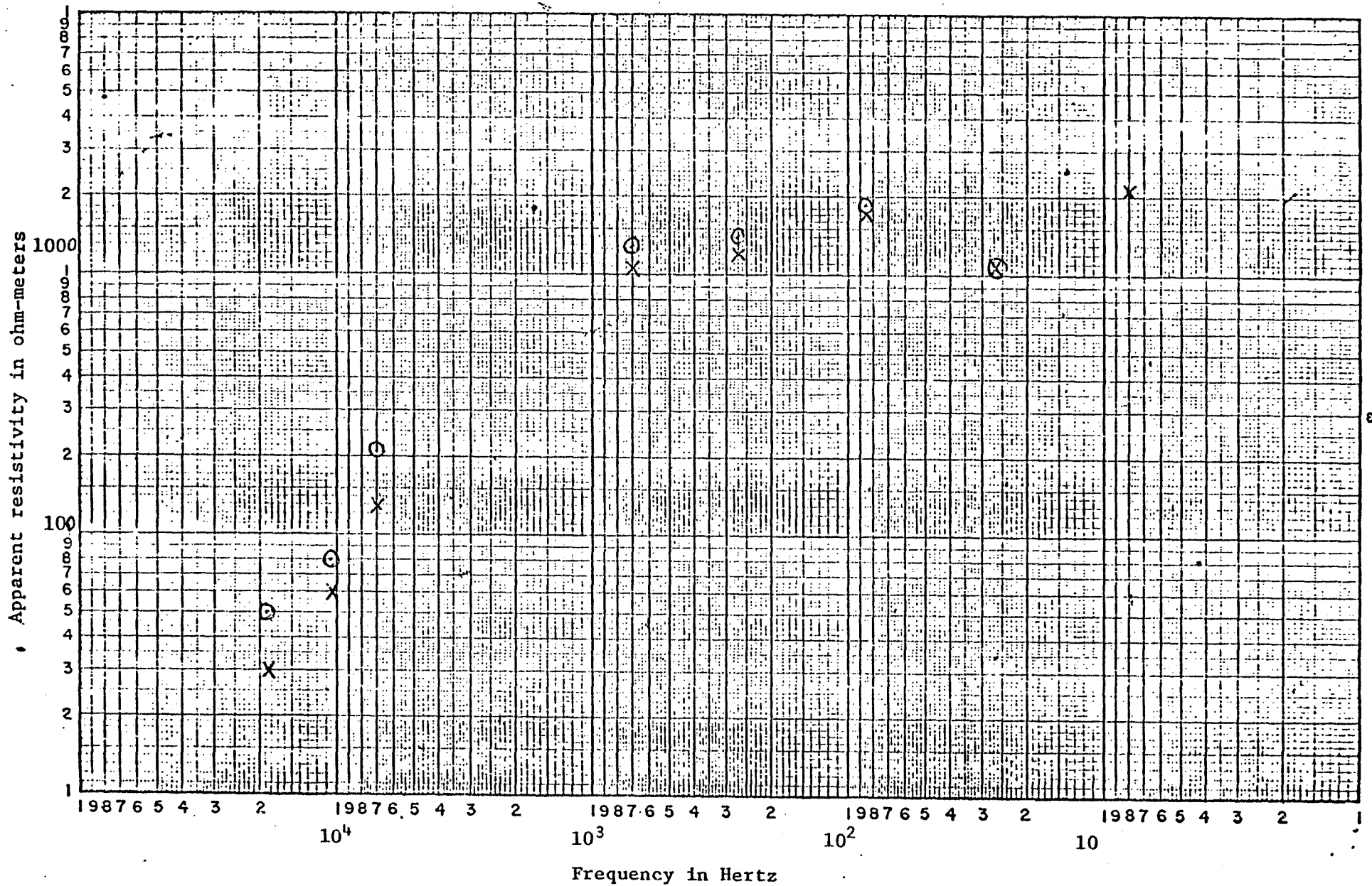
Figure 22. AMT sounding, Long Valley #27, x, electric line west, O electric line south.
