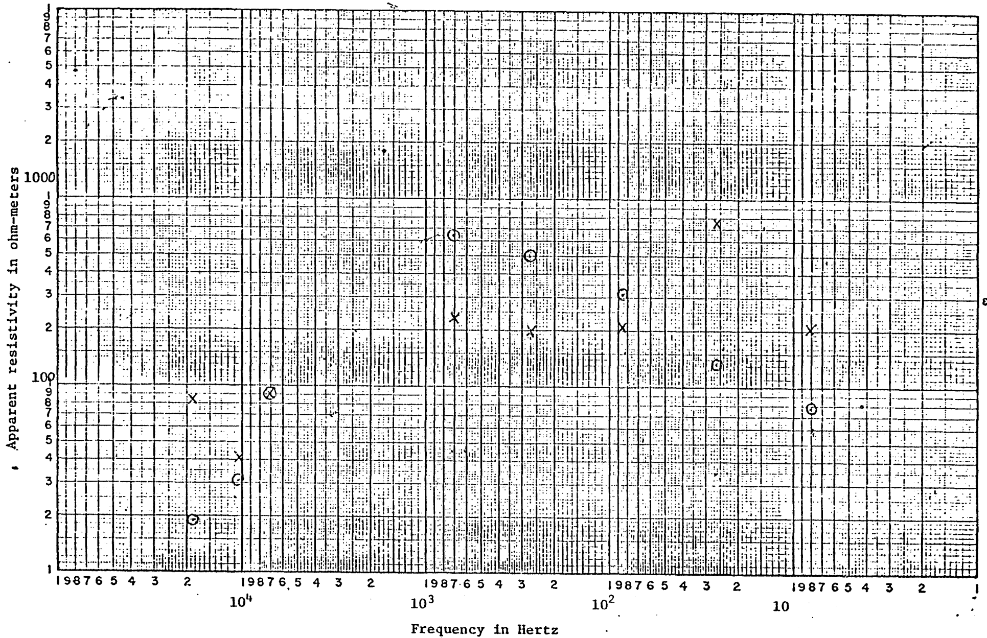
Figure 16. AMT sounding, Long Valley #21. x, electric line west, ⊗ electric line north.
