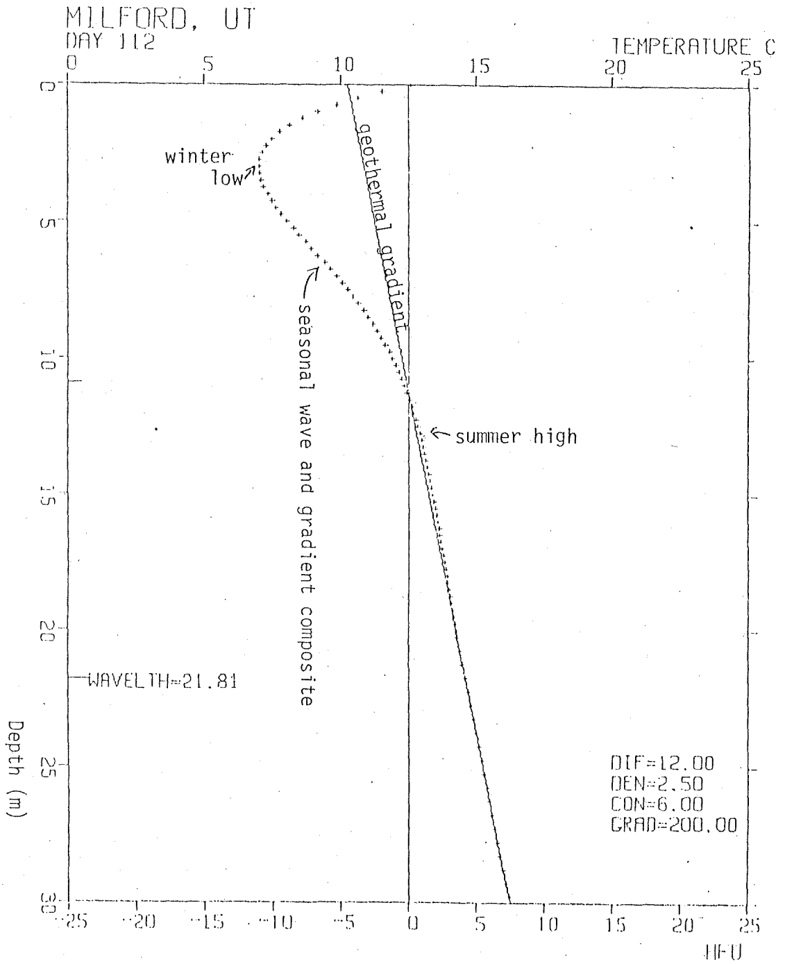
Figure 1. Thermal log (+) consisting of the seasonal wave superimposed on a geothermal gradient of 200^{\circ}\text{C}/\text{km} , in a medium having a thermal conductivity of 6 units. The diurnal wave is not shown; but would be confined to the upper 1 meter of the log.
