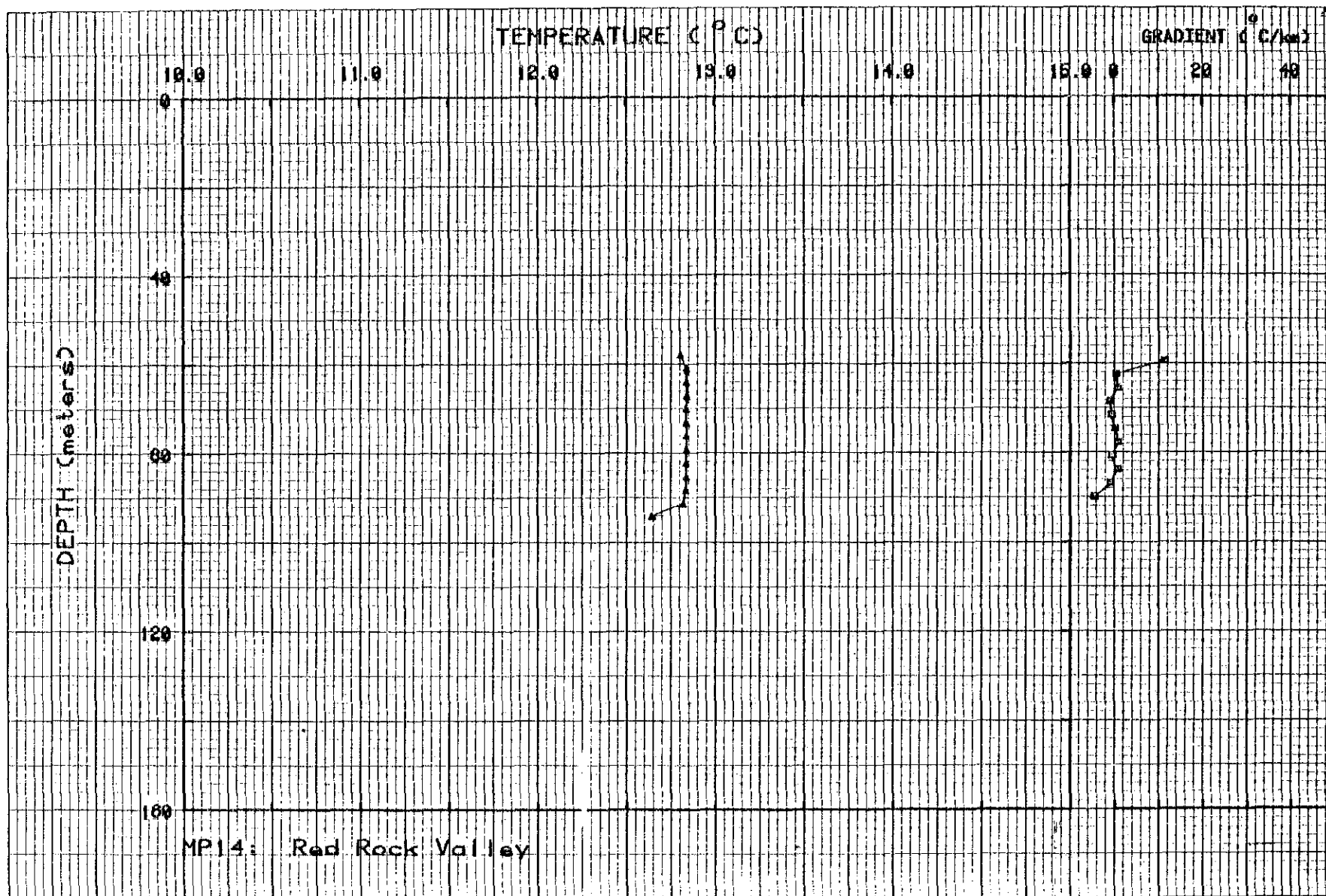
Figure II-14. Temperature and gradient profiles for MP14.
