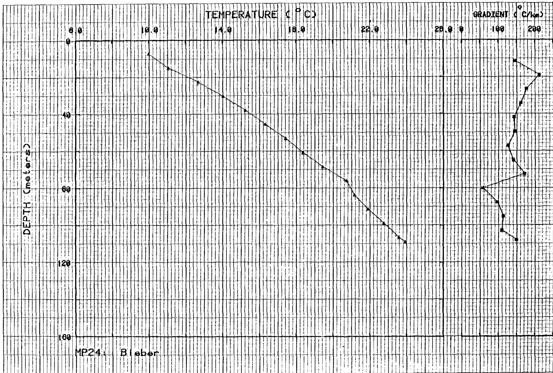
Figure II-24. Temperature and gradient profiles for MP24.
