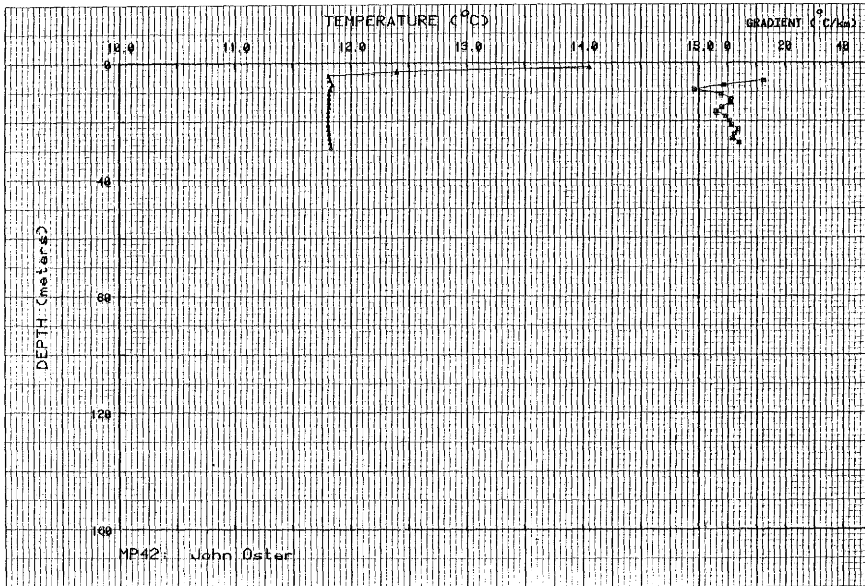
Figure II-41. Temperature and gradient profiles for MP42.
