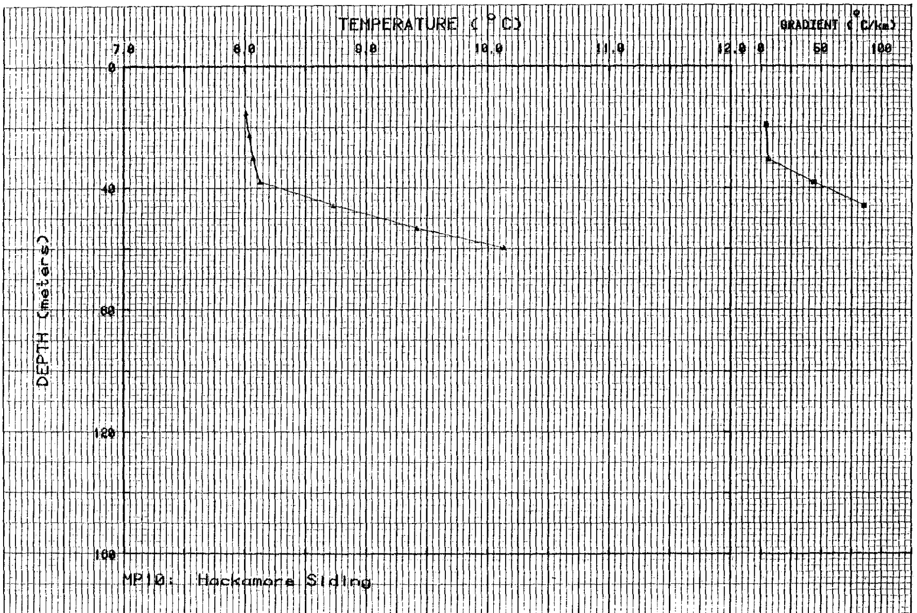
Figure II-10. Temperature and gradient profiles for MP10.
