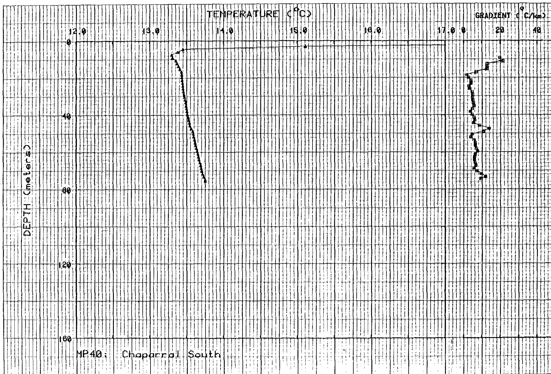
Figure II-39. Temperature and gradient profiles for MP40.
