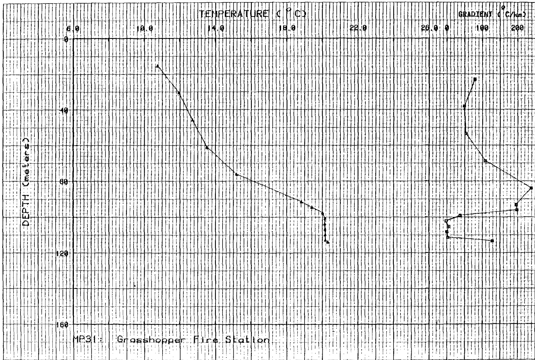
Figure II-31. Temperature and gradient profile for MP31.
