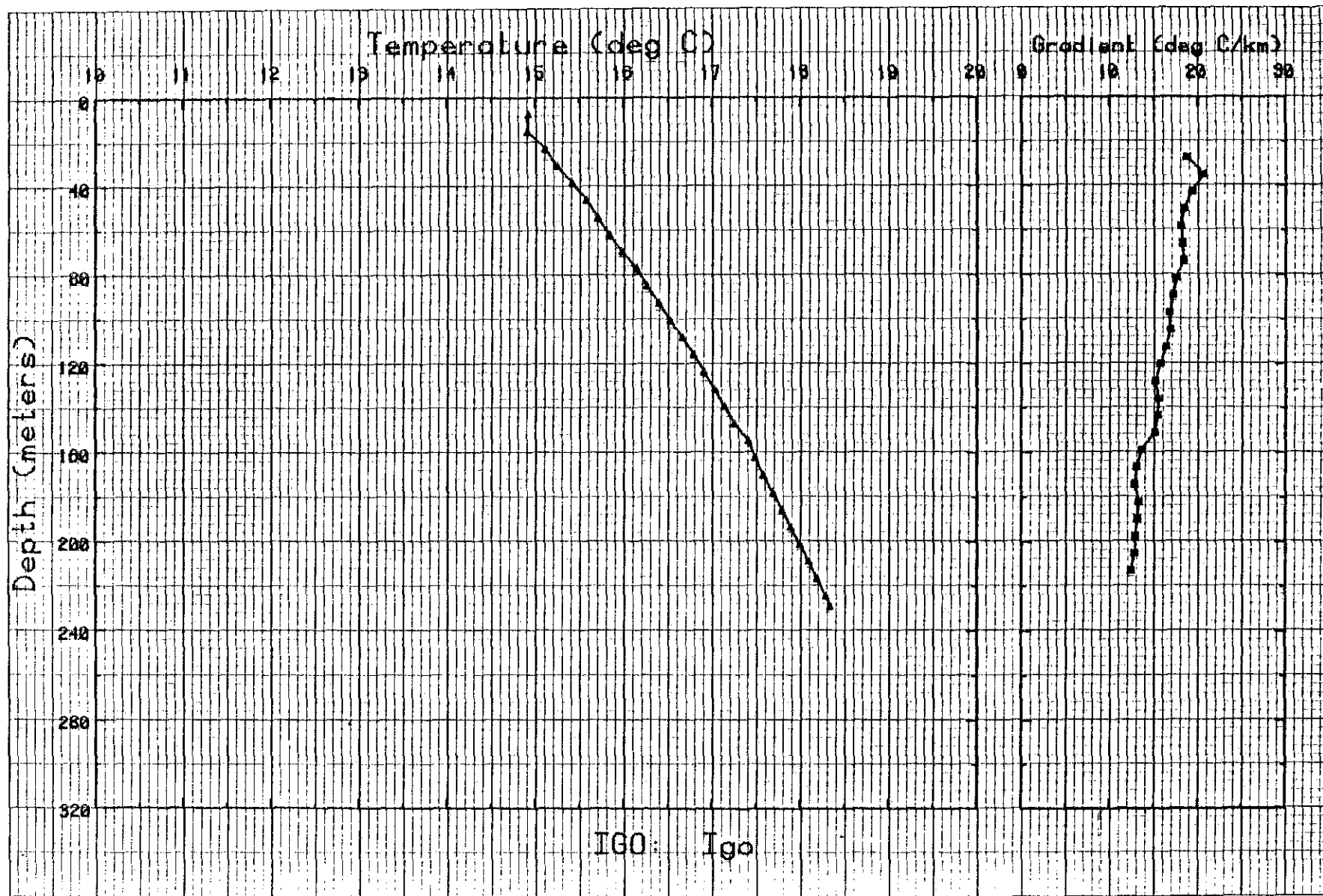
Figure I-5. Temperature and gradient profile for IGO.
