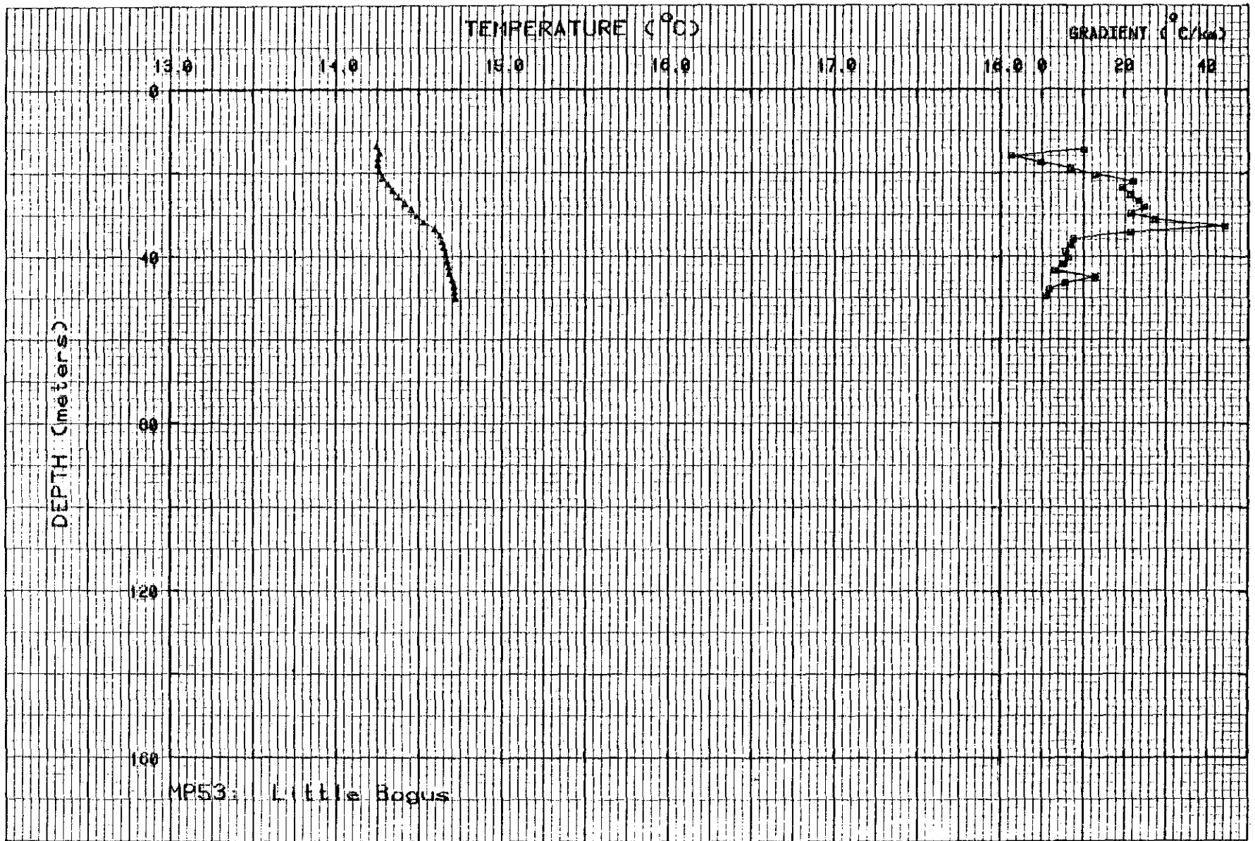
Figure II-52. Temperature and gradient profiles for MP53.
