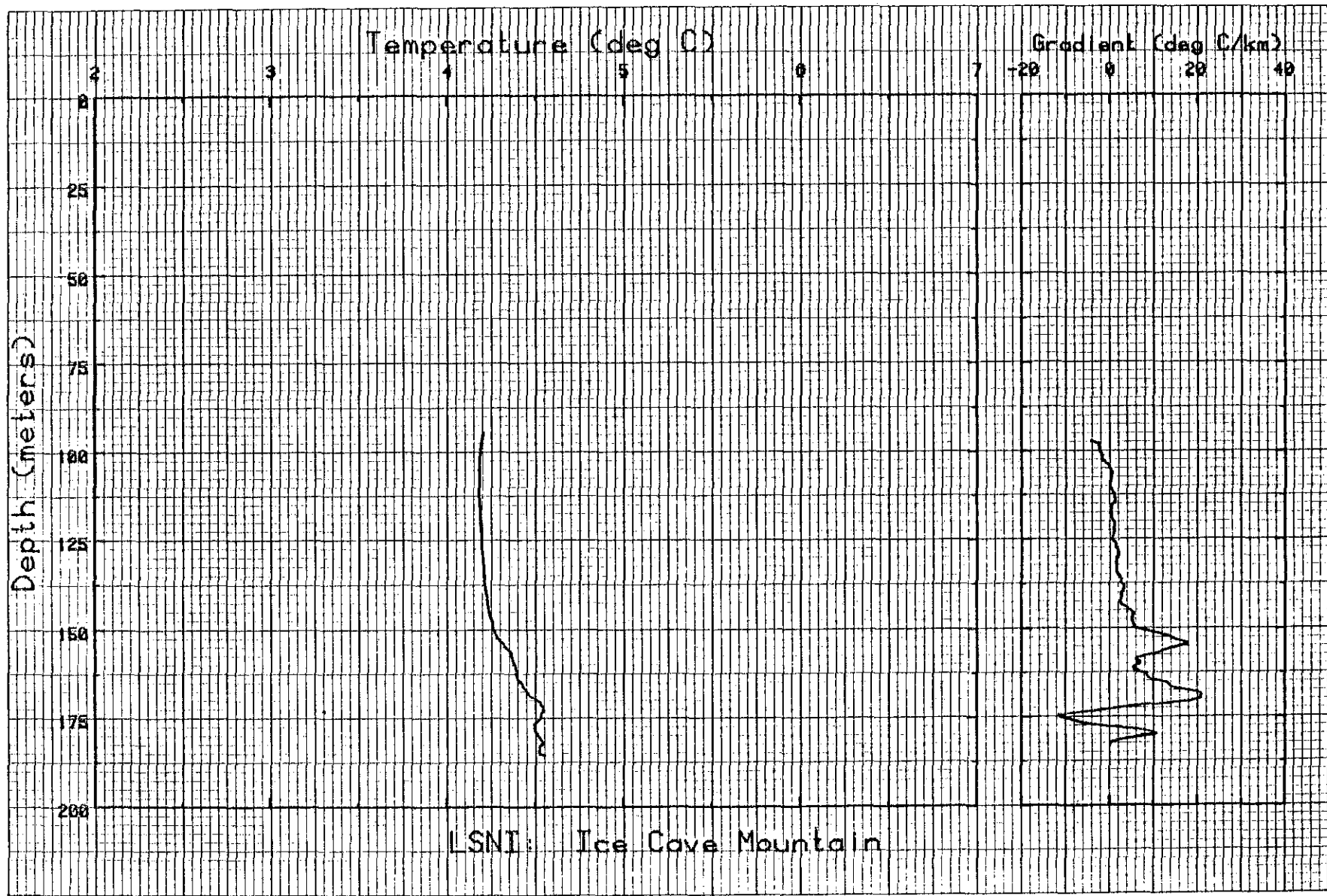
Figure I-13. Temperature and gradient profiles for LSNI.
