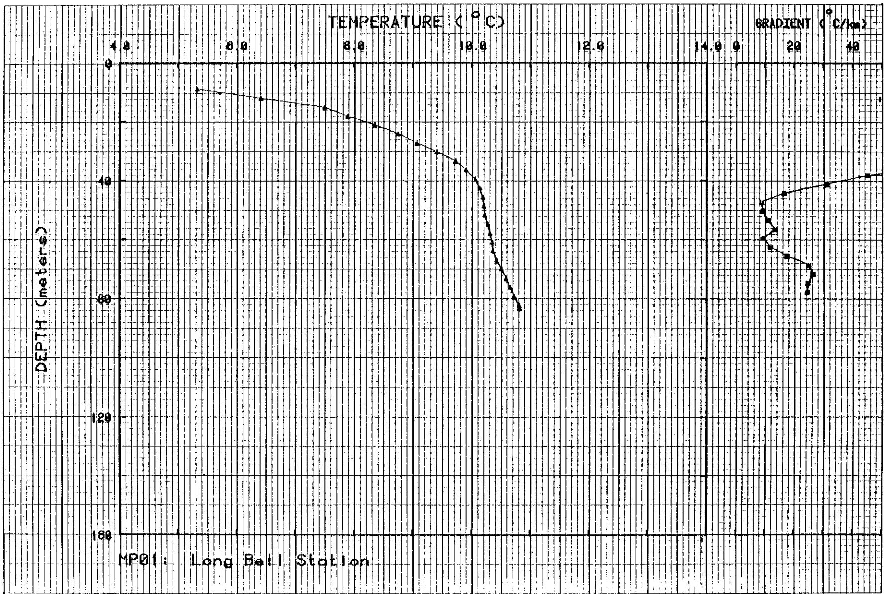
Figure II-1. Temperature and gradient profiles for MP01.
