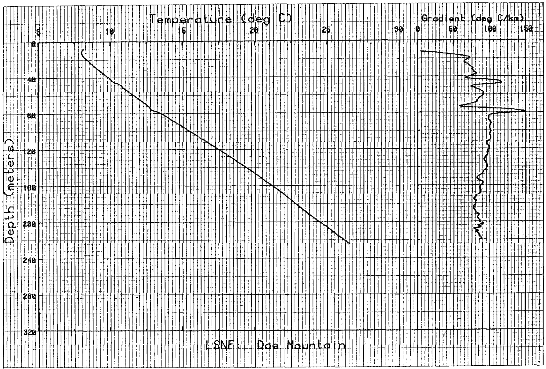
Figure I-10. Temperature and gradient profiles for LSNF.
