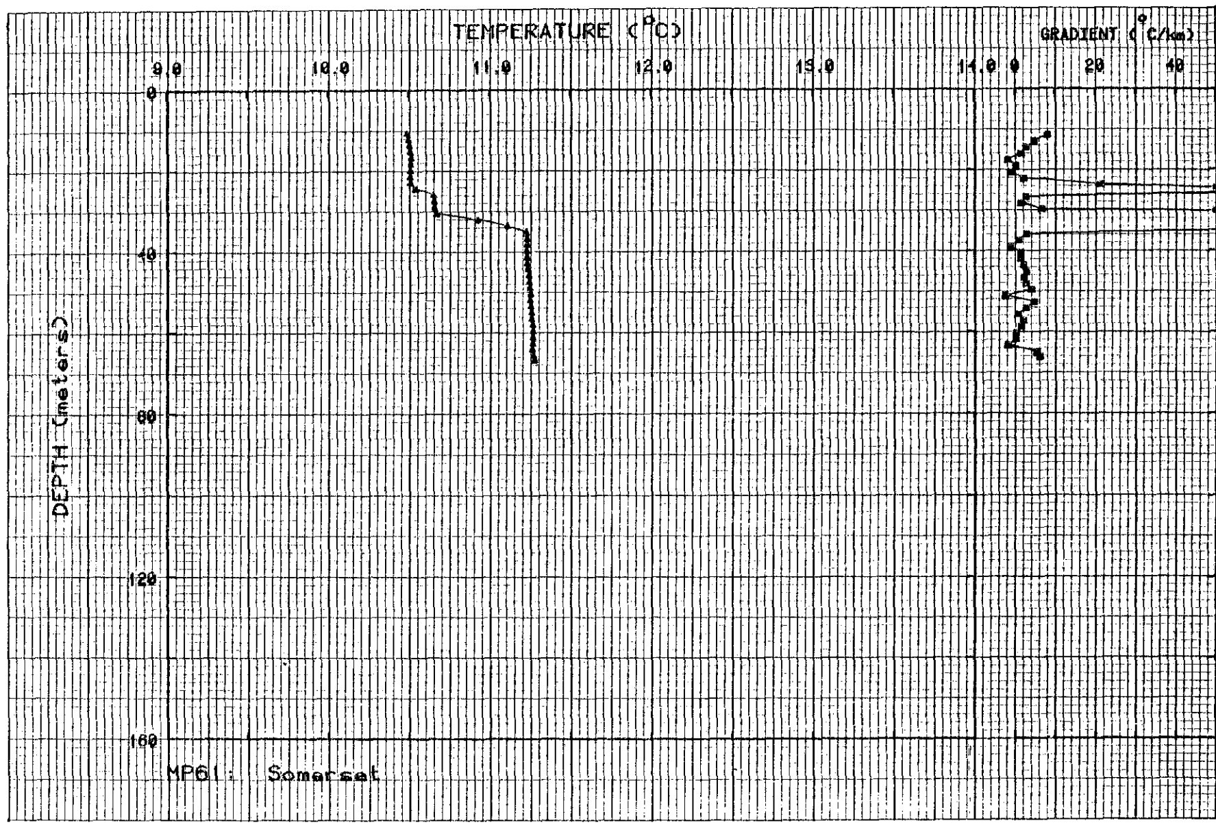
Figure II-60. Temperature and gradient profiles for MP61.
