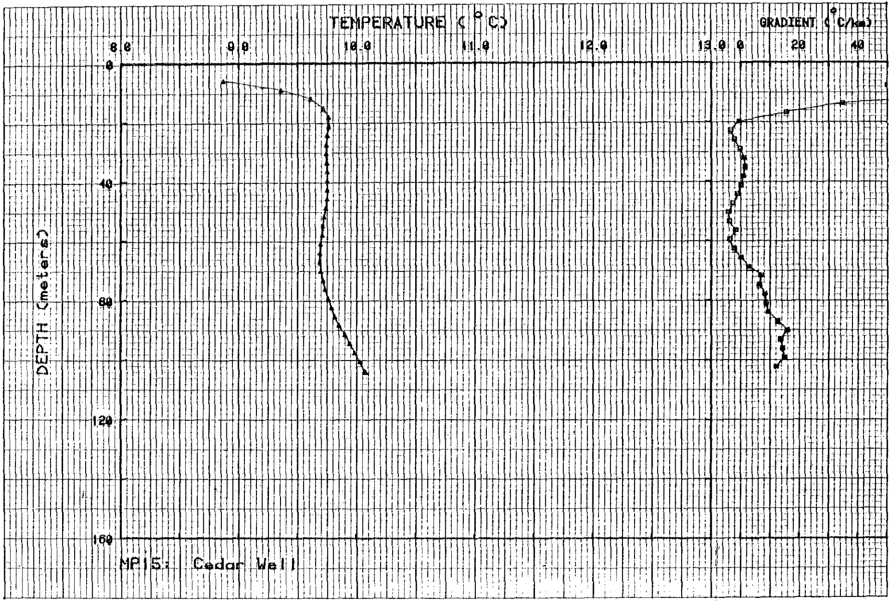
Figure II-15. Temperature and gradient profiles for MP15.
