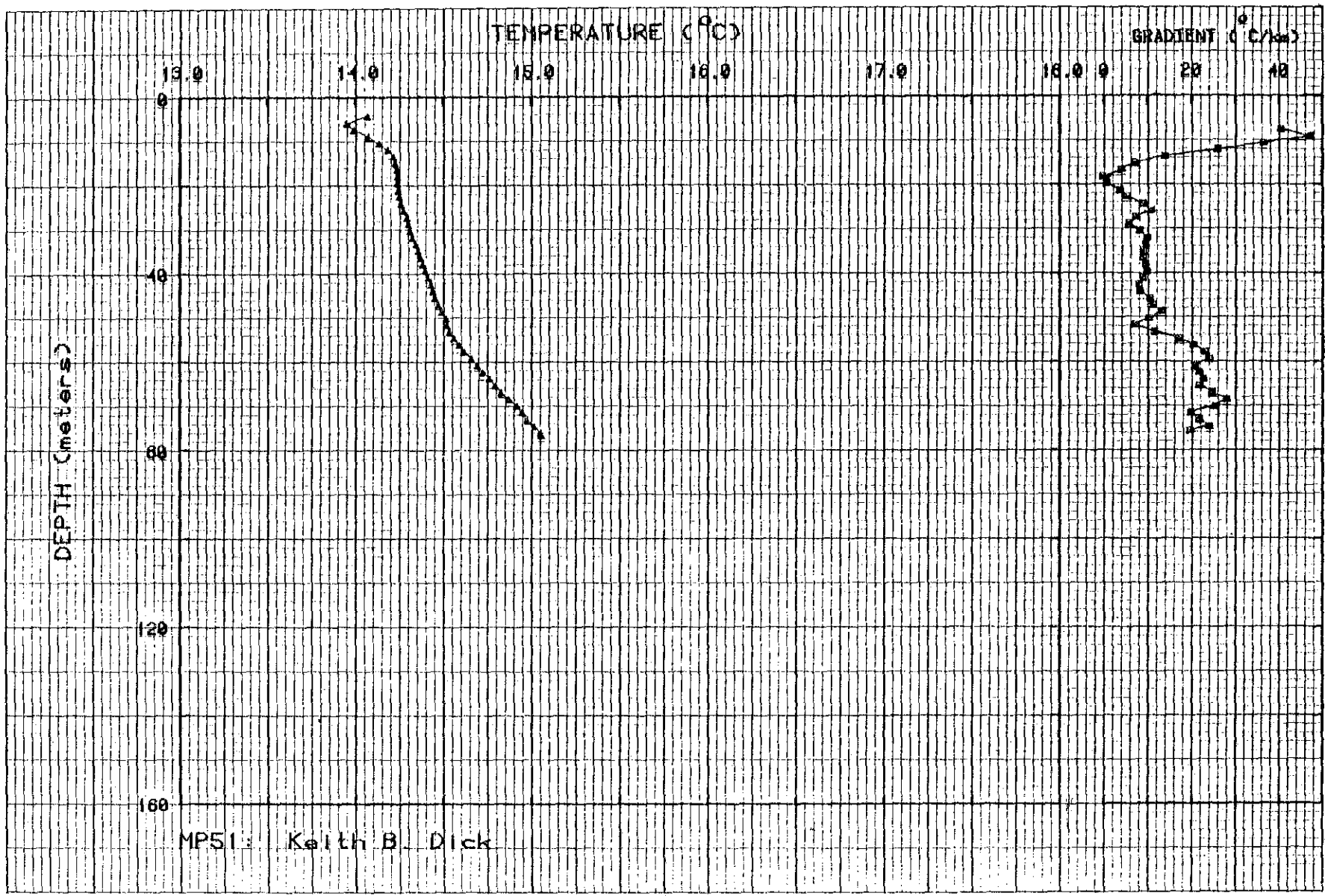
Figure II-50. Temperature and gradient profiles for MP51.
