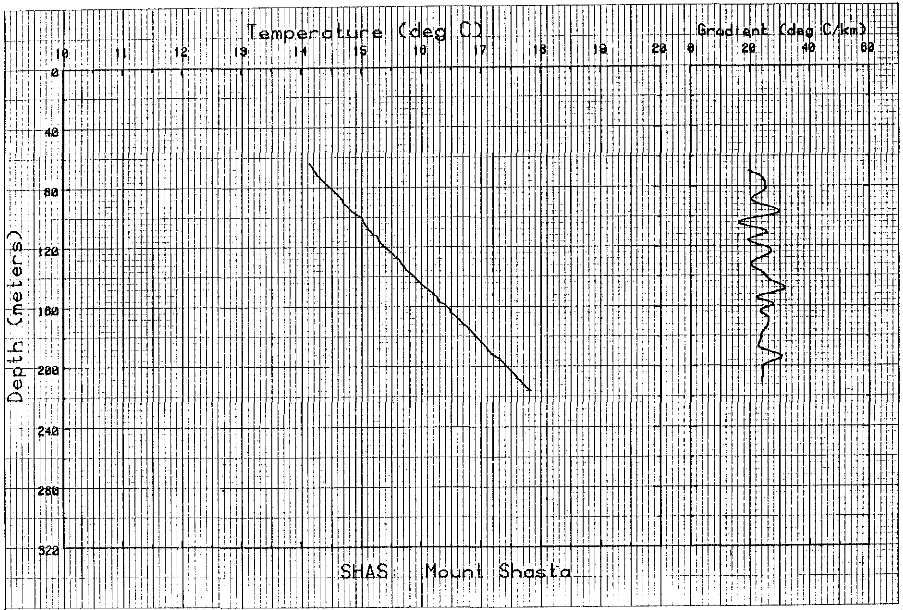
Figure I-18. Temperature and gradient profiles for SHAS.
