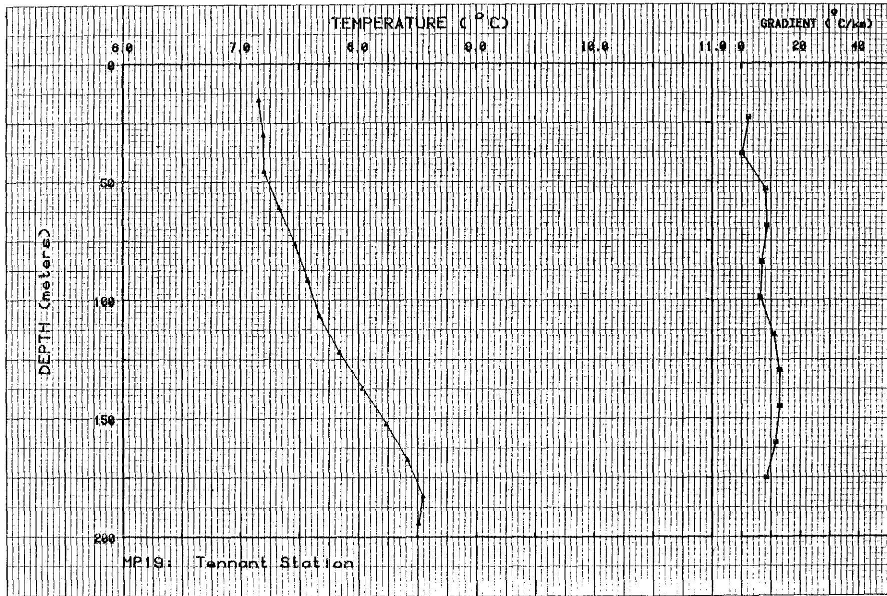
Figure II-19. Temperature and gradient profiles for MP19.
