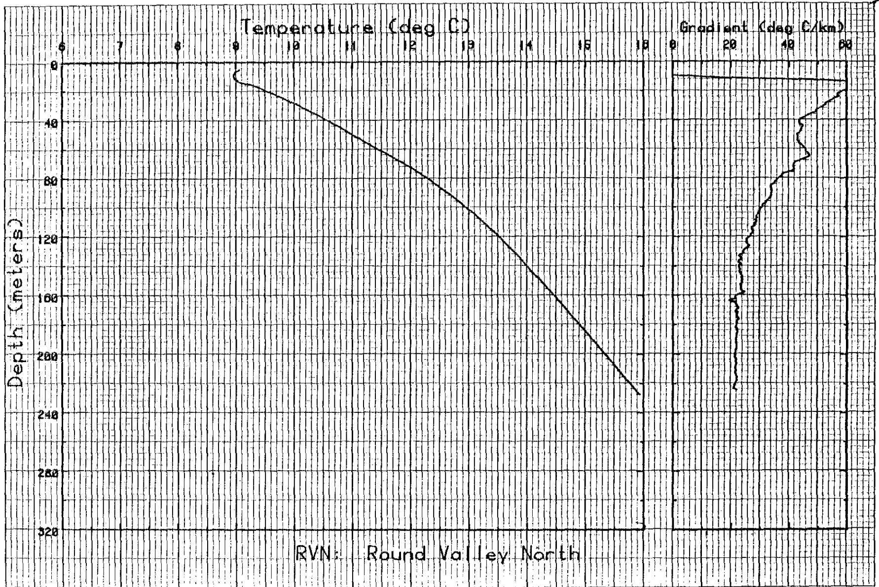
Figure I-17. Temperature and gradient profiles for RVN.
