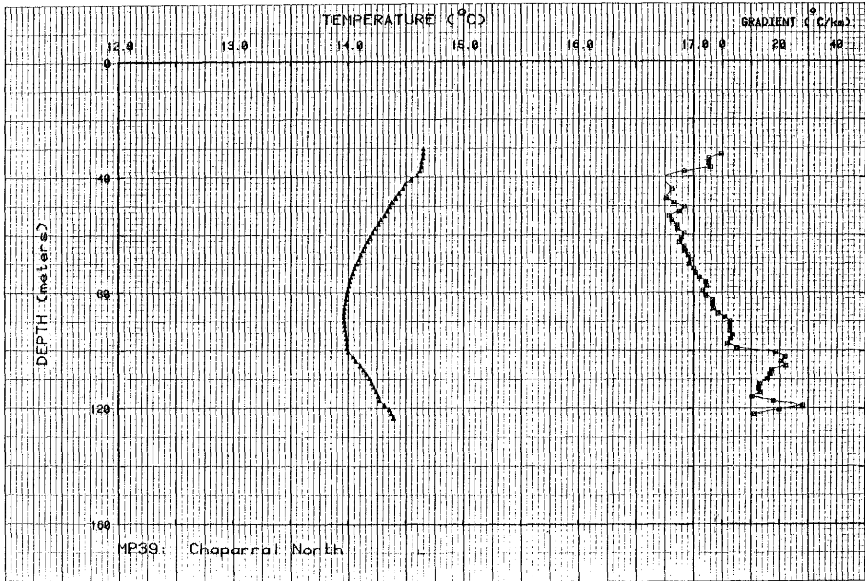
Figure II-38. Temperature and gradient profiles for MP39.
