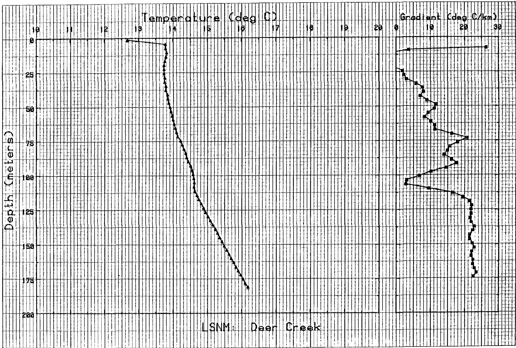
Figure I-15. Temperature and gradient profiles for LSM.
