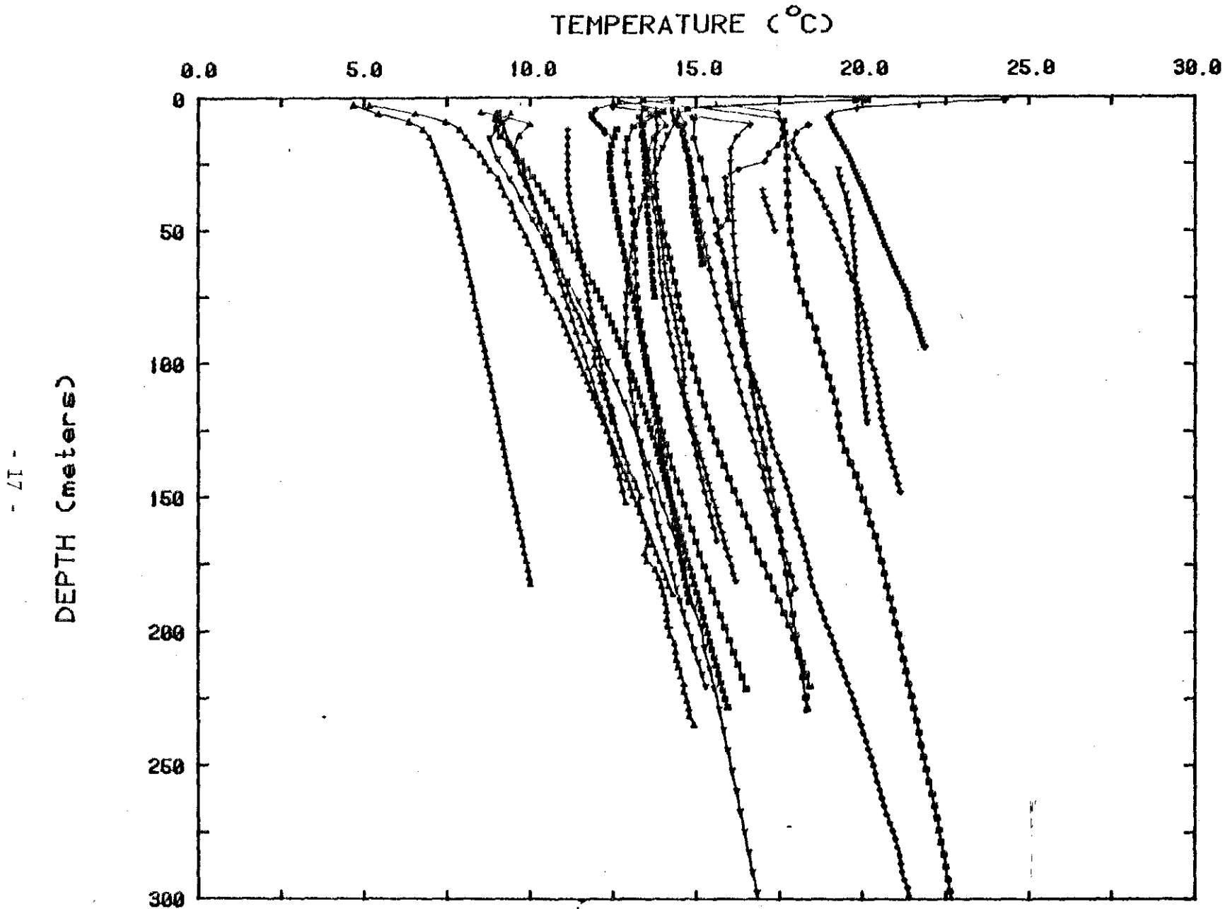
Figure 3. Temperature-depth profiles for the Coastal Provinces, Klamath Mountains, and Sierra Nevada
