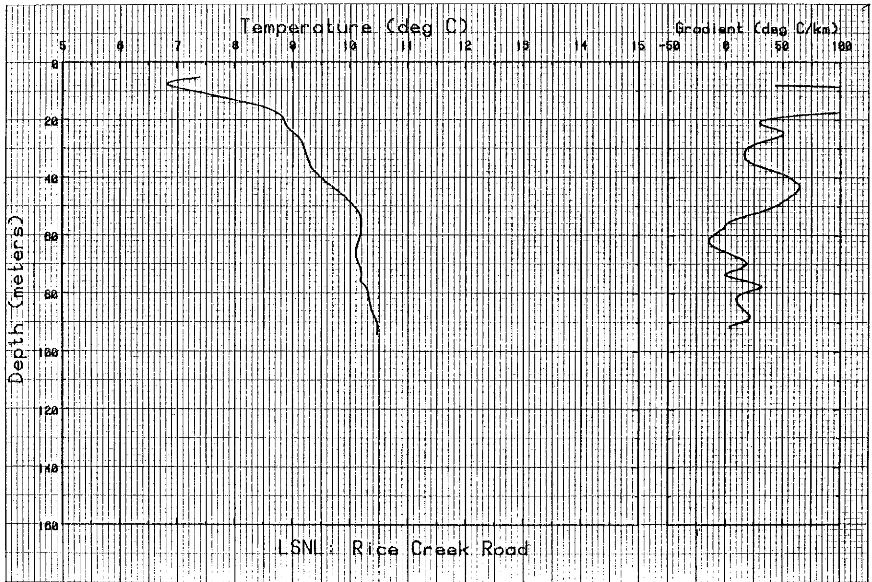
Figure I-14. Temperature and gradient profiles for LSNL.
