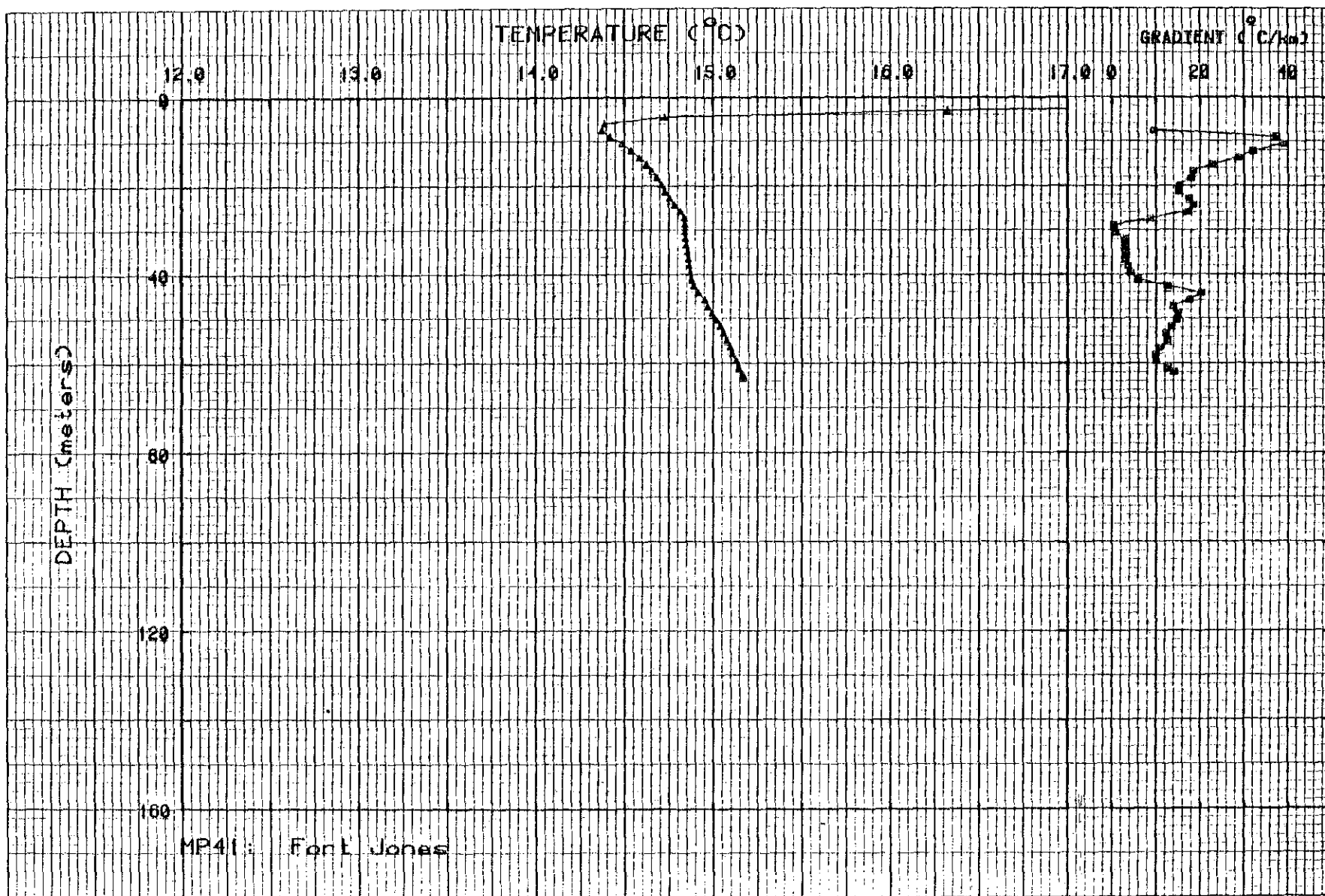
Figure II-40. Temperature and gradient profiles for MP41.
