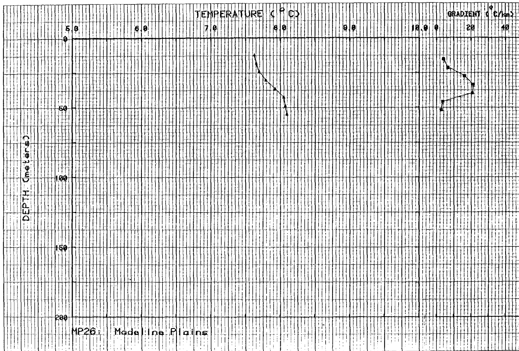
Figure II-26. Temperature and gradient profiles for MP26.
