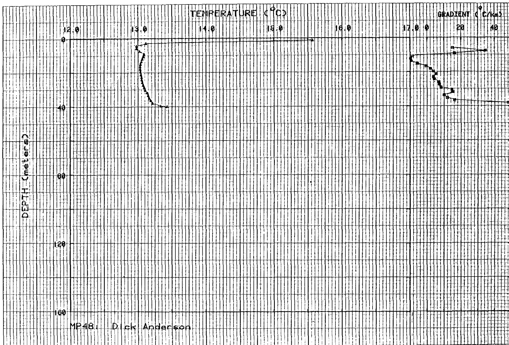
Figure II-47. Temperature and gradient profiles for MP48.
