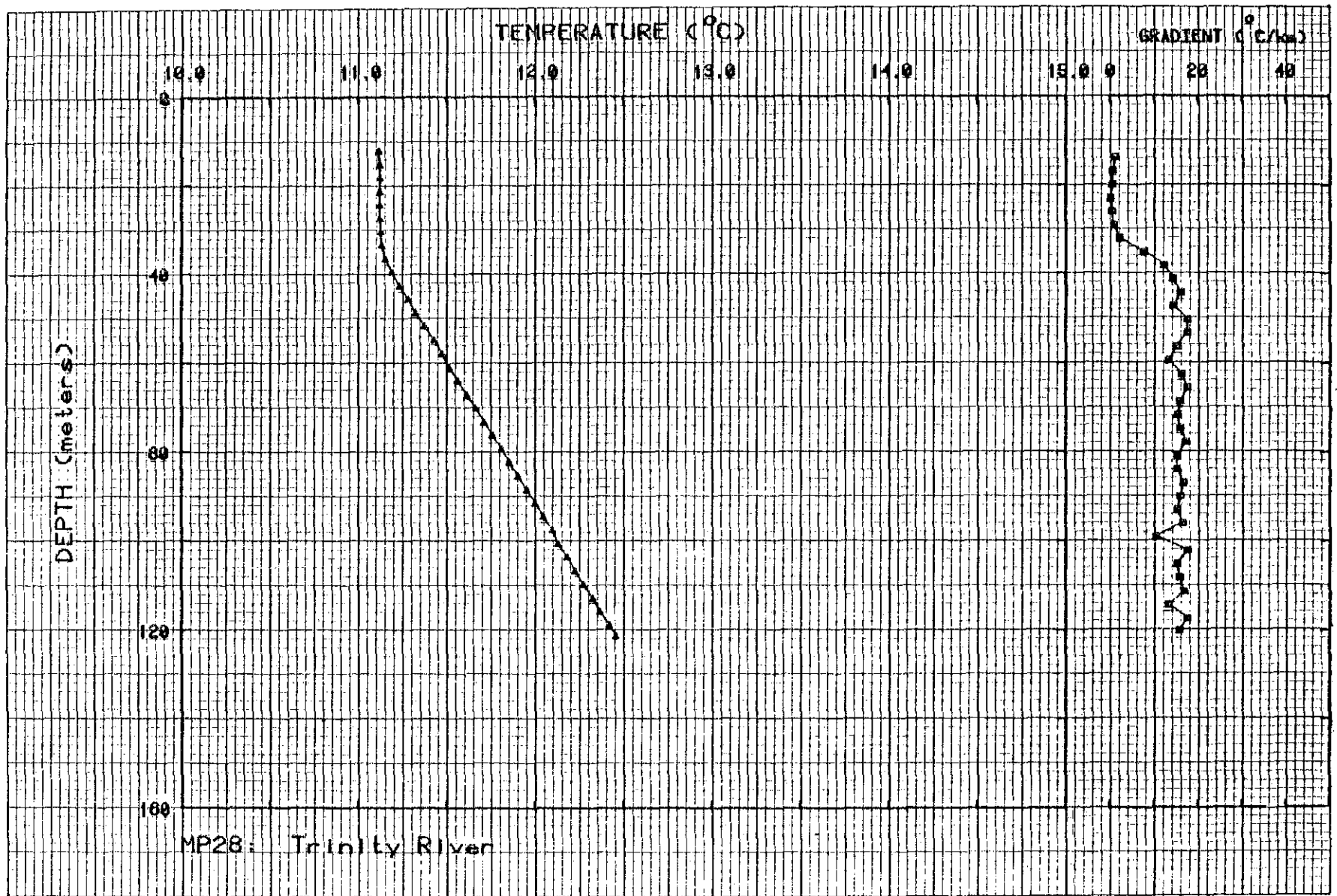
Figure II-28. Temperature and gradient profiles for MP28.
