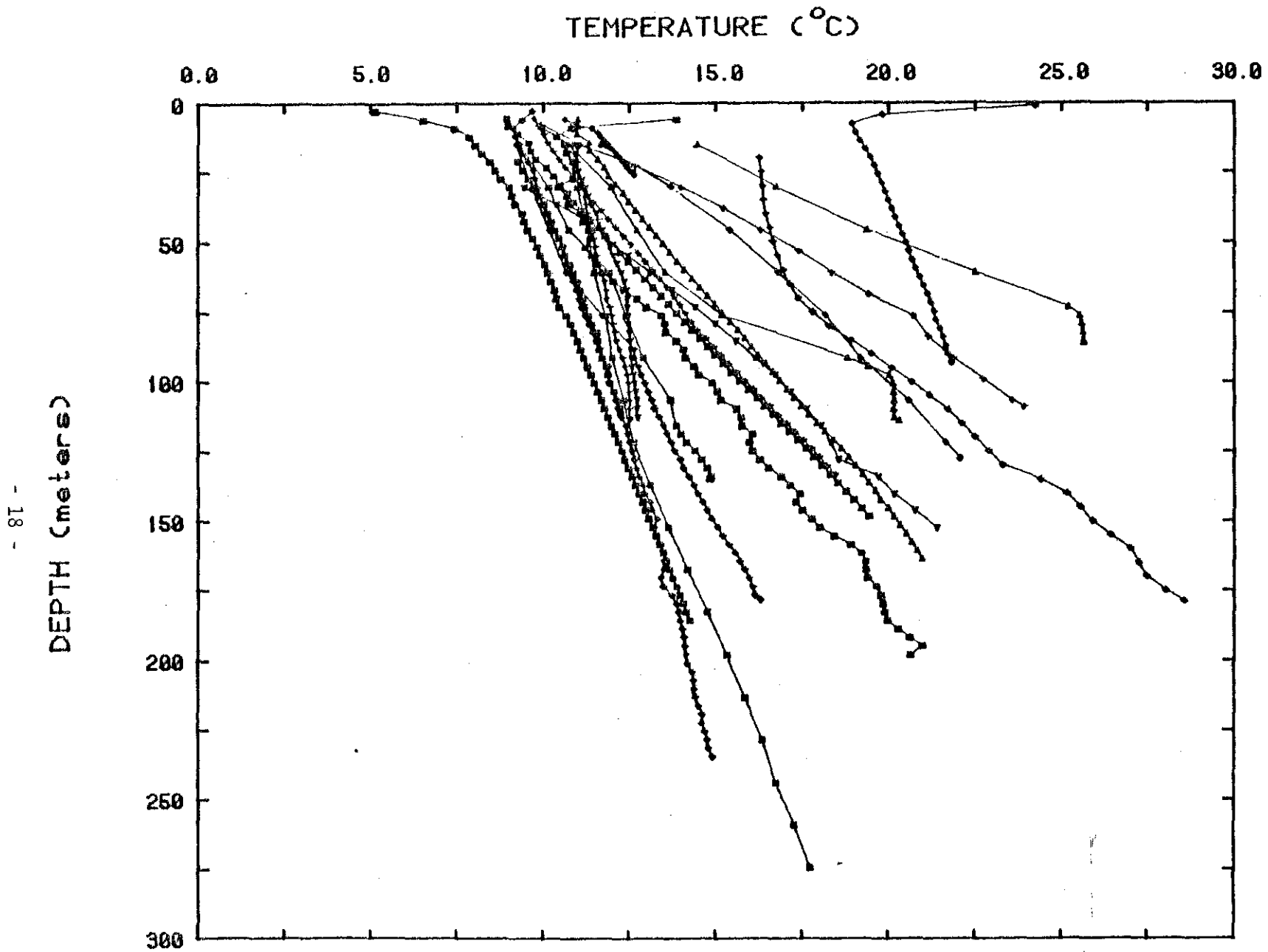
Figure 4. Temperature-depth profiles for the Basin and Range.
