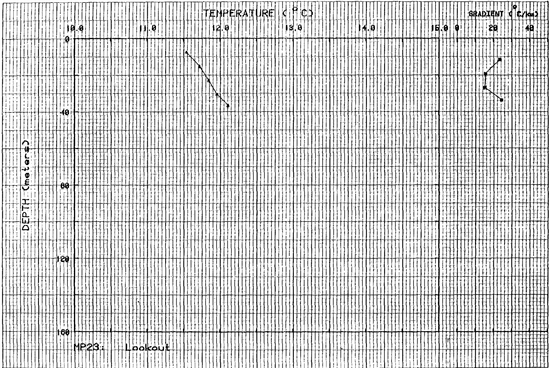
Figure II-23. Temperature and gradient profiles for MP23.
