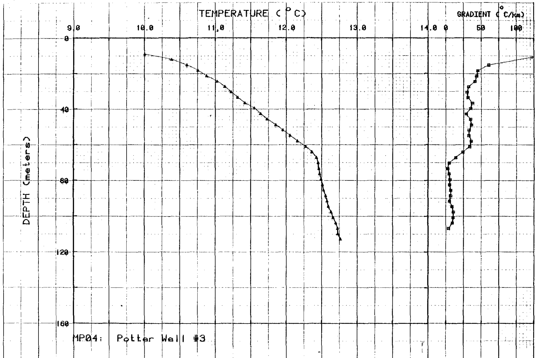
Figure II-4. Temperature and gradient profiles for MP04.
