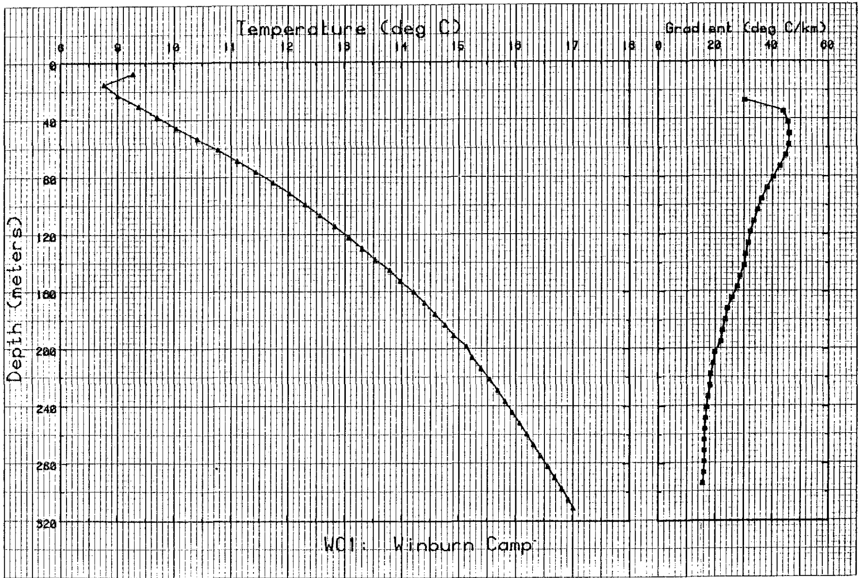
Figure I-19. Temperature and gradient profiles for W01.
