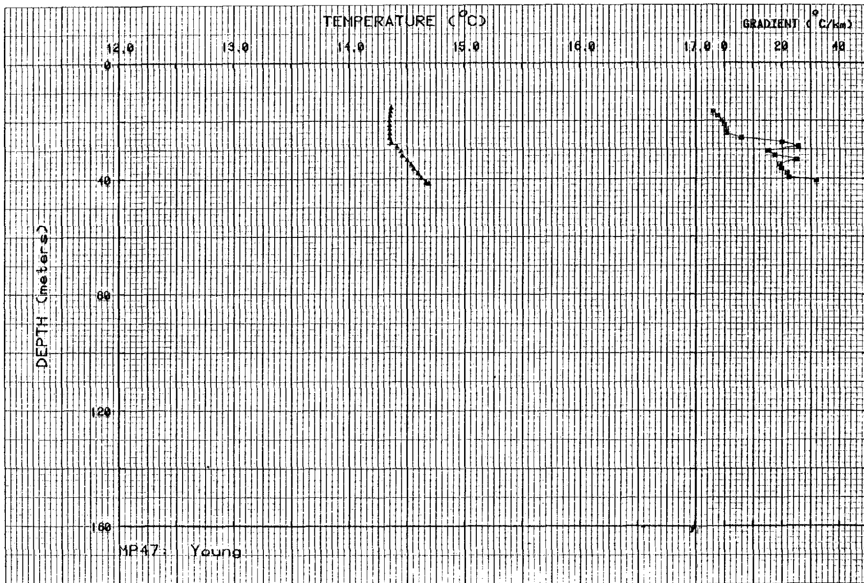
Figure II-46. Temperature and gradient profiles for MP47.
