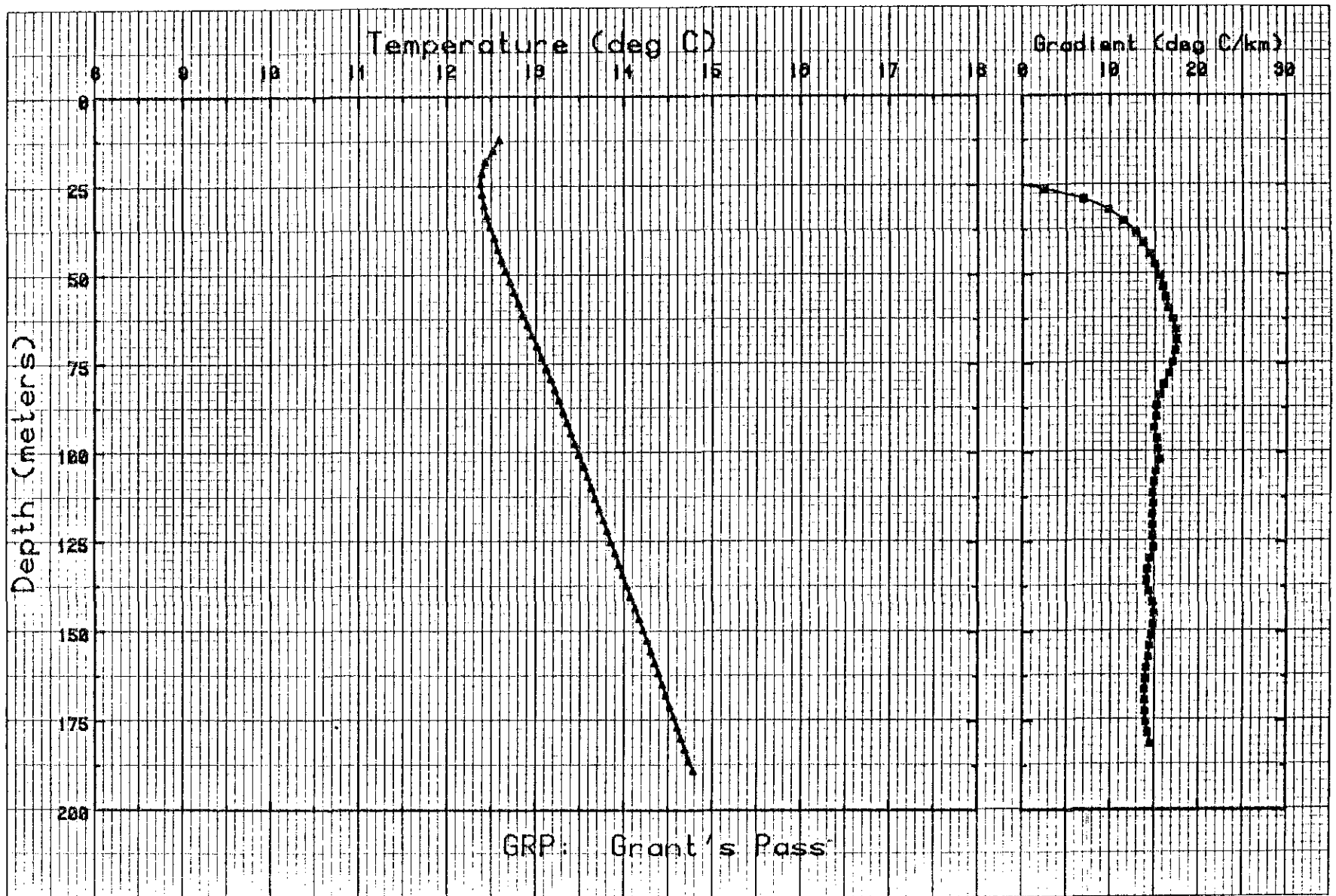
Figure I-3. Temperature and gradient profiles for GRP.
