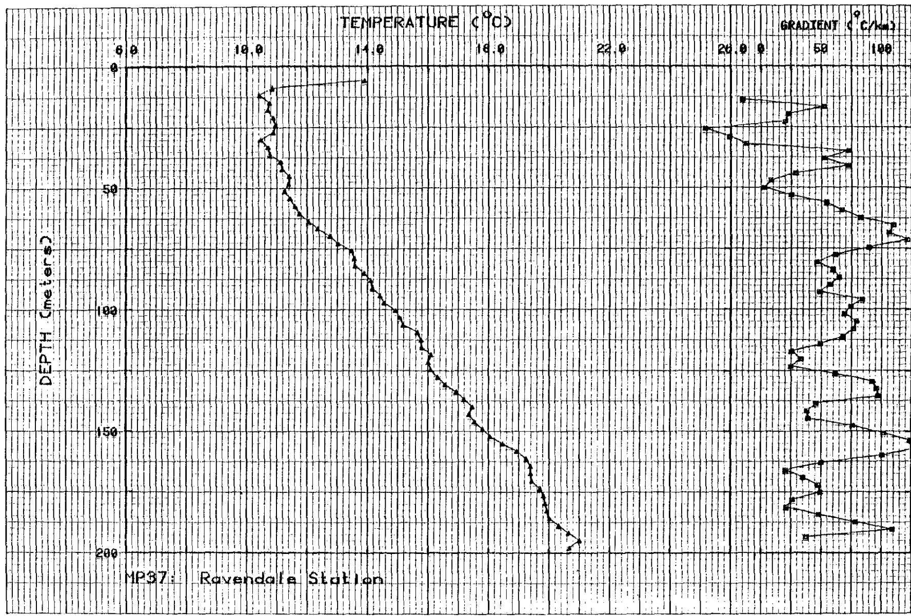
Figure II-36. Temperature and gradient profiles for MP37.
