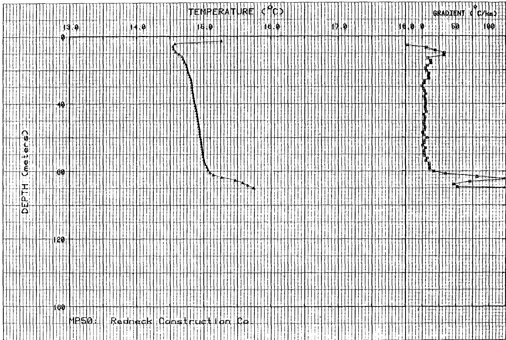
Figure II-49. Temperature and gradient profiles for MP50.
