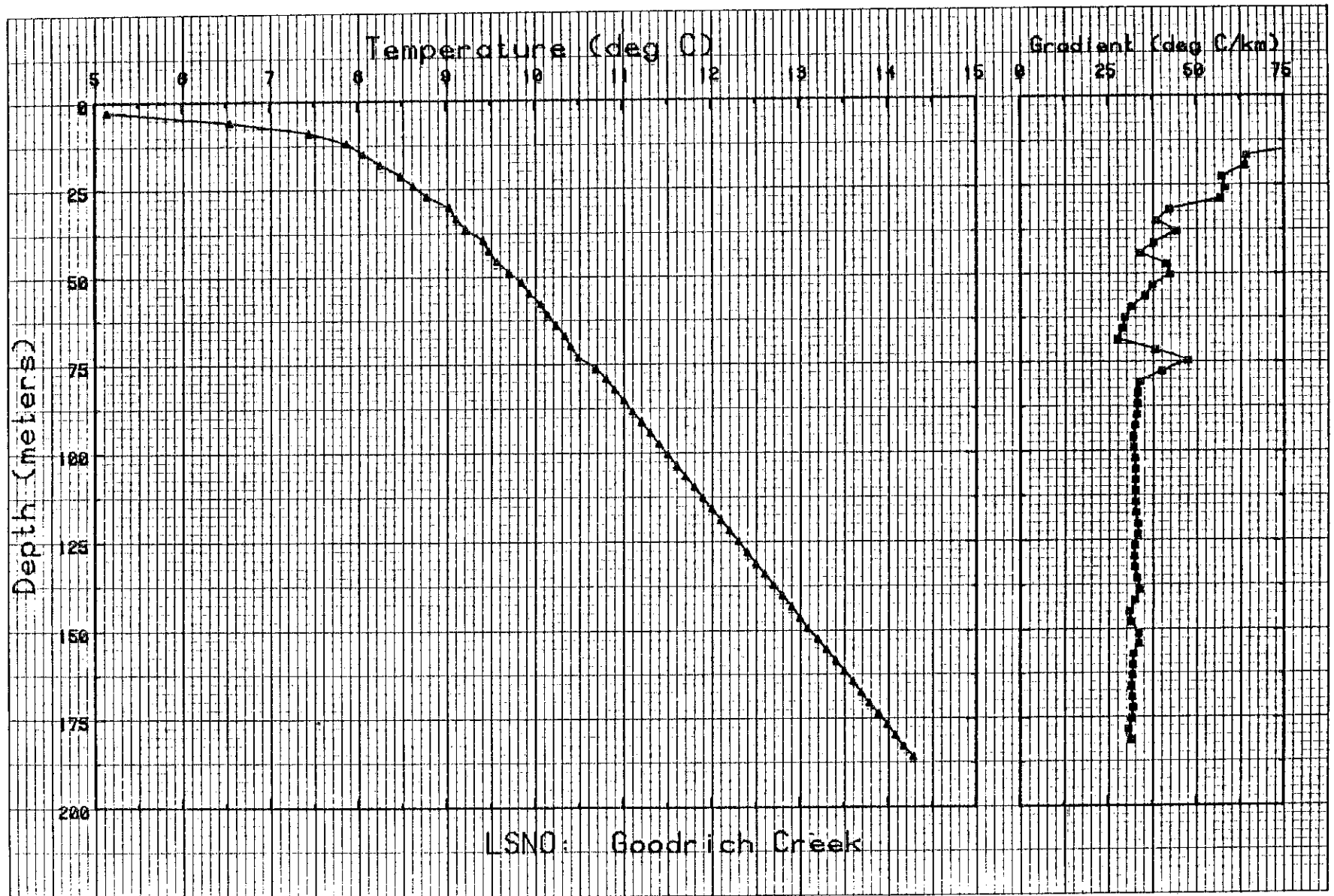
Figure I-16. Temperature and gradient profiles for LSNO.
