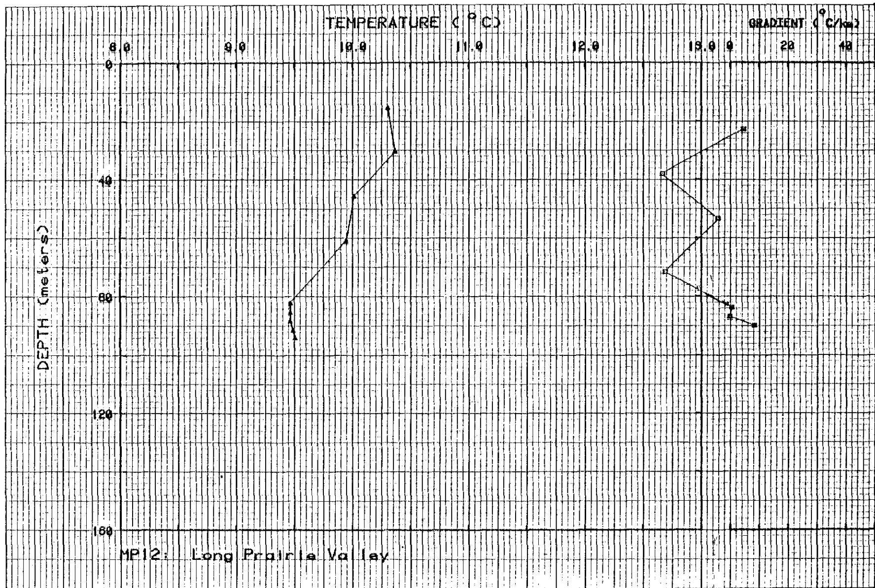
Figure II-12. Temperature and gradient profiles for MP12.
