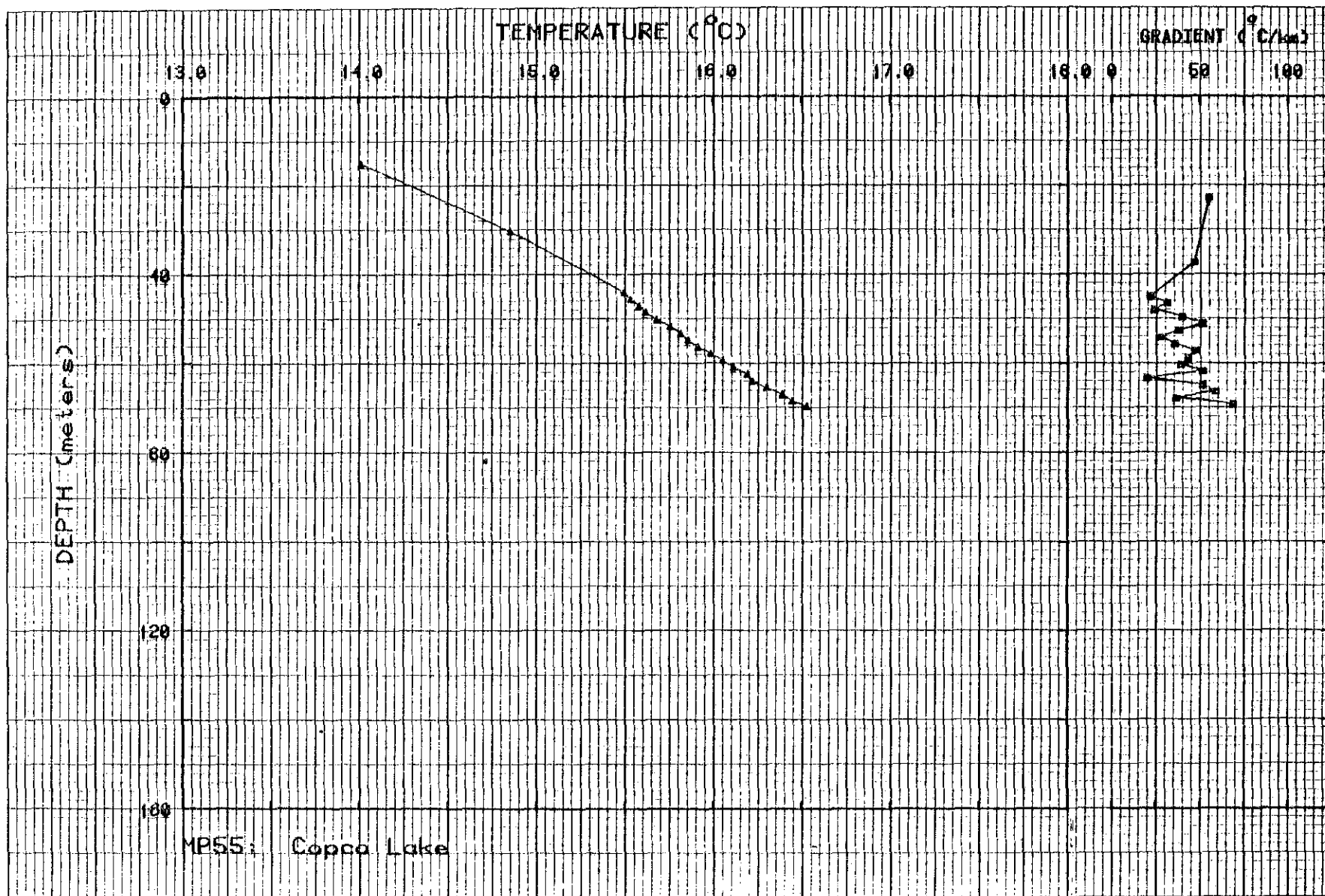
Figure II-54. Temperature and gradient profiles for MP55.
