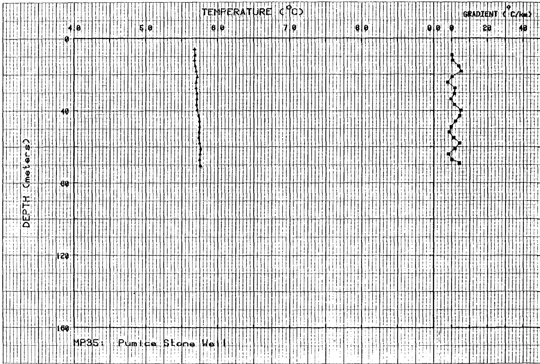
Figure II-35. Temperature and gradient profiles for MP35.
