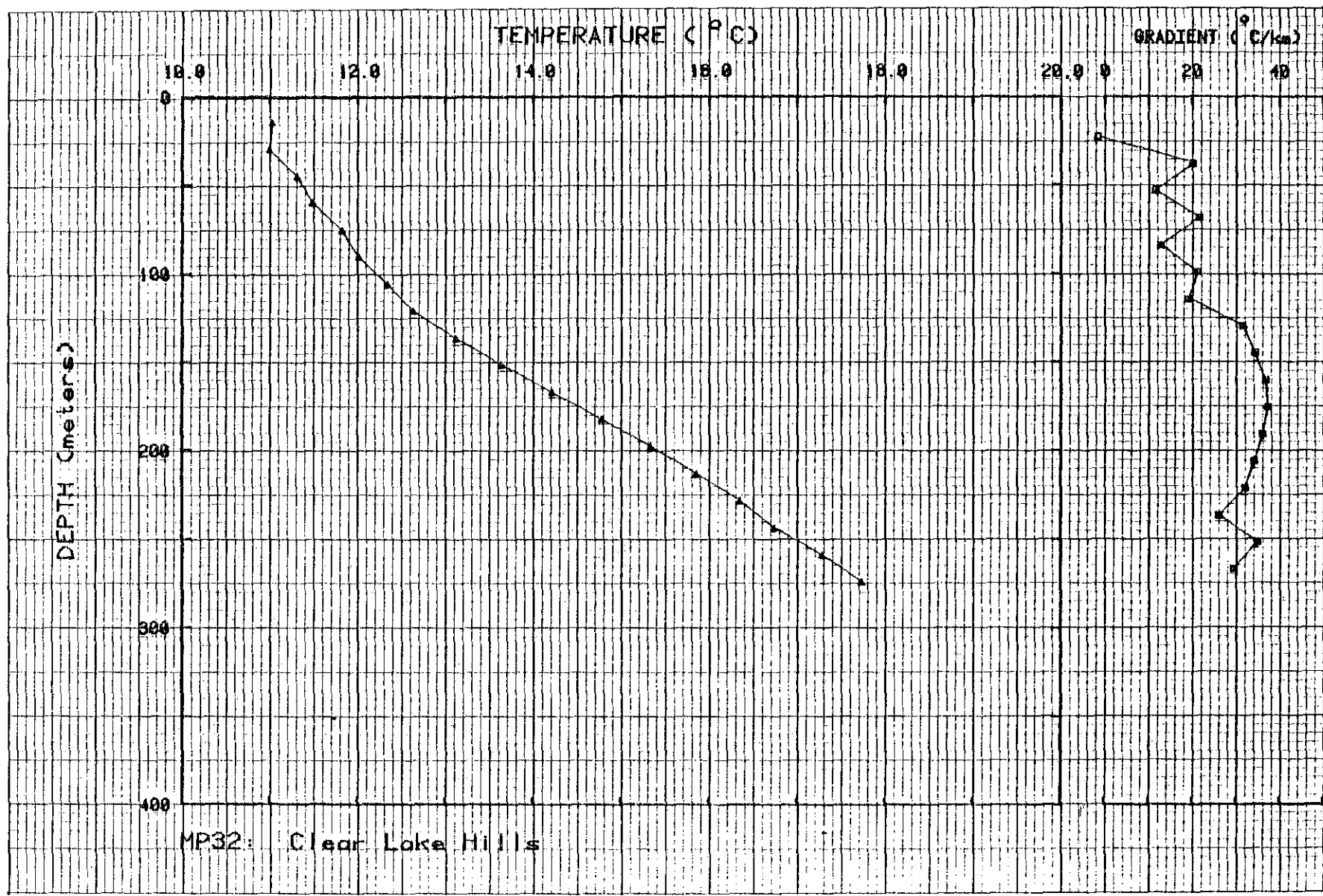
Figure II-32. Temperature and gradient profiles for MP32.
