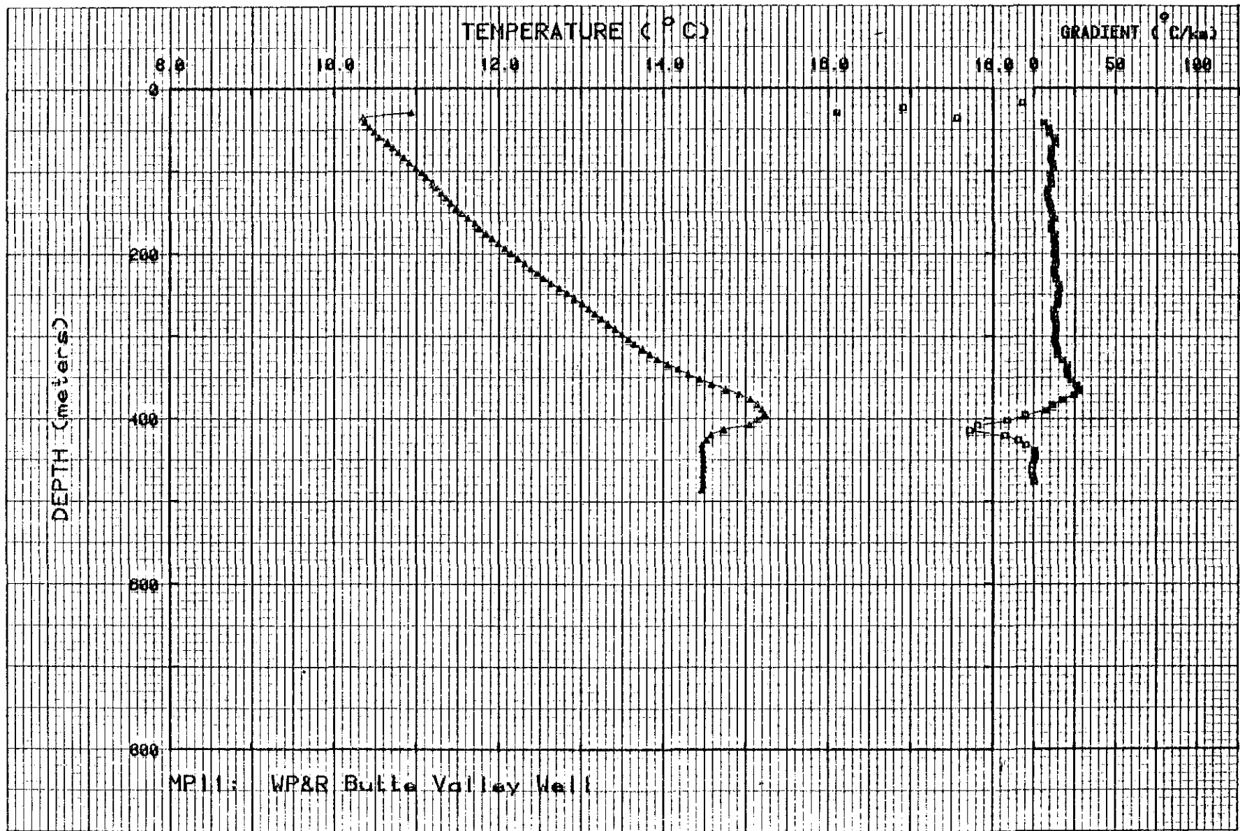
Figure II-11. Temperature and gradient profiles for MP11.
