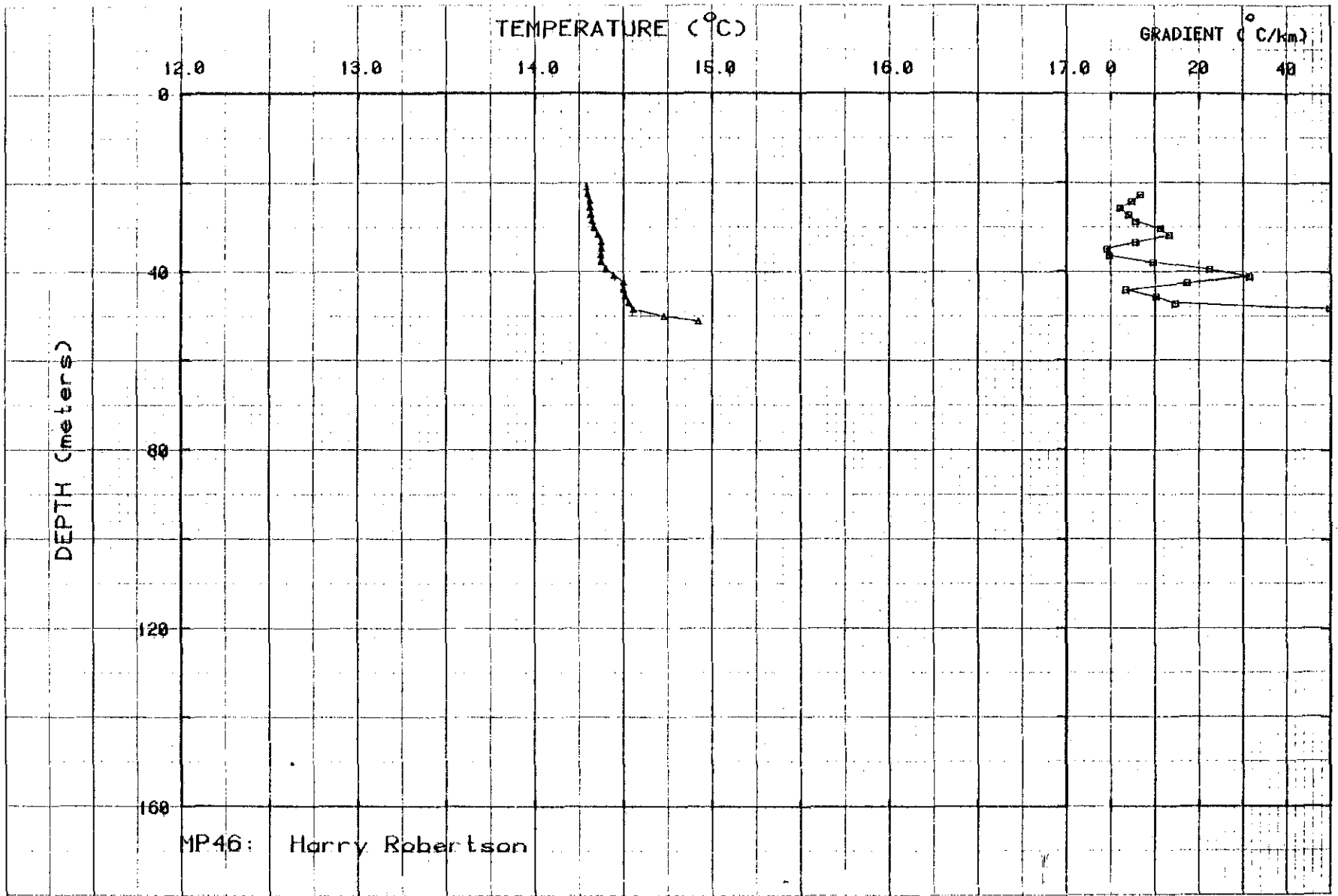
Figure II-45. Temperature and gradient profiles for MP46.
