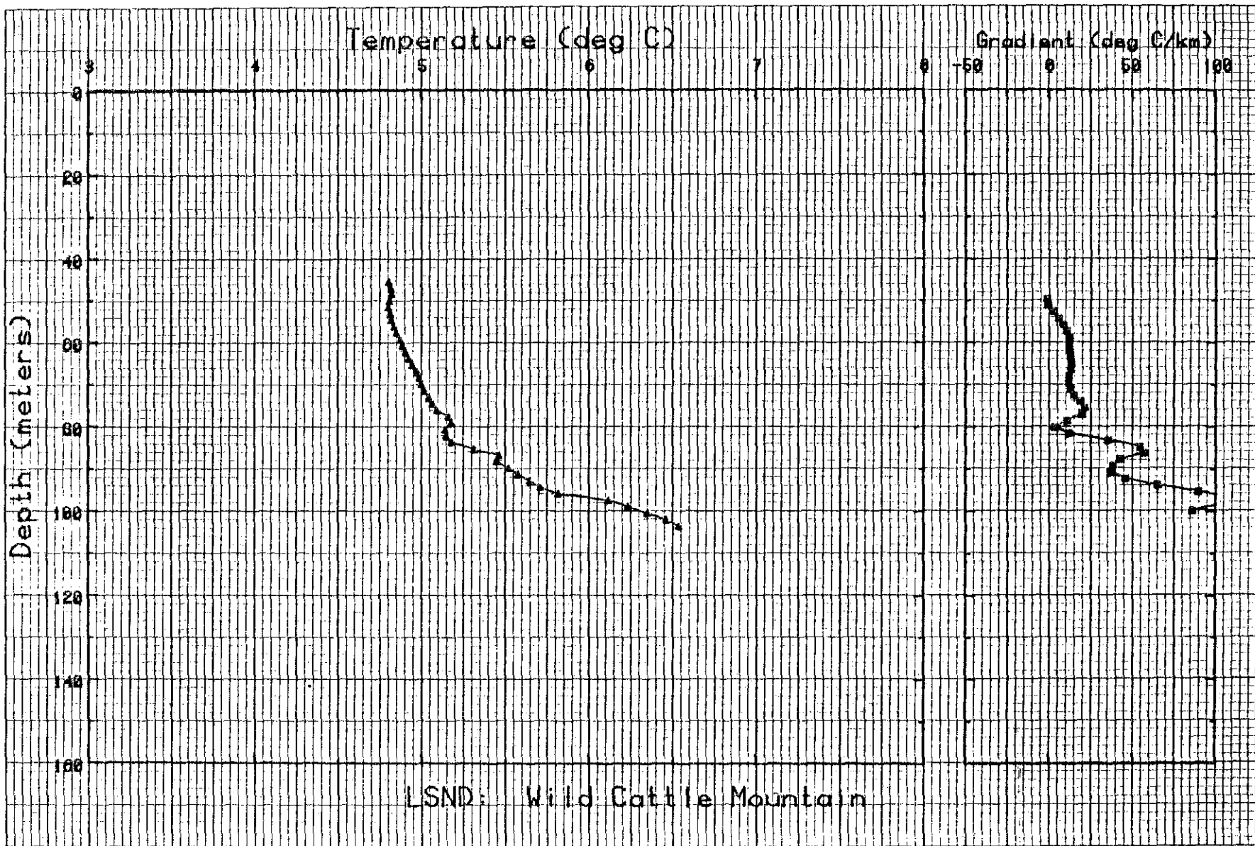
Figure I-8. Temperature and gradient profiles for LSND.
