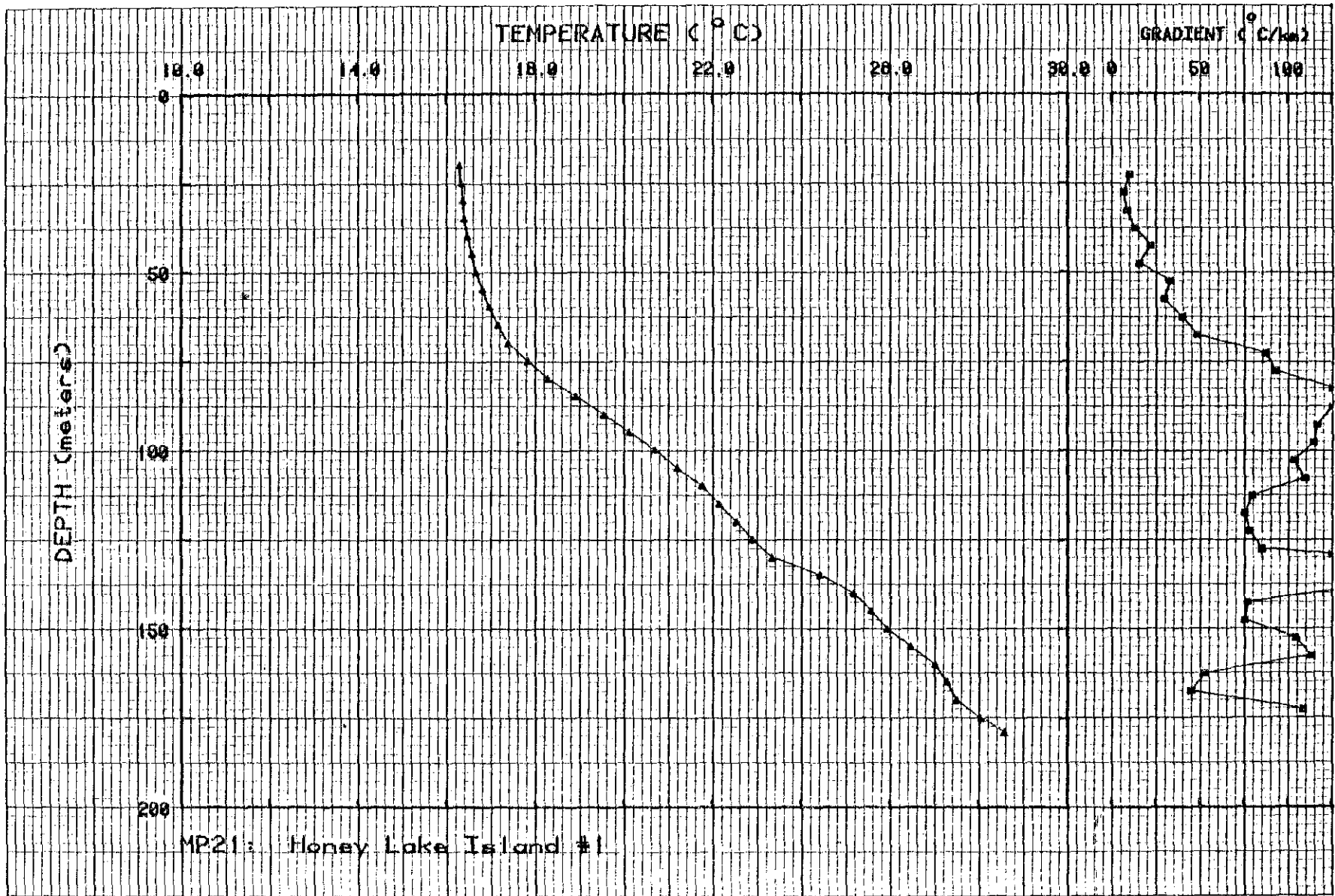
Figure II-21. Temperature and gradient profiles for MP21.
