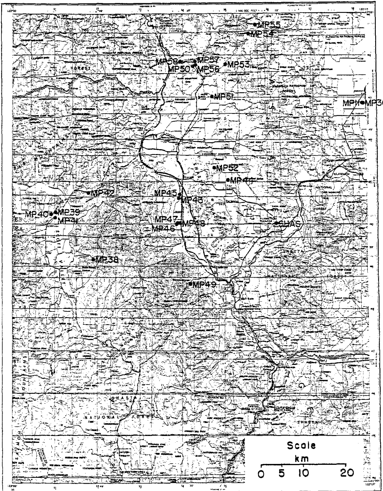
Figure IIc. Location map for the Mount Shasta region.
