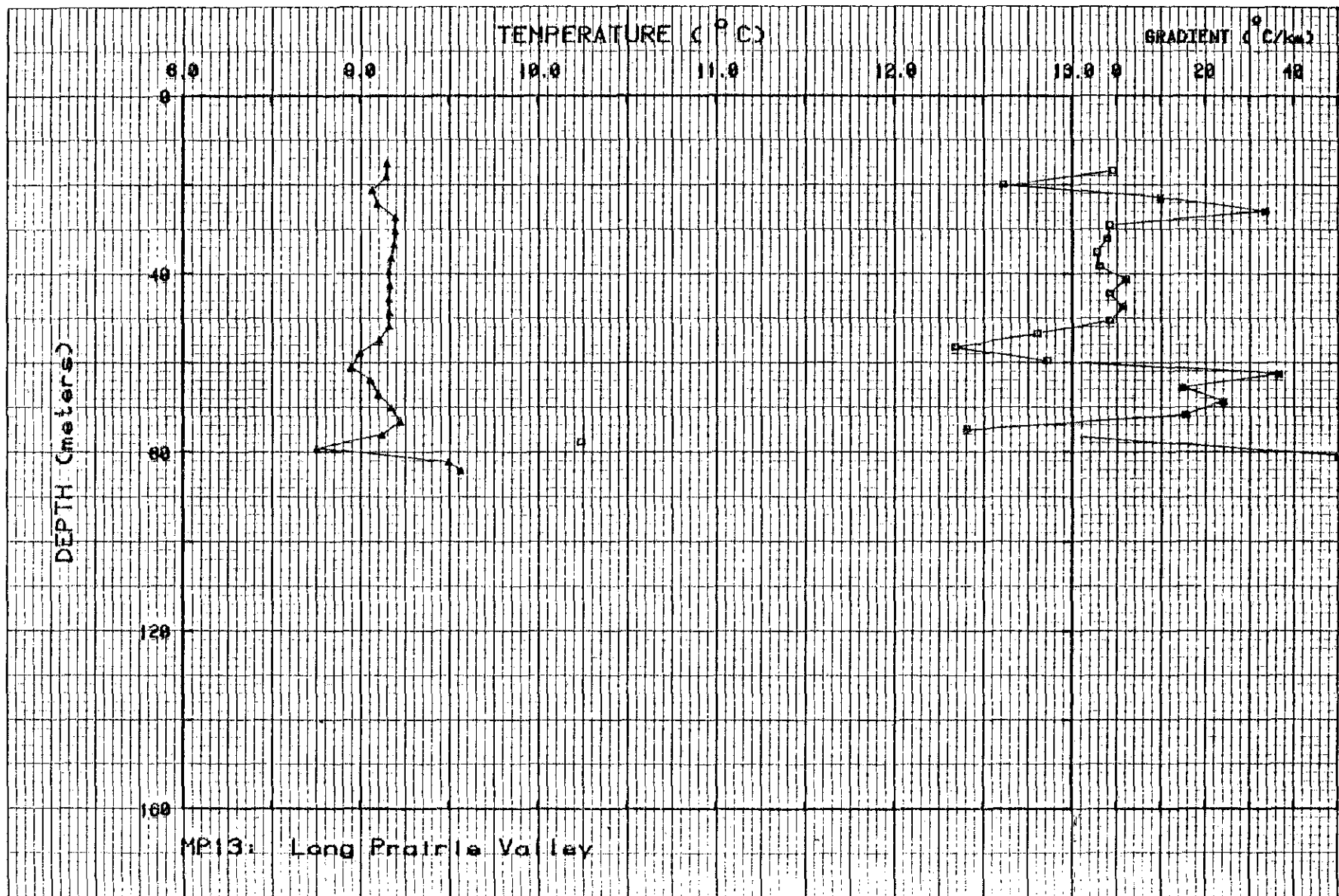
Figure II-13. Temperature and gradient profiles for MP13.
