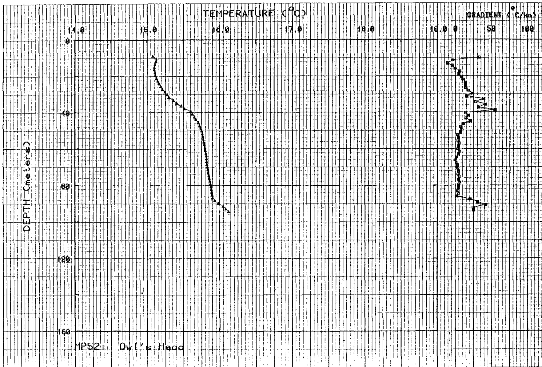
Figure II-51. Temperature and gradient profiles for MP52.
