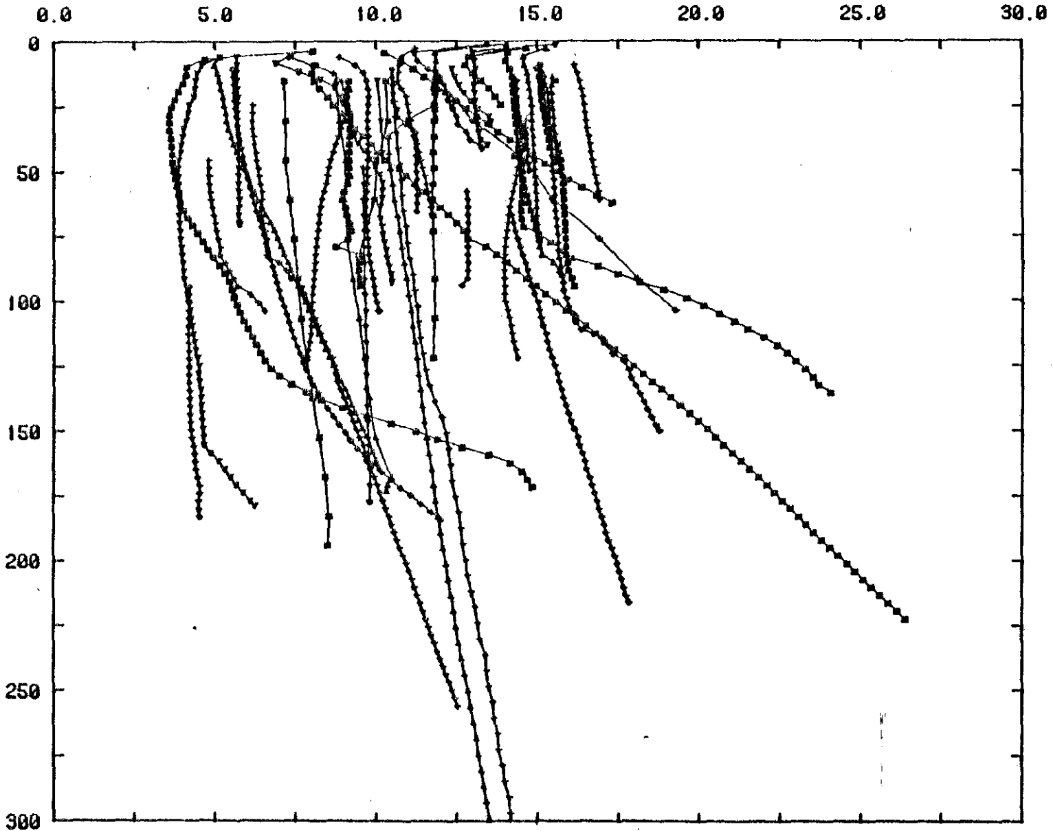
Figure 5. Temperature-depth profiles for the Cascades.
