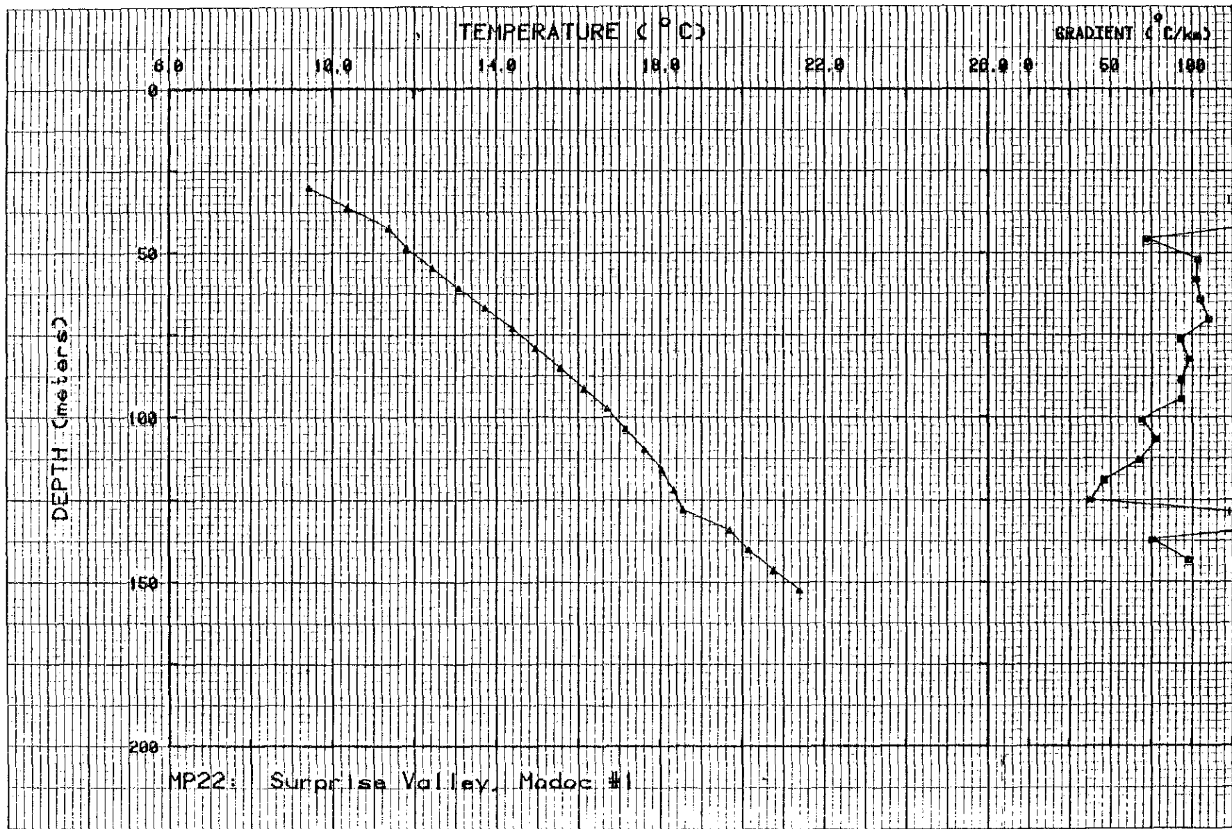
Figure II-22. Temperature and gradient profiles for MP22.
