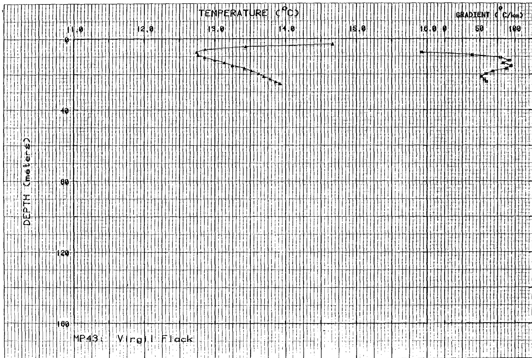
Figure II-42. Temperature and gradient profiles for MP43.
