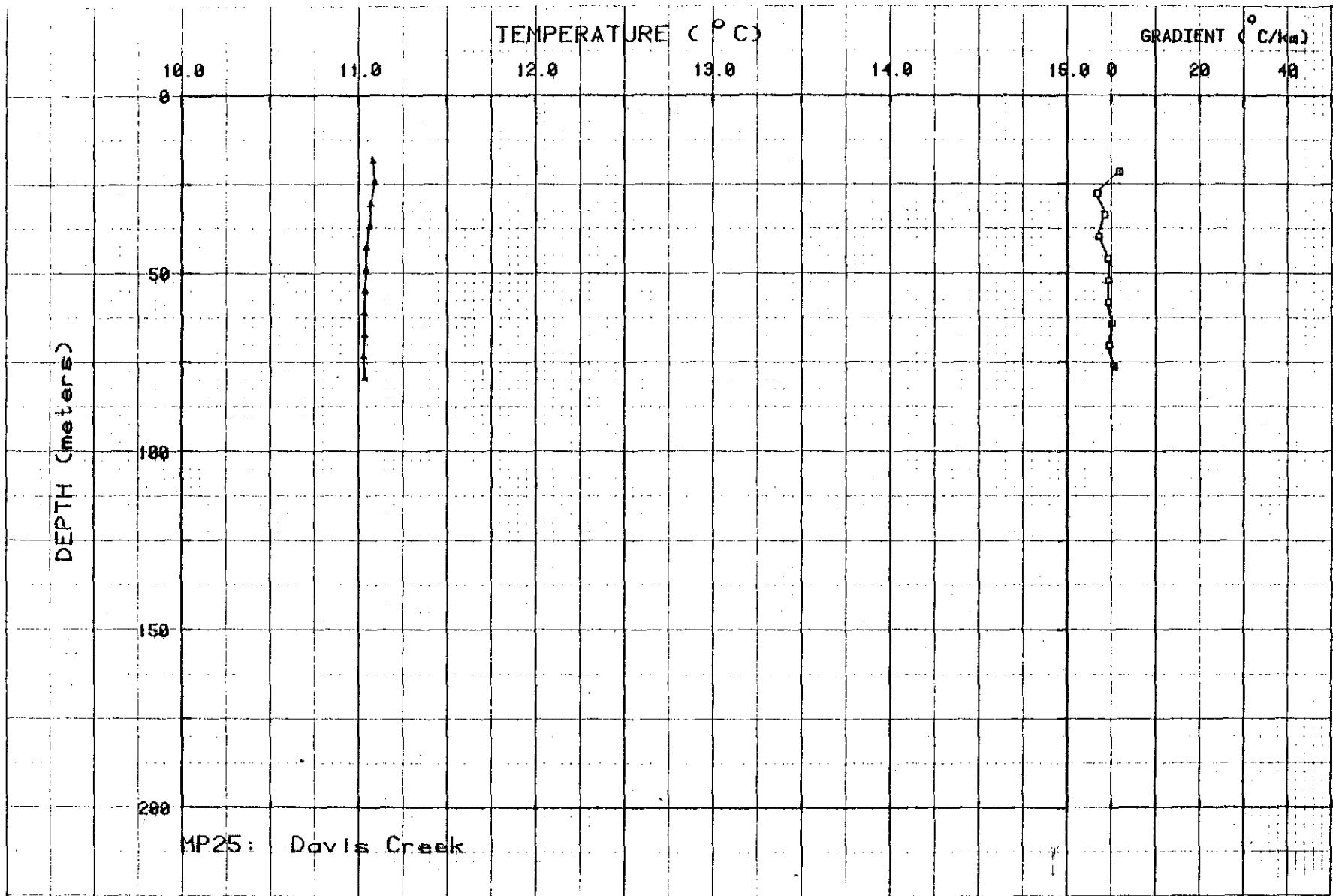
Figure II-25. Temperature and gradient profiles for MP25.
