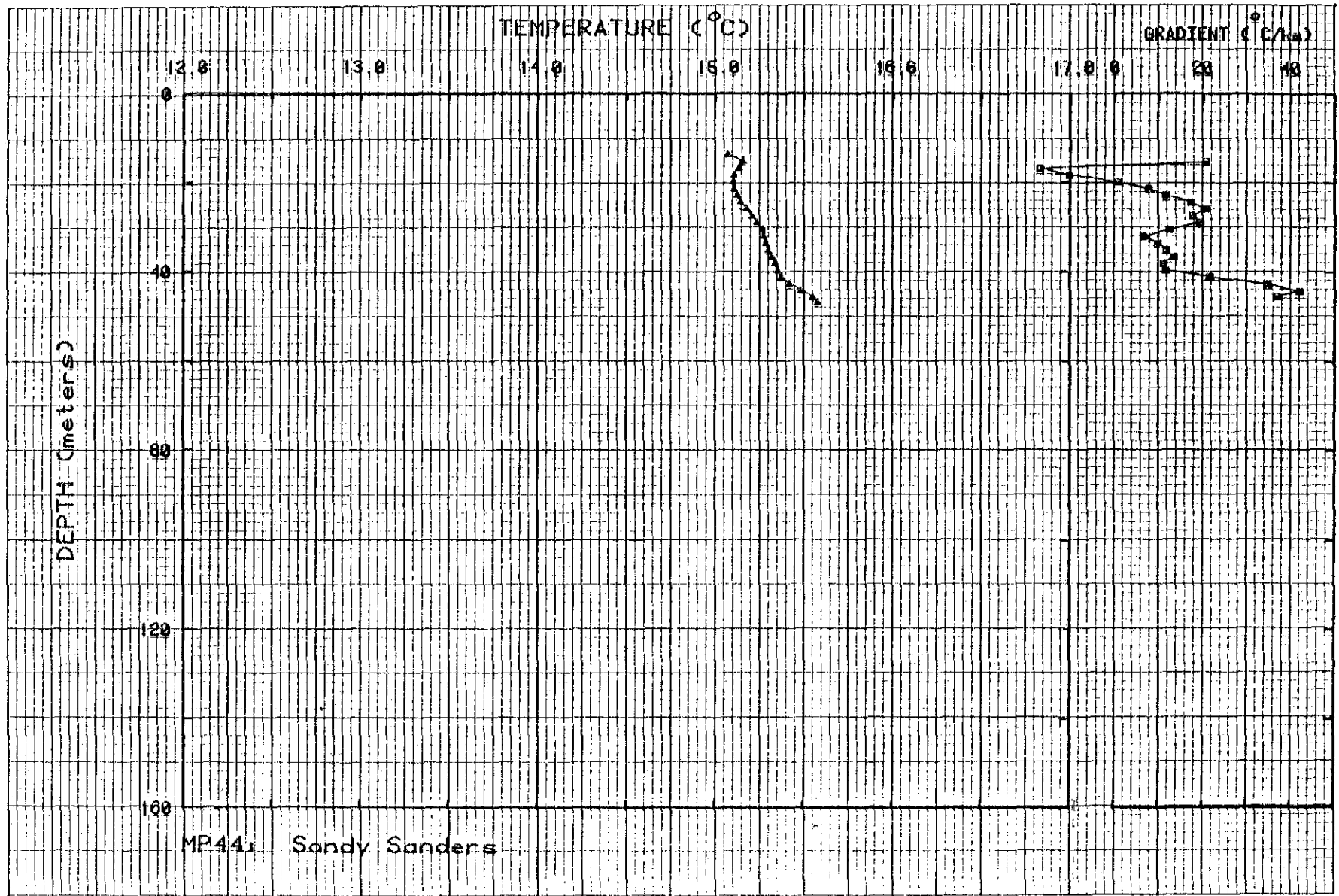
Figure II-43. Temperature and gradient profiles for MP44.
