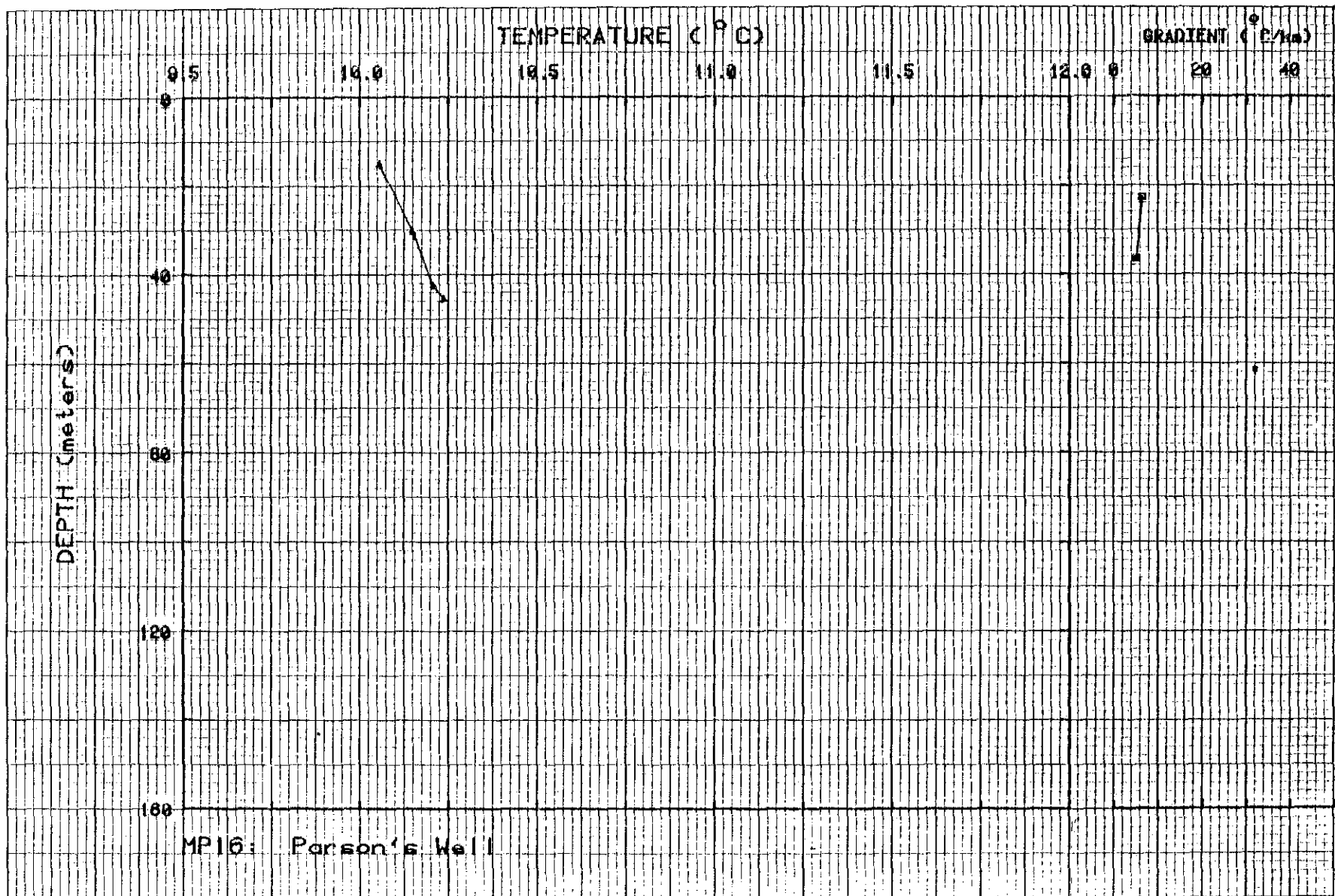
Figure II-16. Temperature and gradient profiles for MP16.
