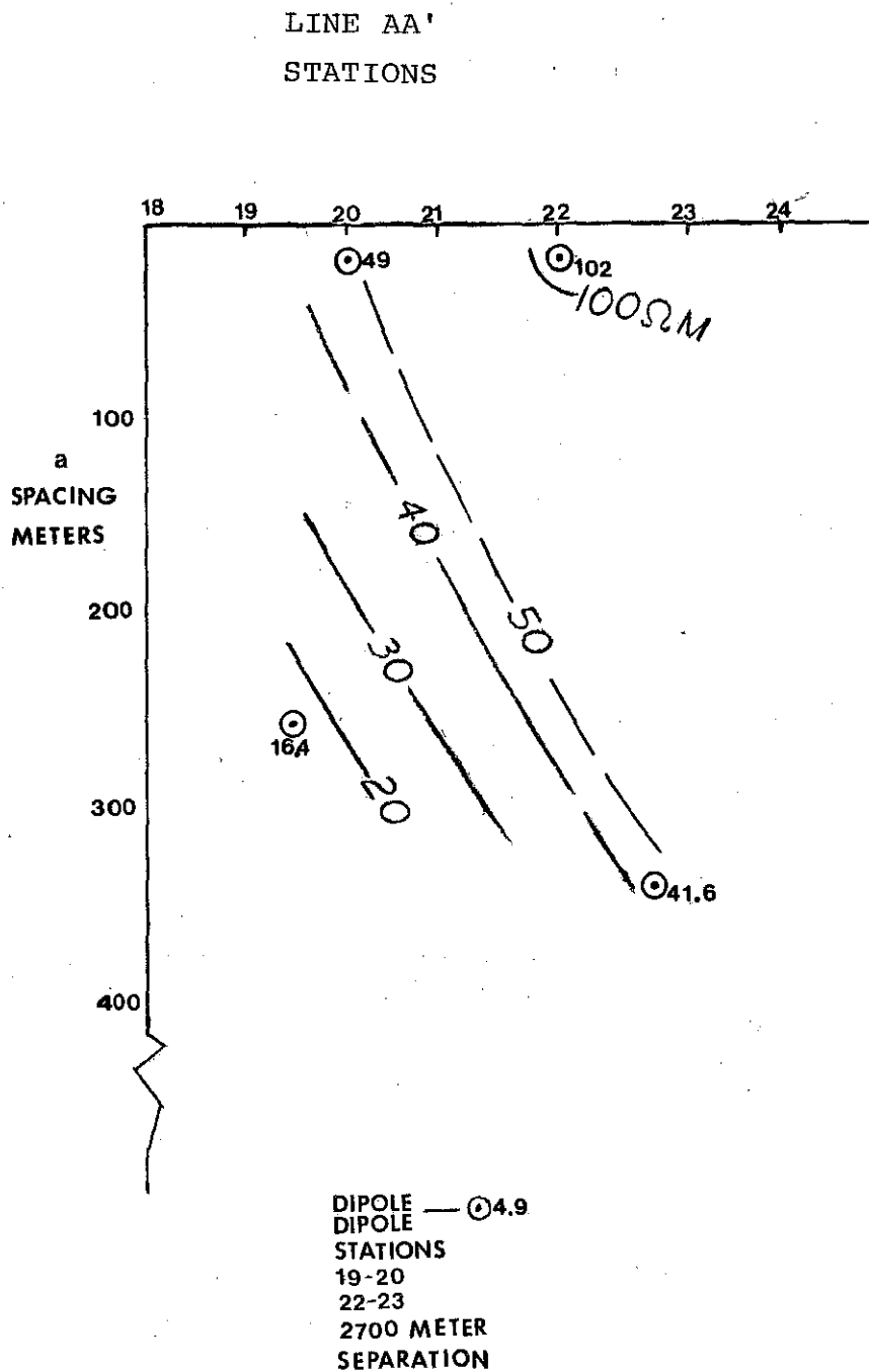
Figure 4. D.C. resistivity measurements were taken between stations 18 to 23, Wenner a spacings from 15 to 330 meters. One dipole-dipole measurement was made between stations 19-20 and 22-23.
