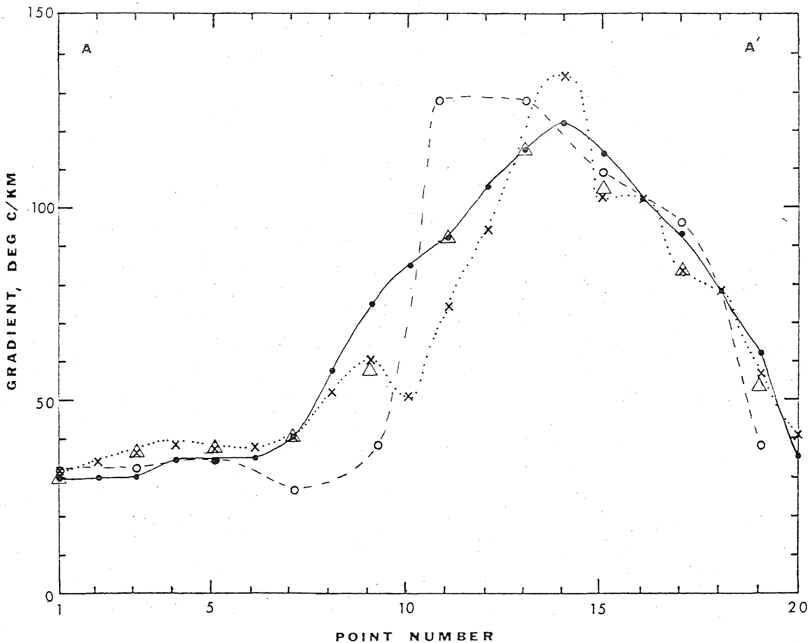
Figure 1b. Gradients for profile AA'. Dots are ideal (contoured) gradients, X's are input "terrain corrected" gradients, \Delta 's are gradients calculated at -70 m, and O's are gradients calculated at -1070 m.
