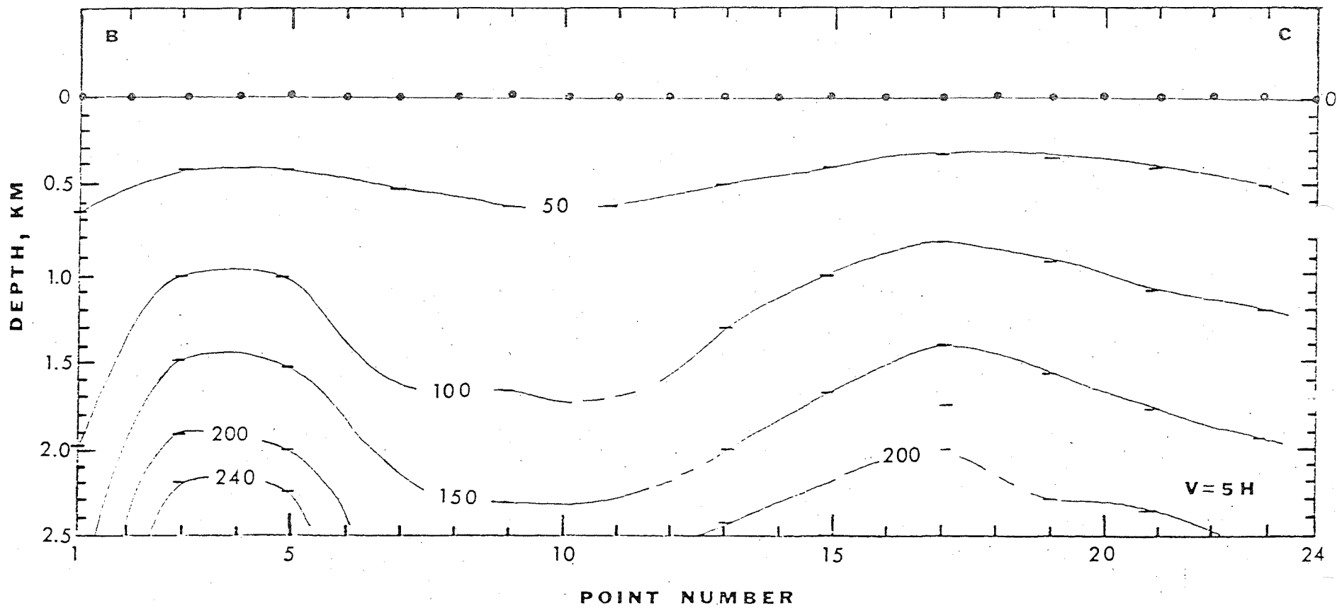
Figure 3a. Isothermal section for profile BC assuming a plane surface. Isotherms ( ^{\circ}\text{C} ) constructed using data from Table 6.
