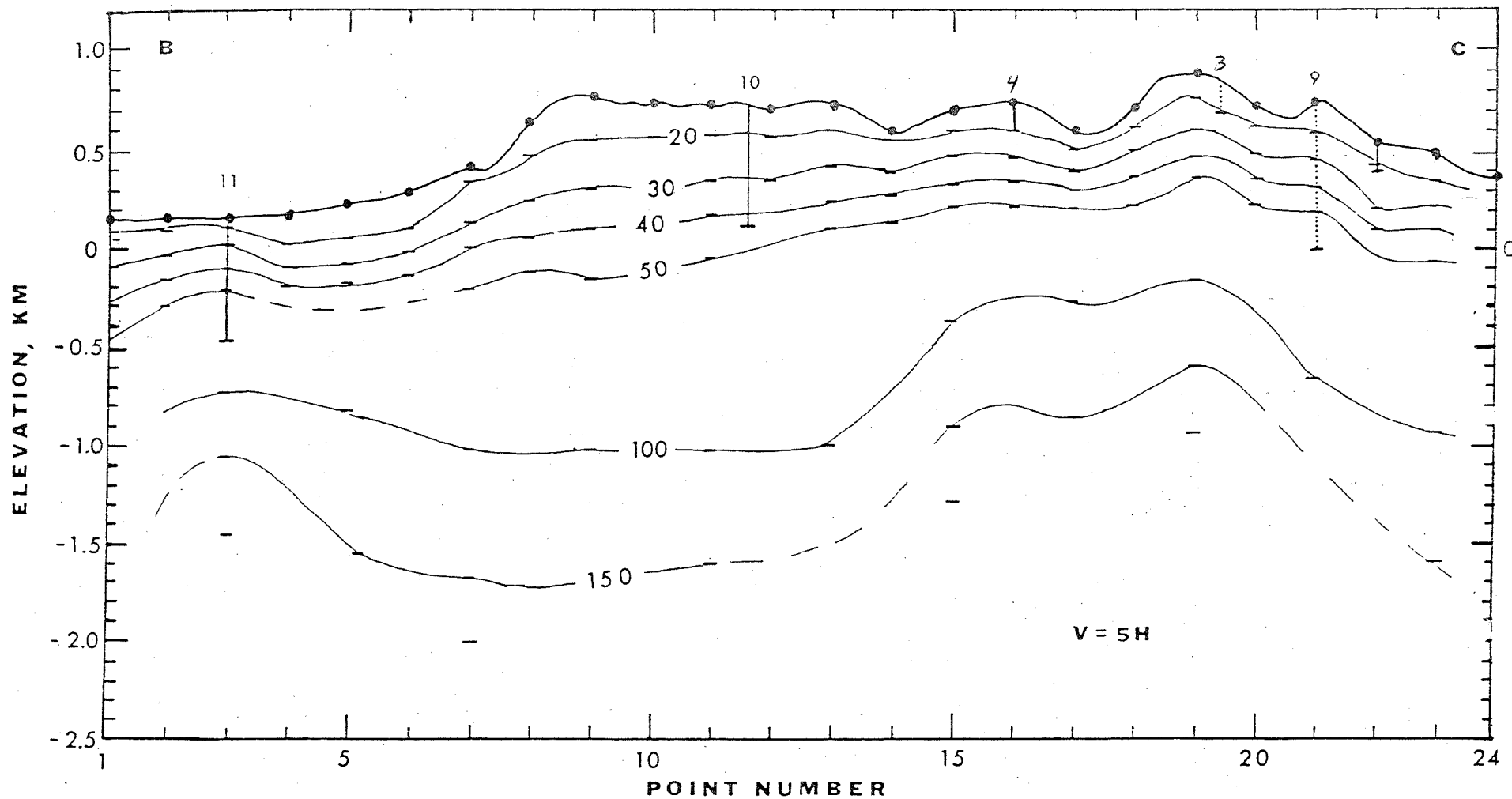
Figure 2a. Isothermal section and digitized topography (dots) for profile BC. Isotherms ( ^{\circ}\text{C} ) shown were constructed using data from Table 5 (horizontal bars). Hole locations shown.
