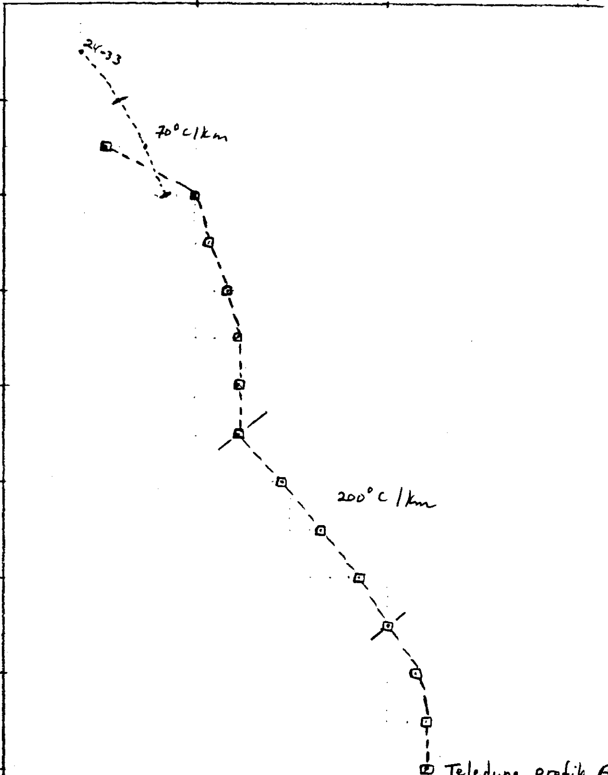
Figure 3. Depth temperature curve for well 24-33 and the depth temperature profile for line A-A' predicted by the Teledyne technique for well 24-33.
