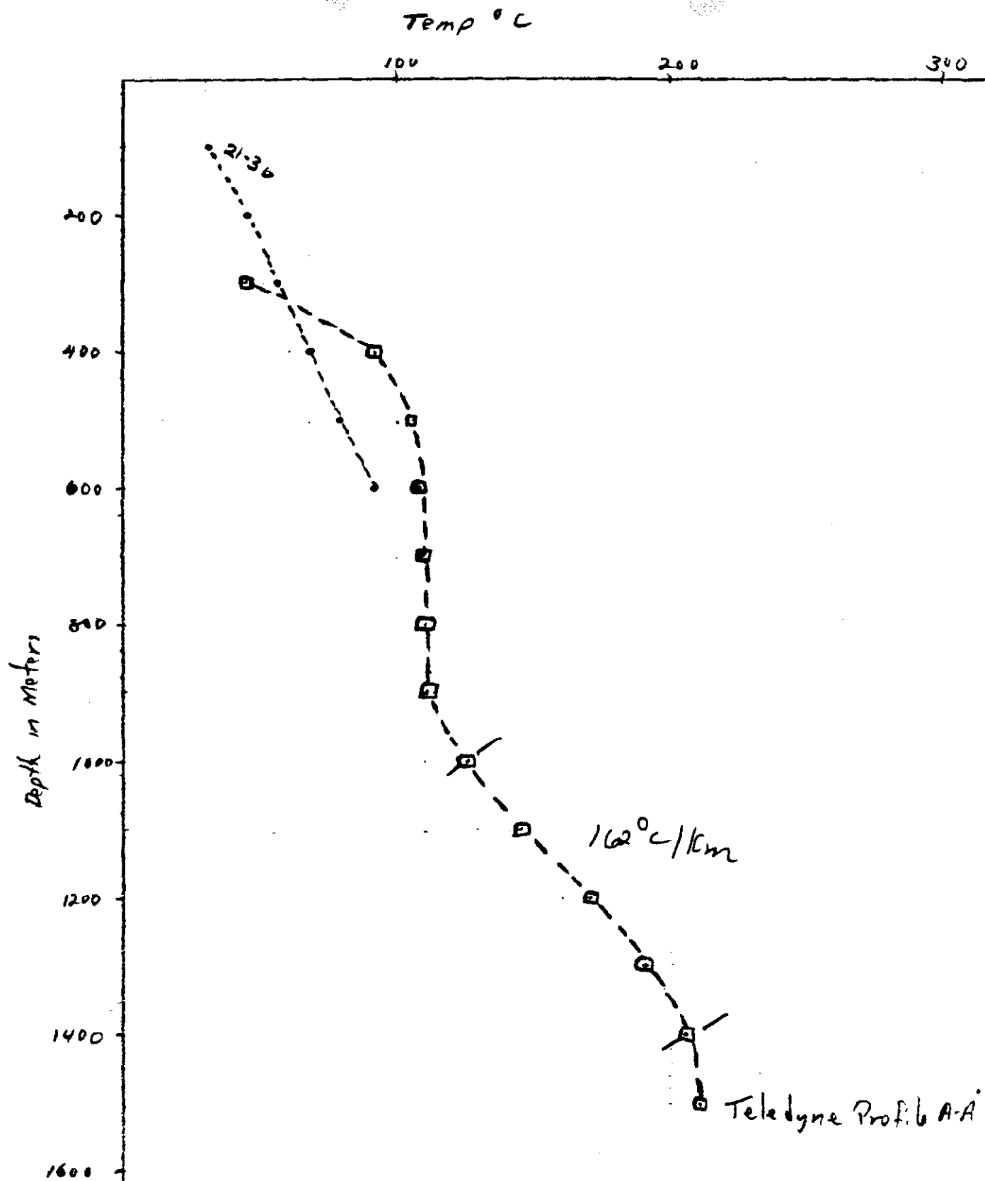
Figure 4. Depth-temperature curve for well 21-30 and the depth-temperature profile for line A-A' predicted by the Tele-dyne technique.
