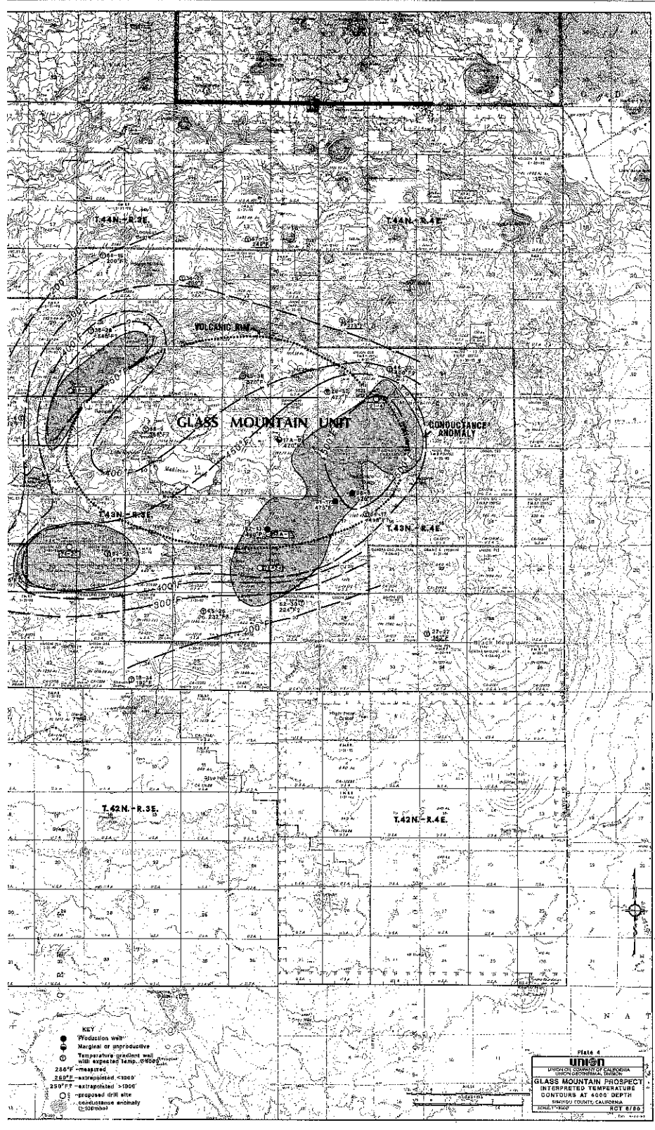
Interpreted Temp contours 4000 ft mapA.TIF
