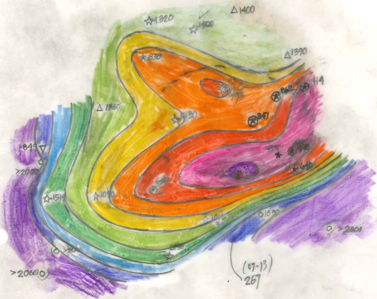
DEPTH TO 150°C ISOTHERM
