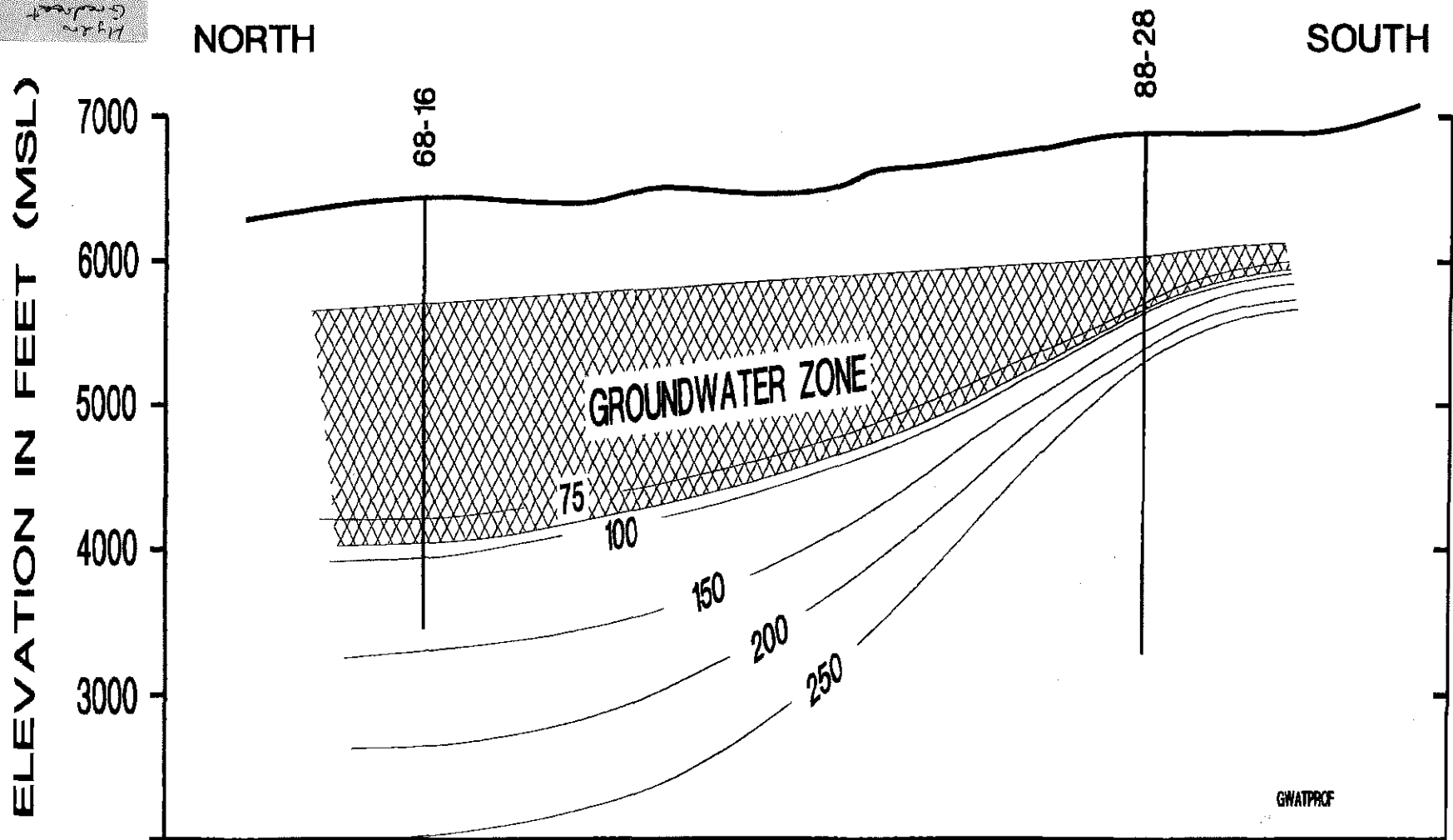
Figure 4. Cross section through gradient holes 68-16 and 88-28 showing subsurface temperature distribution and zone of groundwater saturation. Vertical exaggeration = 2X.
