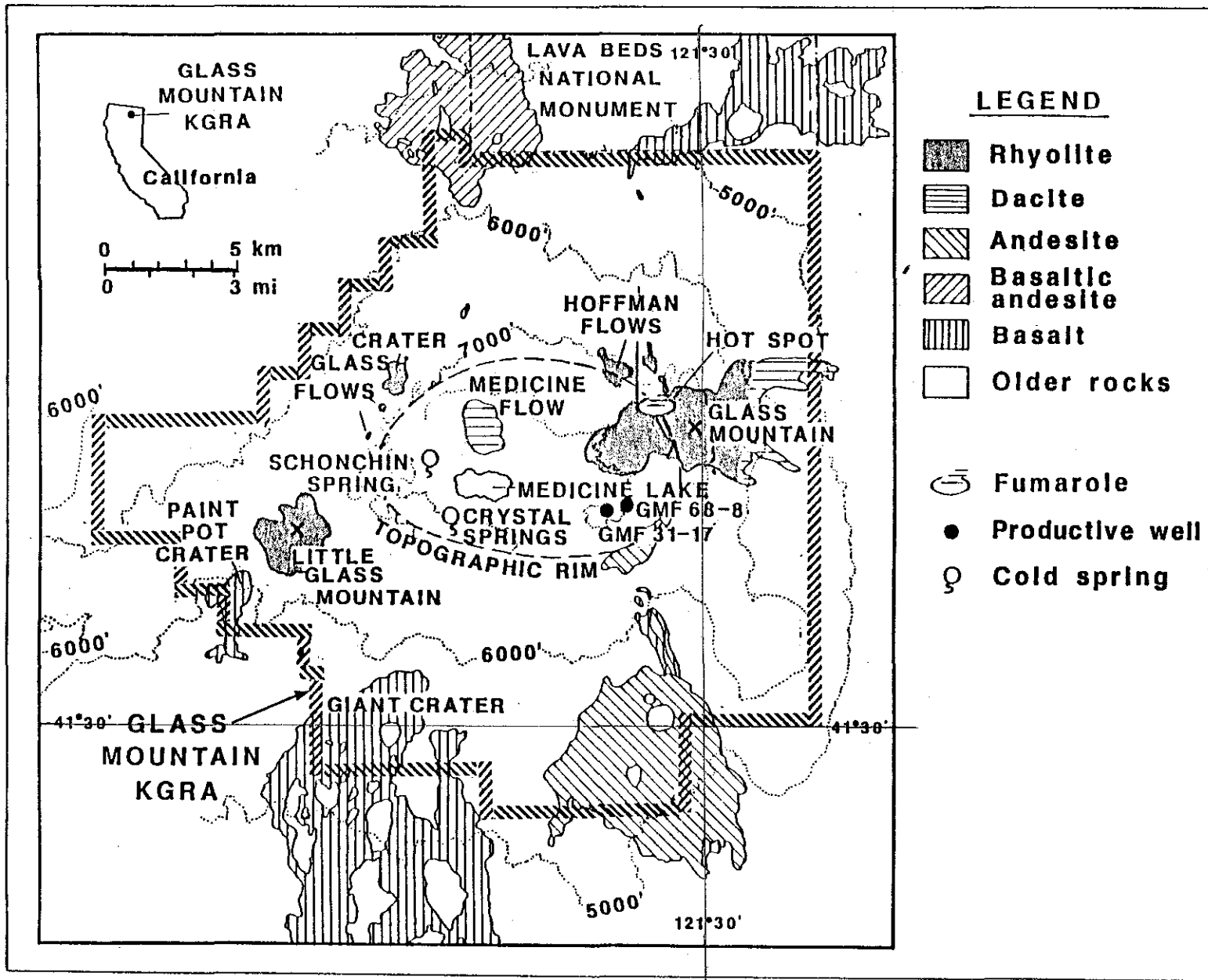
Figure 1: Geologic Map of Medicine Lake Volcano showing Holocene lavas (Donnelly-Nolan, 1988) and the Glass Mountain KGRA.
