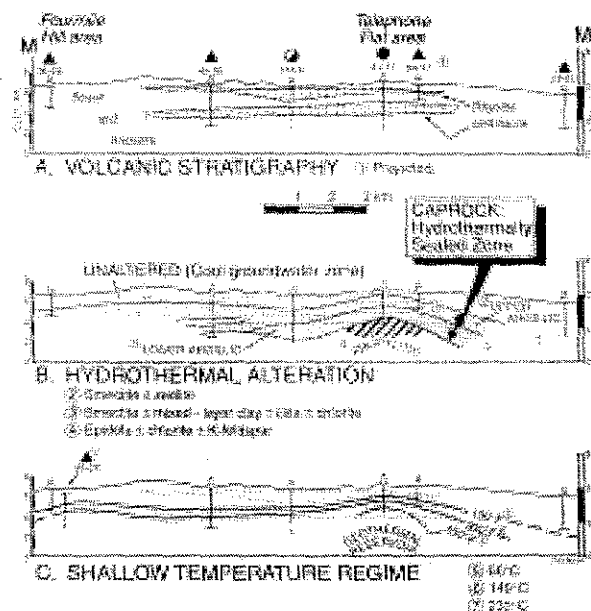
Fig. 2. Stratigraphic, alteration, and temperature cross-sections through upper portion of Medicine Lake volcano. A - Highly simplified Quaternary volcanic stratigraphy. The section is dominated by basalt, basaltic andesite, and andesite, but includes tongues of rhyolitic and dacitic flow, dome, and pyroclastic rock in the upper 1000 m of the wells. B - Generalized hydrothermal zoning in shallow portions of the boreholes. The key feature is a thick impermeable, argillic zone that inhibits the escape of hot waters from the underlying geothermal reservoir. C - Isothermal cross-section. The geothermal system intersected in well 31-17 reaches a temperature of about 275°C.
