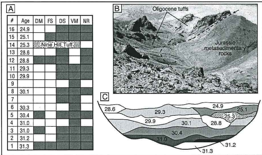
Figure 2. A: Shaded boxes indicate presence of tuff in paleovalley segment (see Fig. 3B for locations and abbreviation definitions); ages are in millions of years. B: Northern margin of paleovalley, Nightingale Range (looking west). C: Schematic paleovalley fill at Dogskin Mountain, with ages corresponding to individual tuffs.
