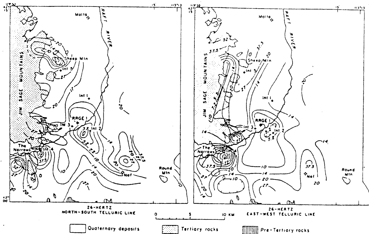
Figure 5. Audiomagnetotelluric apparent-resistivity maps of the southern Raft River valley. Resistivity contours shown are a logarithmic interval in ohm-meters.
