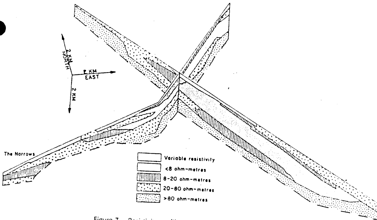
Figure 7. Resistivity profiles of the southern Raft River valley.
