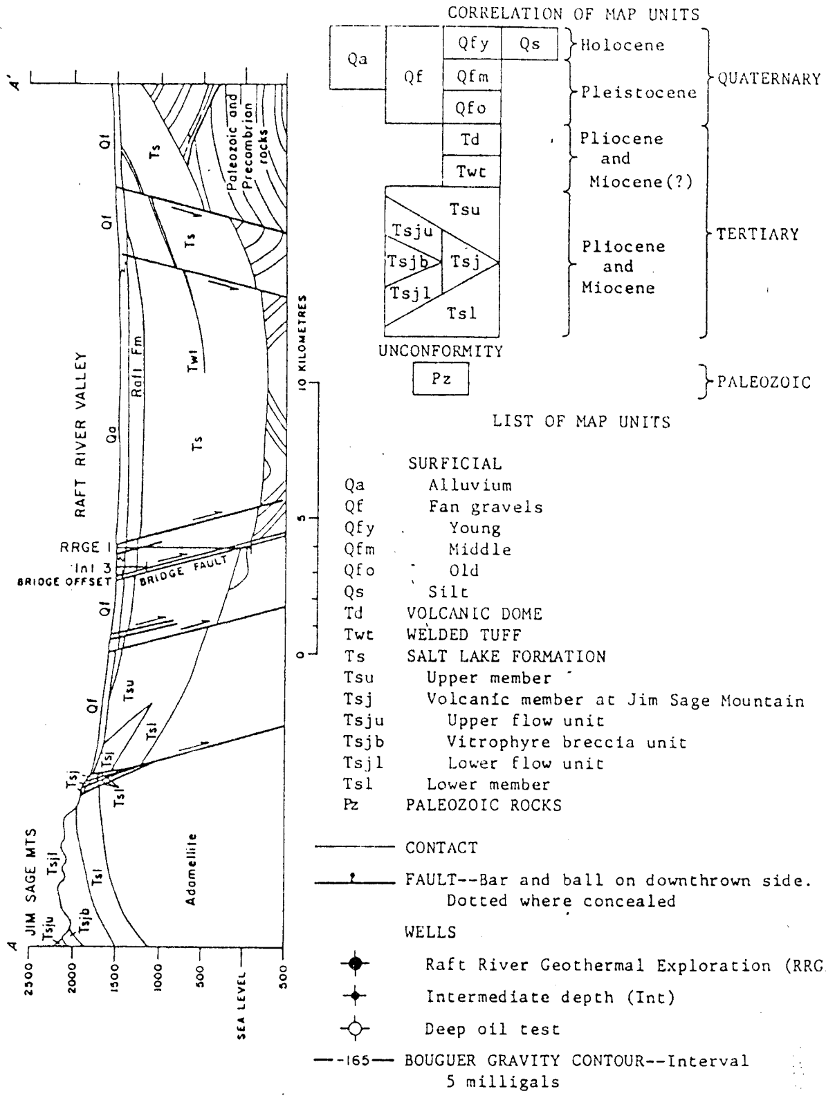
Contours, wells and geology. Right, cross section through AA' on the area map. Far right, correlation and list of geologic map symbols. Geology based on Williams et. al. (1974).
